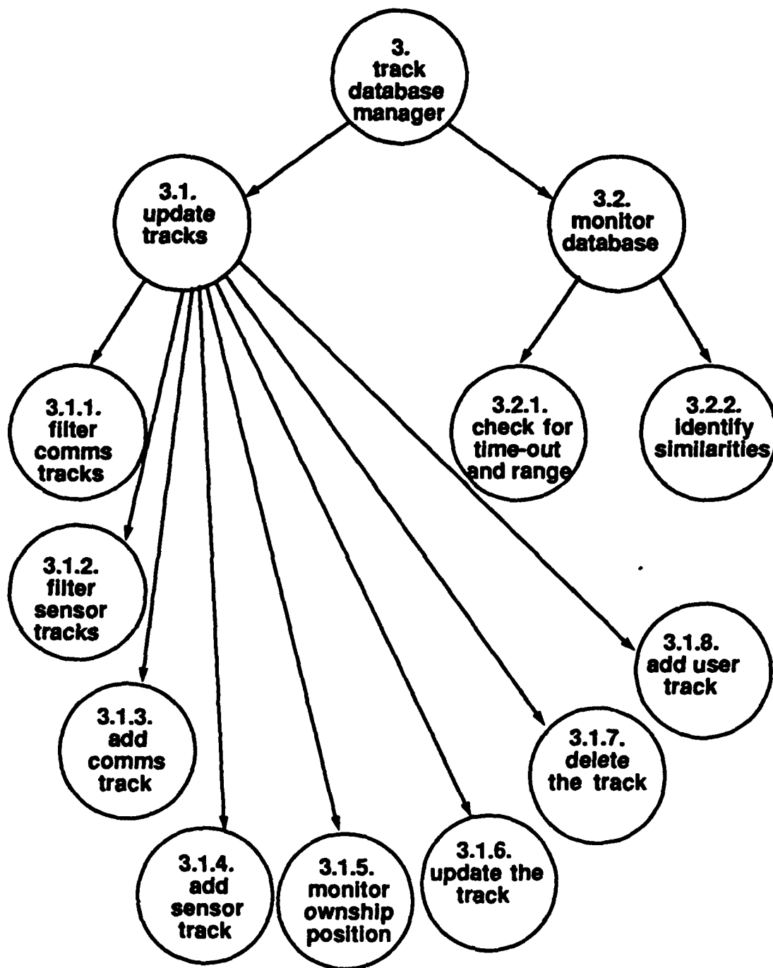
Figure 4-5. Decomposition of Track Database Manager Module
