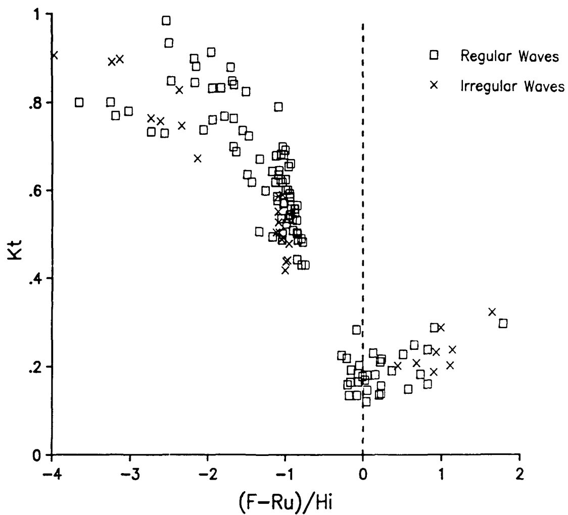
Figure 45. K_t versus (F-Ru)/H_i for irregular and regular waves
