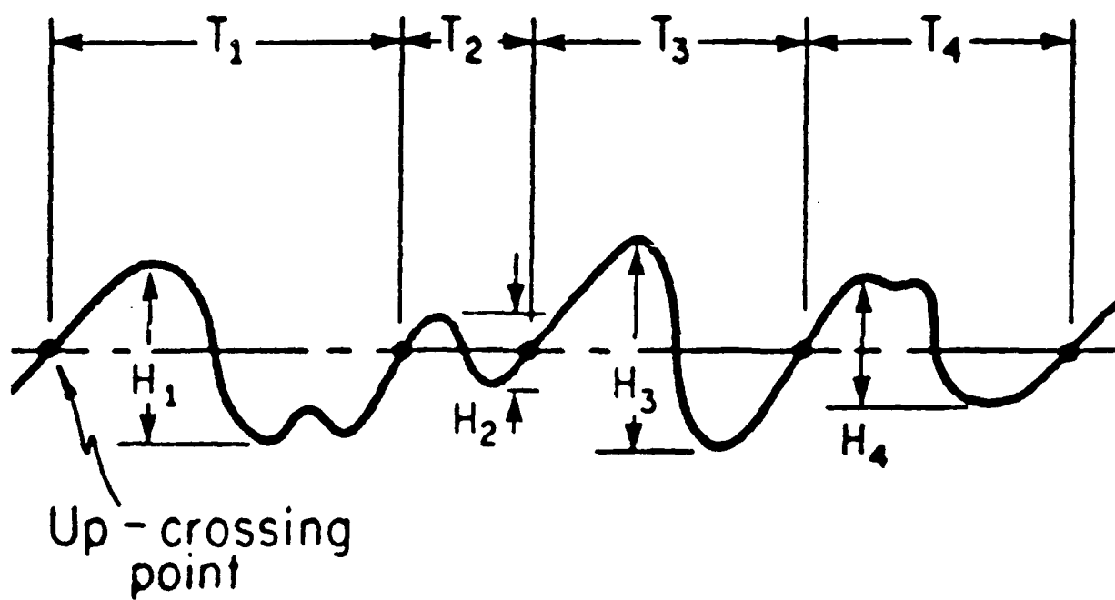
Figure 40. Zero-upcrossing method
