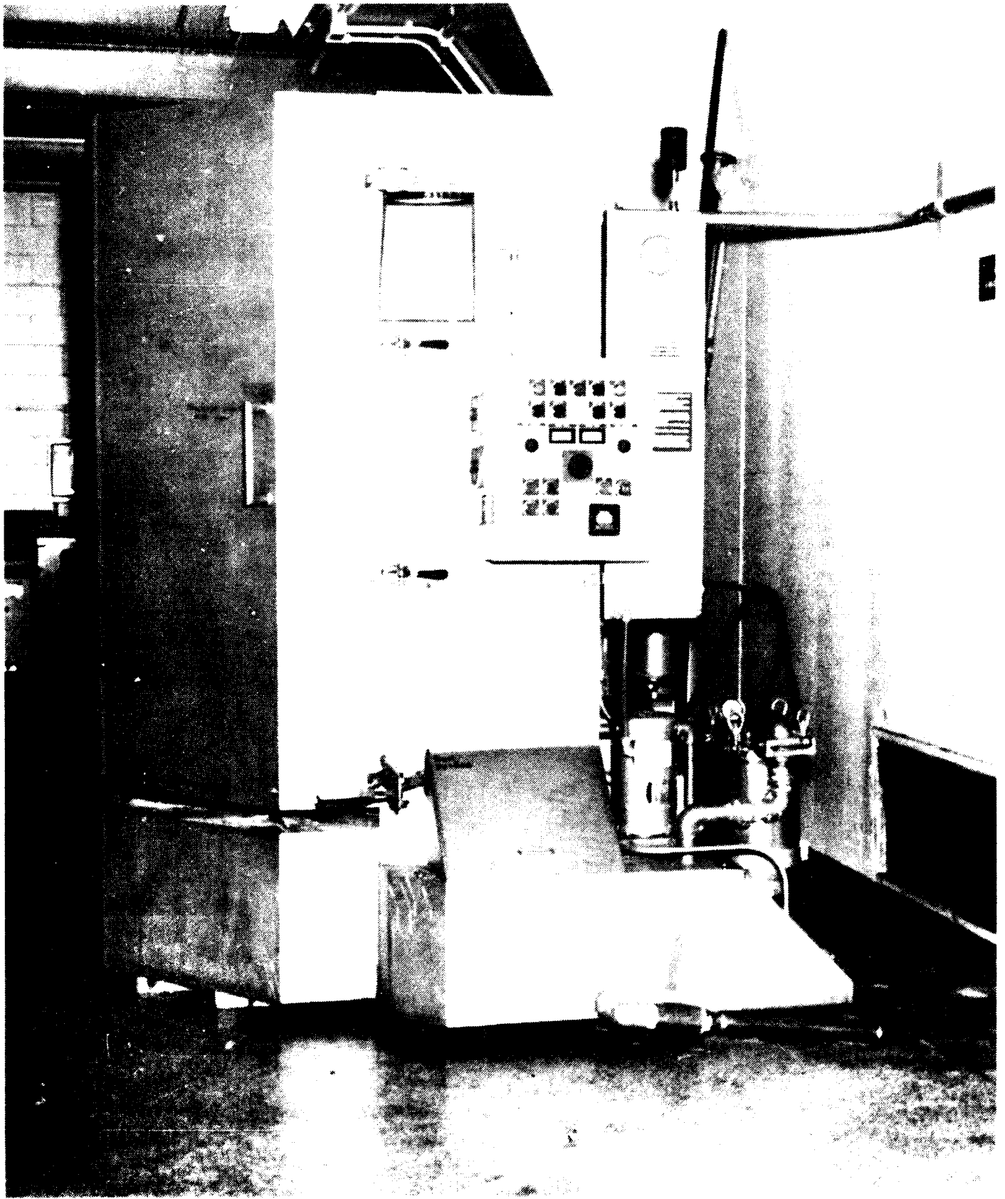
FIGURE 2 SIDE VIEW OF POWER SPRAY WASHER 5
