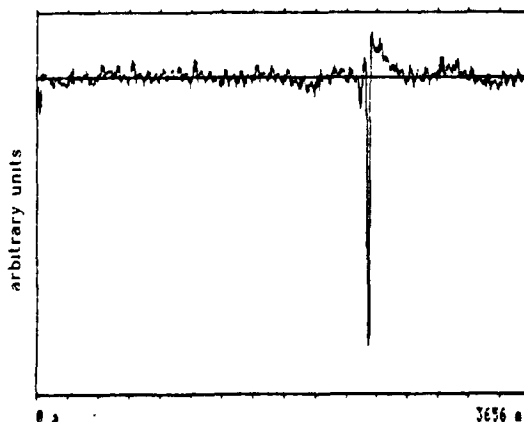
Fig. 4.3 Ranging at battle tank.
