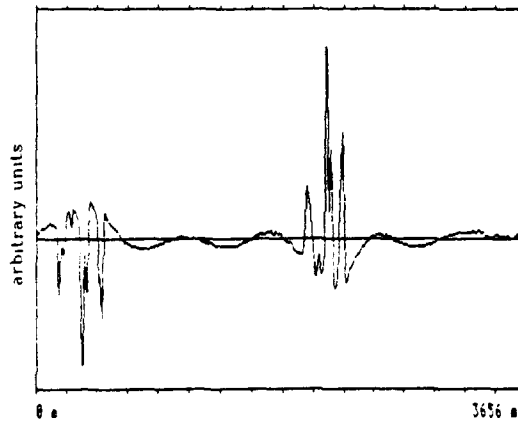
Fig. 4.8 Several clouds forming multiple targets, measurement in double (up/down) chirp mode.
