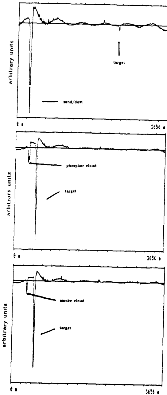
Fig. 4.7 a. object behind sand/dust cloud b. object behind white phosphorous cloud c. object behind fire smoke cloud
