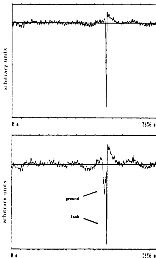
Fig. 4.5 a. Transmitter beam aimed on vehicle, b. Transmitter aimed partly on vehicle.
