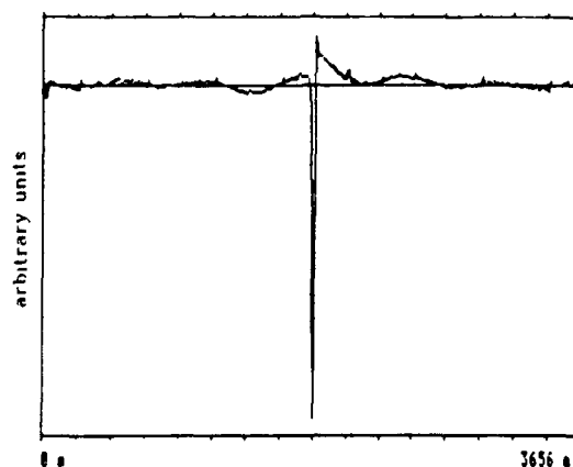
Fig. 5.1 Measurement output on VIDIS system, showing singular target reflection with side lobes and noise.
