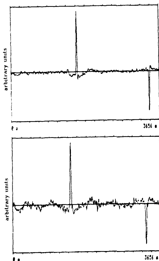
Fig. 4.10 a. double chirp measurement on target vehicle, b. idem, on ground in front of vehicle.
