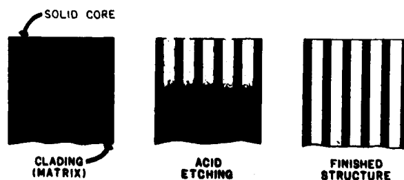
Figure 38. Etched Fiber Optics
