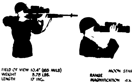
Figure 22. First Generation Small Starlight Scope
