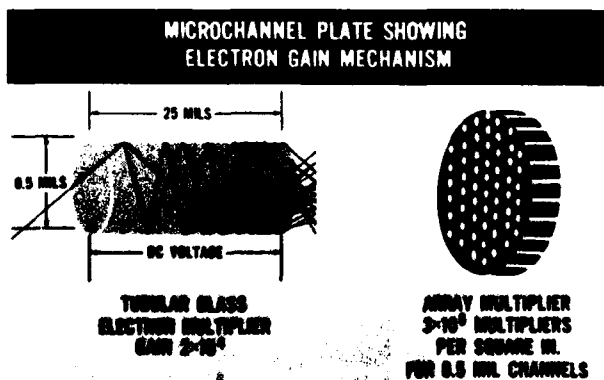
Figure 37. Microchannel Plate
