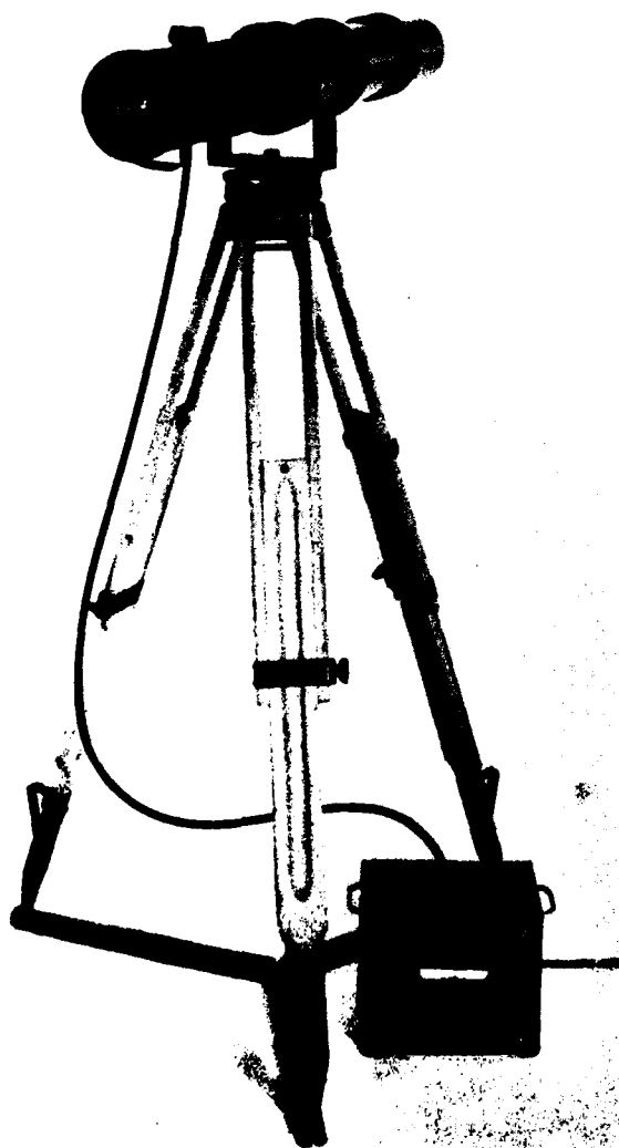
Figure 8. Three-Stage Viewer
