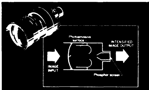
Figure 9. Demag- nification Tube
