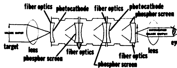
Figure 11. Three-Stage Cascade Tube with Fiber Optics Coupling
