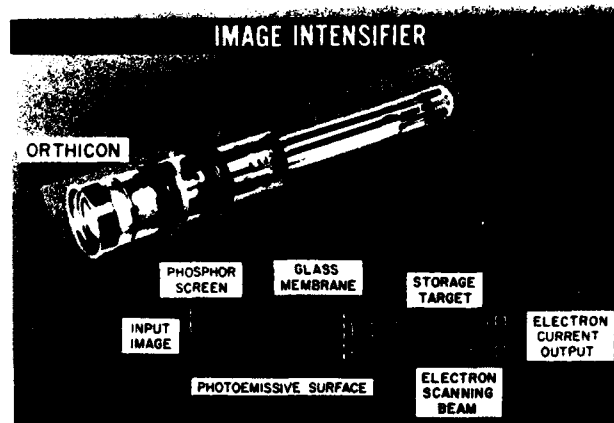
Figure 6. Image Intensifier Orthicon
