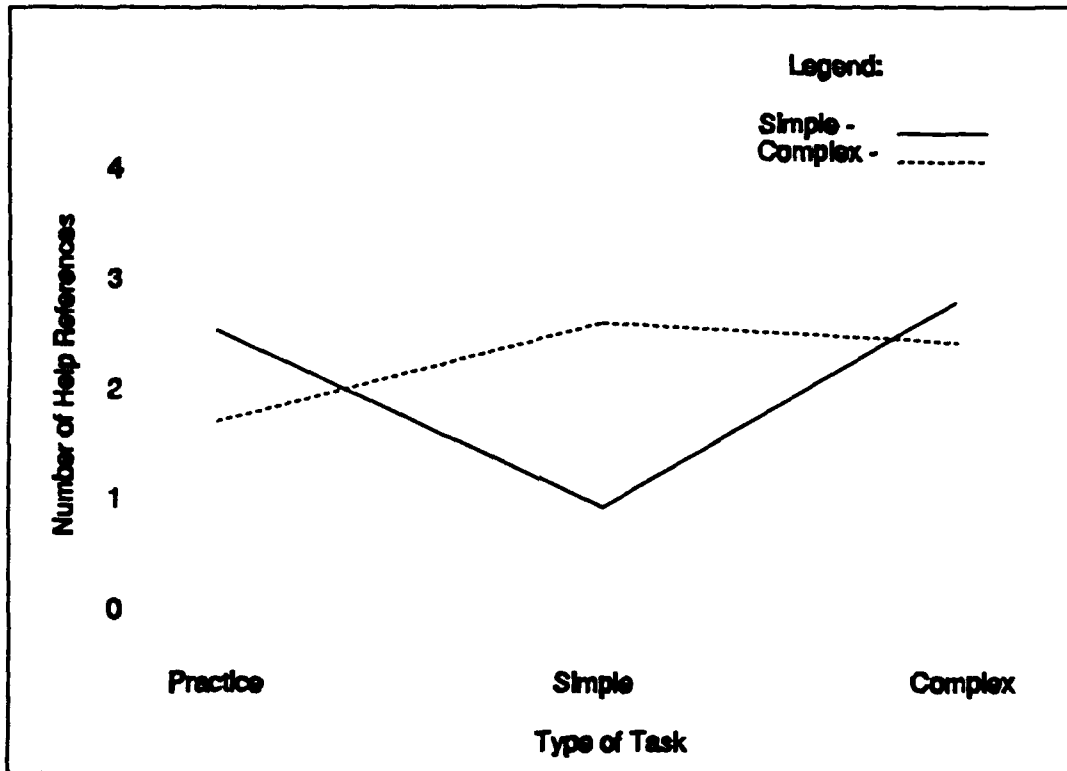
Figure 28 Mean Value of Number of Help References, as a Function of Interface Type and Task Type
