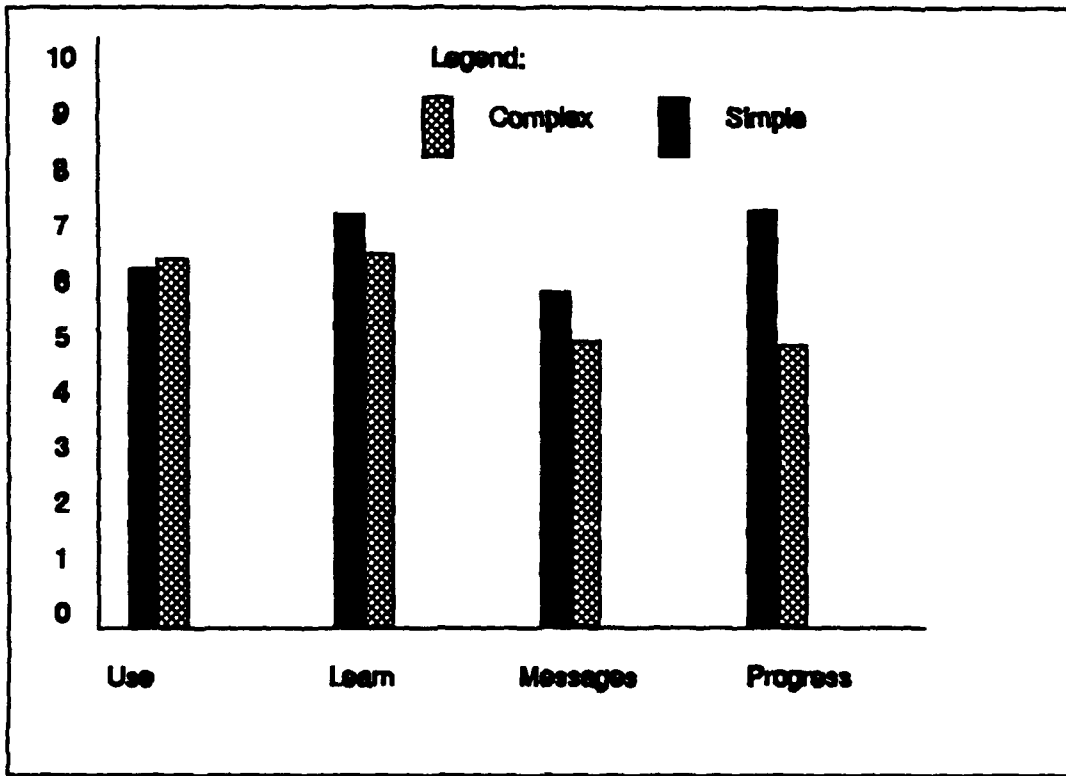
Figure 29 User Ratings of the Simple and Complex Interfaces for Four Variables
