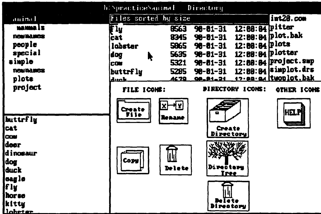
Figure 2 Simple Interface Opening Screen
