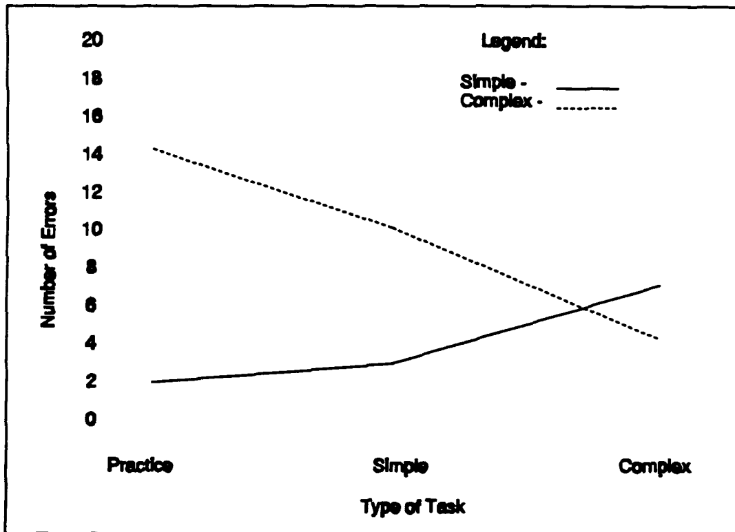
Figure 27 Mean Values for Number of Errors, as a Function of Interface Type and Task Type
