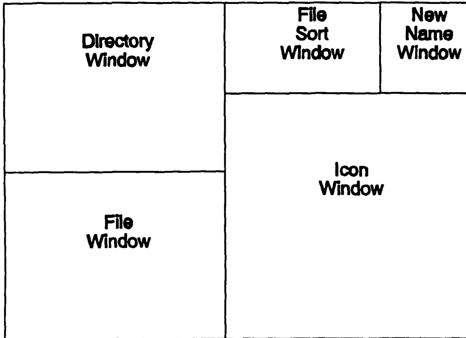
Figure 3 The Direct Manipulation Interface (DMI) Top Pane and Component Windows
