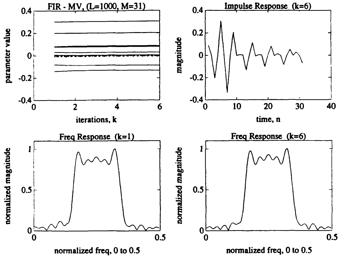
Figure A.2: 31 st Order FIR Model Using the V-cycle Method. Impulse and normalized frequency responses shown using L=1000 data points.
