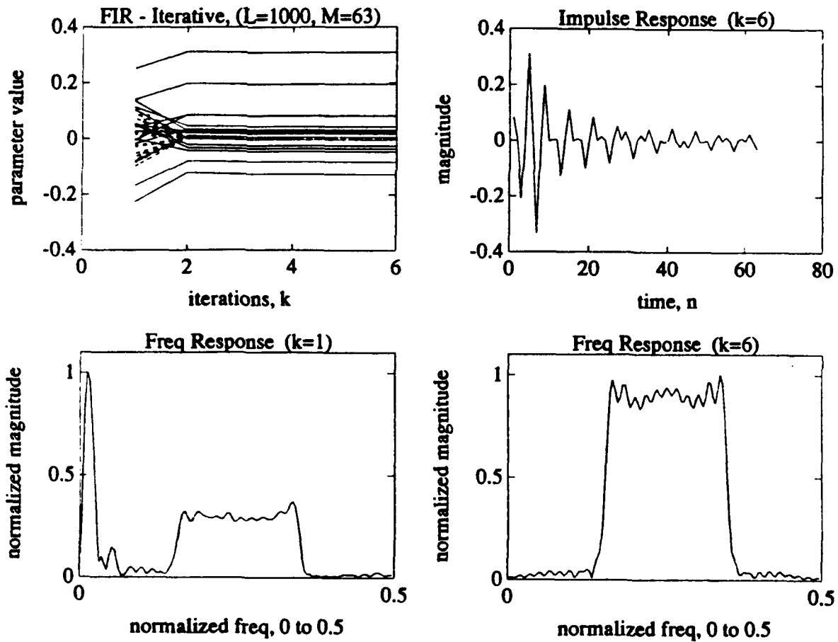
Figure A.5: 63 rd Order FIR Model Using the Straight Iterative Method. Impulse and normalized frequency responses shown using L=1000 data points.
