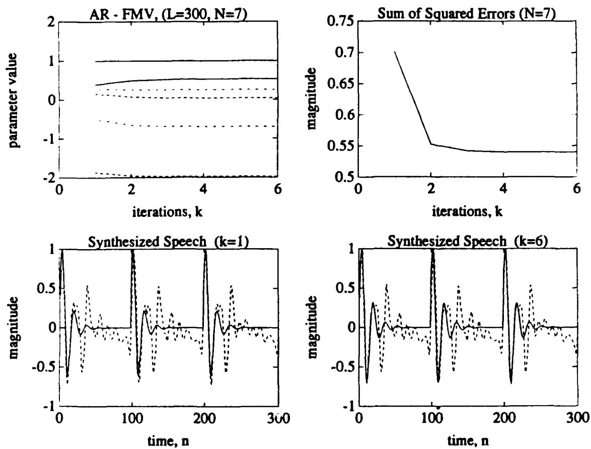
Figure B.6: 7 th Order AR Model of Voiced Speech Using the FMV-cycle Method. Original speech waveform shown in dashed lines, synthesized speech waveform shown in solid lines.
