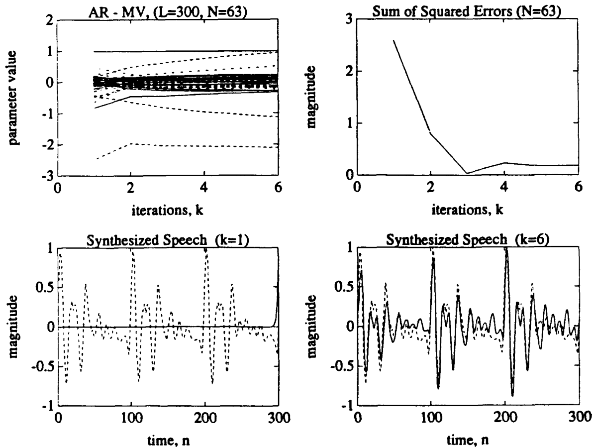
Figure B.11: 63 rd Order AR Model of Voiced Speech Using the V-cycle Method. Original speech waveform shown in dashed lines, synthesized speech waveform shown in solid lines.
