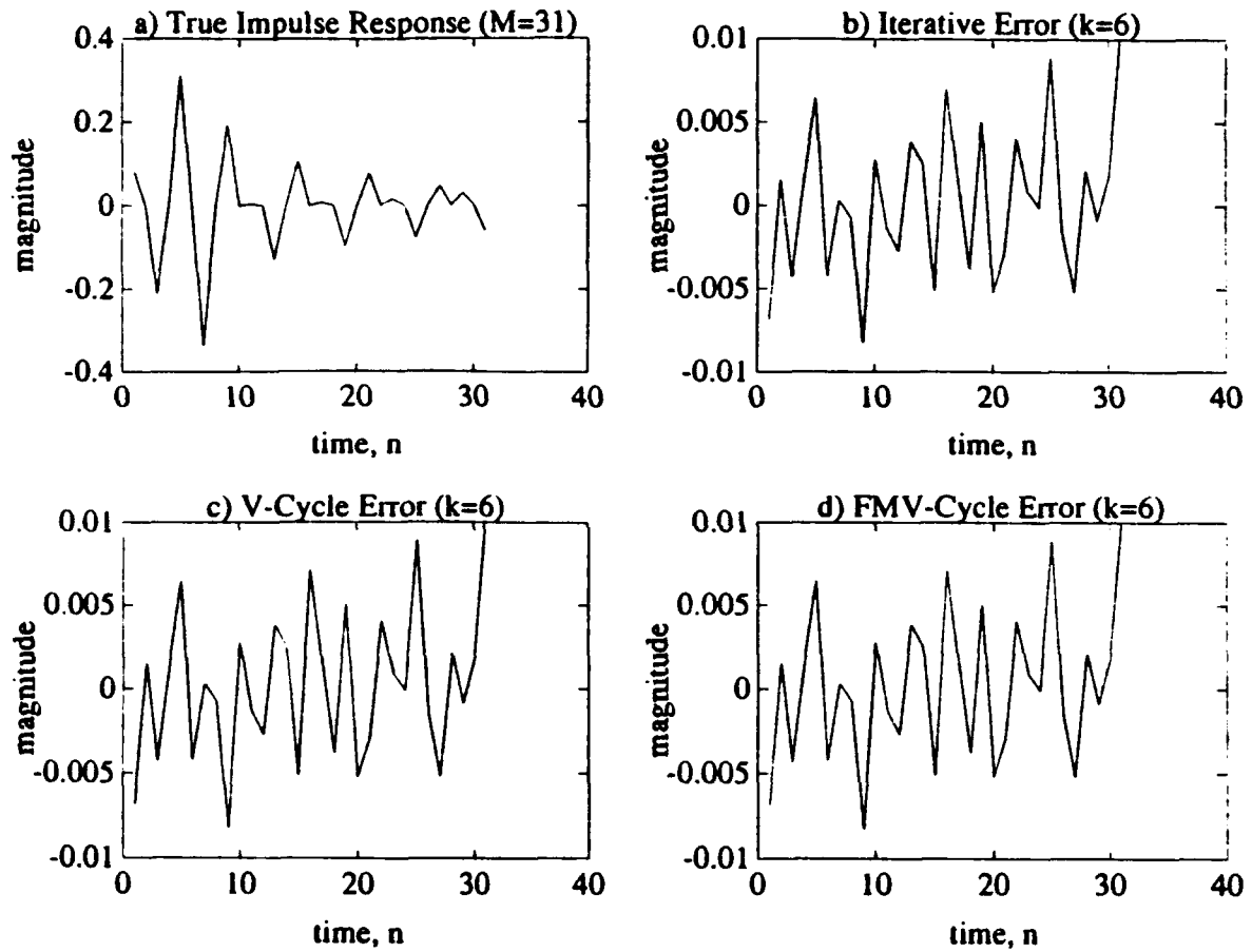
Figure A.4: 31 st Order FIR Model Impulse Response Comparison. a) True System Impulse Response; b) Iterative Method Error; c) V-cycle Method Error; d) FMV-cycle Method Error.
