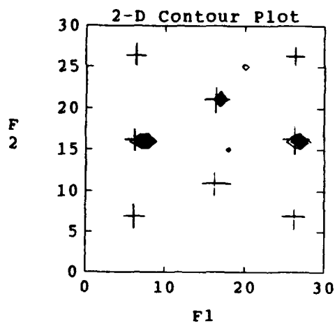
Figure D.11: 2-D AR Spectral Estimate of Eight Sinusoids in Noise (SNR = 10dB) Using the FMV-cycle Method. 1 st & 2 nd quadrant estimates shown, ( k=3 , 9 \times 9 mask).
