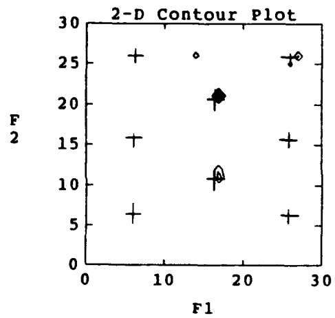
Figure 4.16: 2-D AR Spectral Estimate of Eight Sinusoids in Noise (SNR=10dB) Using the V-cycle Method. 1 st and 2 nd quadrant estimates shown, ( k=5 , 9 \times 9 mask).
