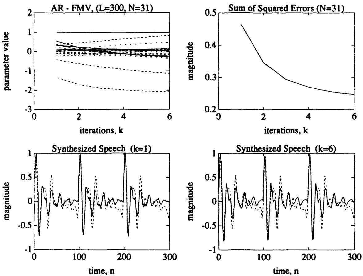
Figure B.9: 31 st Order AR Model of Voiced Speech Using the FMV-cycle Method. Original speech waveform shown in dashed lines, synthesized speech waveform shown in solid lines.
