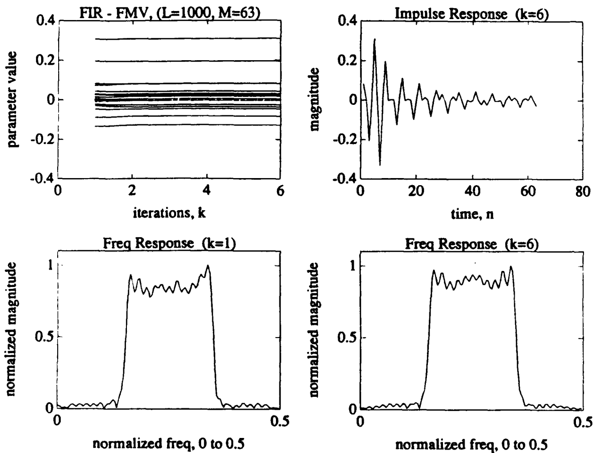
Figure A.7: 63 rd Order FIR Model Using the FMV-cycle Method. Impulse and normalized frequency responses shown using L=1000 data points.
