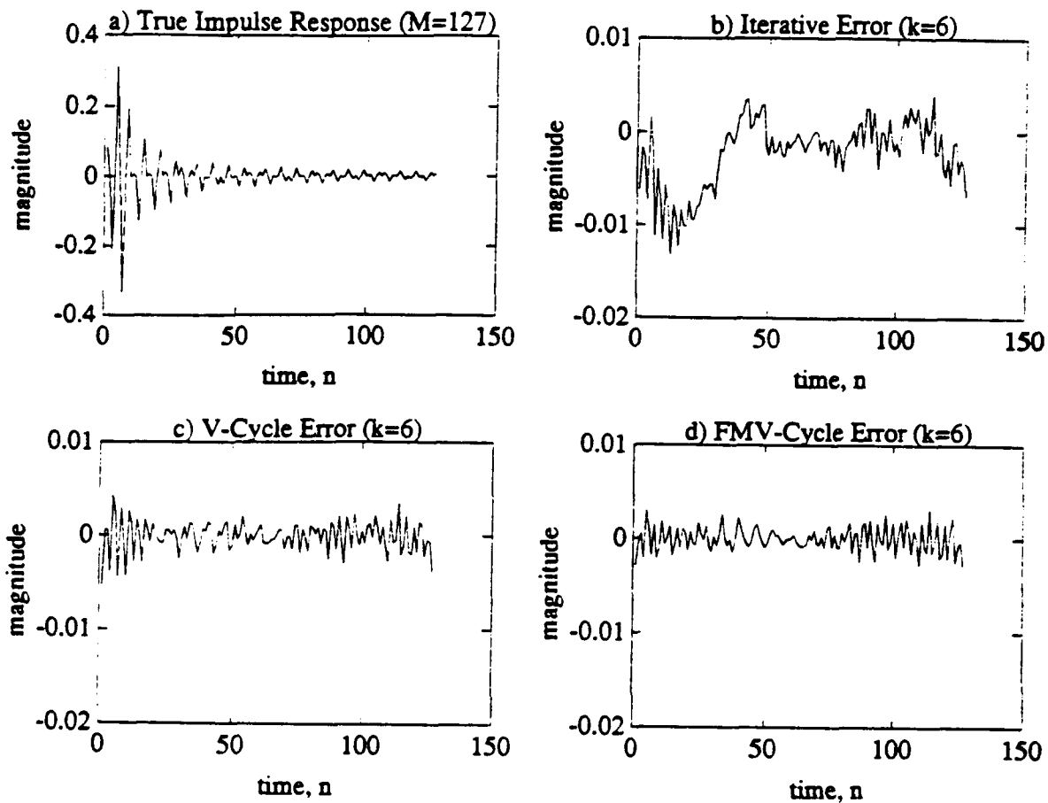
Figure 4.5: 127 th Order FIR Model Impulse Response Error Comparison. a) True System Impulse Response; b) Iterative Method Error; c) V-cycle Method Error; d) FMV-cycle Method Error.
