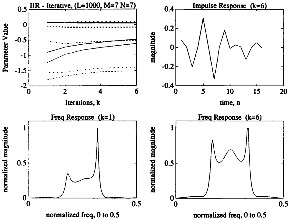
Figure C.1: 7 th Order IIR Model Using the Straight Iterative Method. Impulse and normalized frequency responses shown using L=1000 data points.
