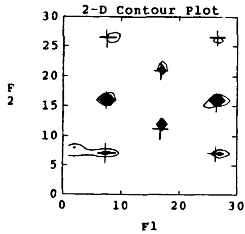
Figure D.6: 2-D AR Spectral Estimate of Eight Sinusoids in Noise (SNR = 10dB) Using the FMV-cycle Method. CQ estimate shown, ( k=1 , 9 \times 9 mask).
