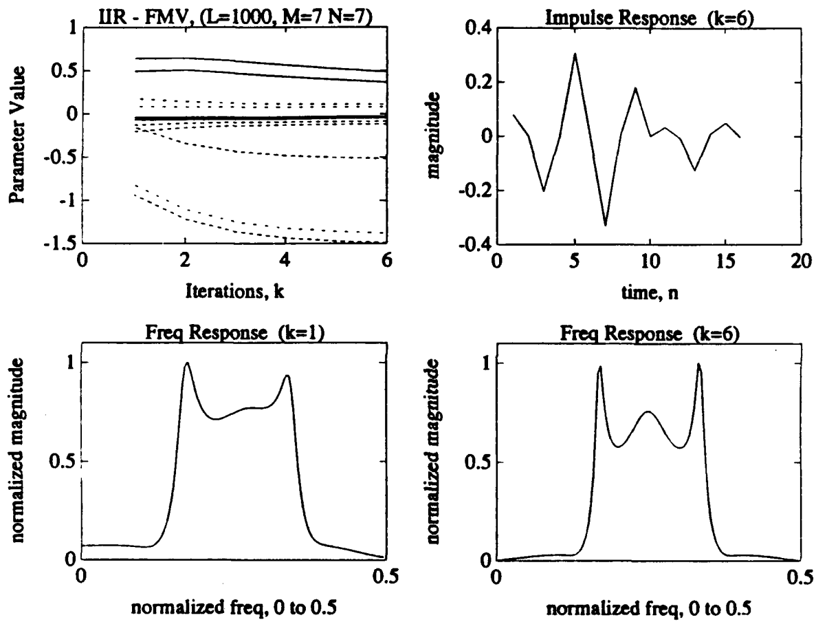
Figure C.3: 7 th Order IIR Model Using the FMV-cycle Method. Impulse and normalized frequency responses shown using L=1000 data points.
