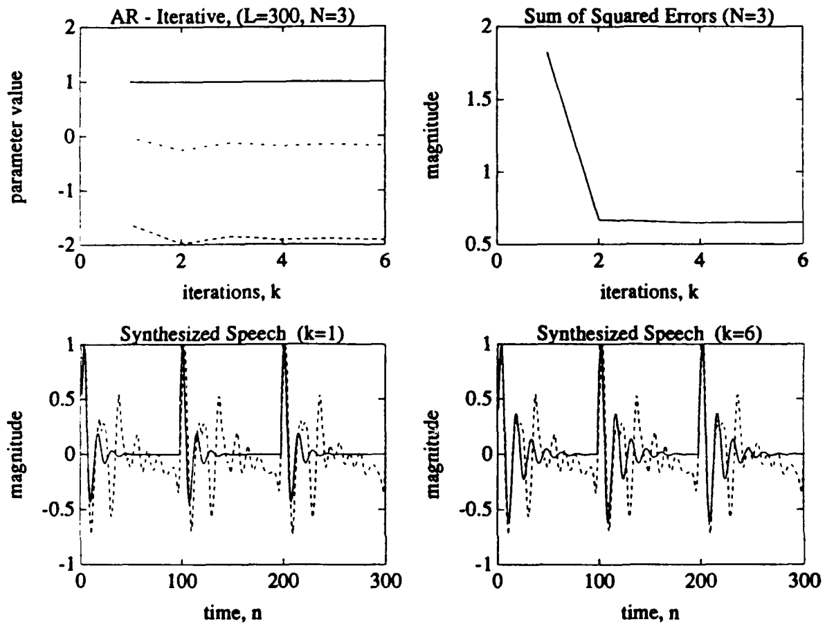
Figure B.1: 3 rd Order AR Model of Voiced Speech Using the Straight Iterative Method. Original speech waveform shown in dashed lines, synthesized speech waveform shown in solid lines.
