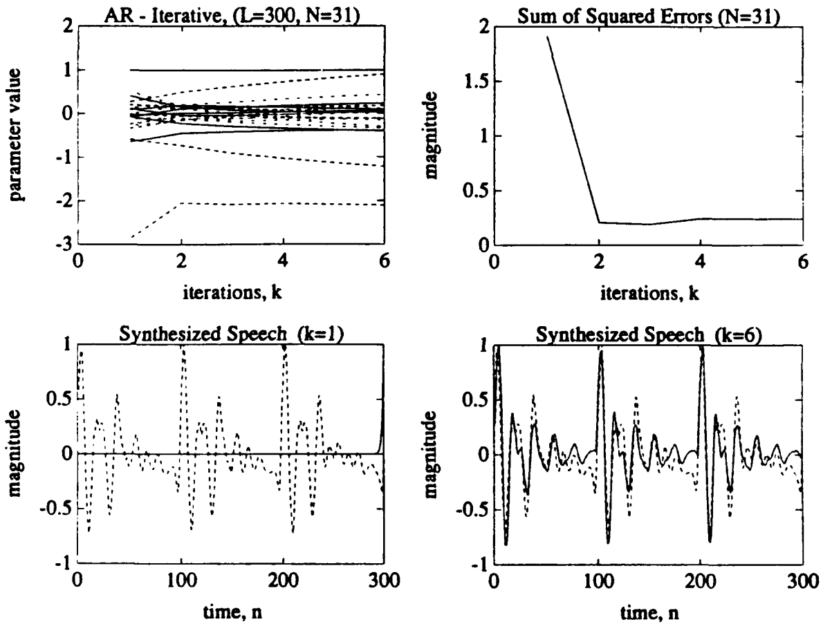
Figure B.7: 31 st Order AR Model of Voiced Speech Using the Straight Iterative Method. Original speech waveform shown in dashed lines, synthesized speech waveform shown in solid lines.
