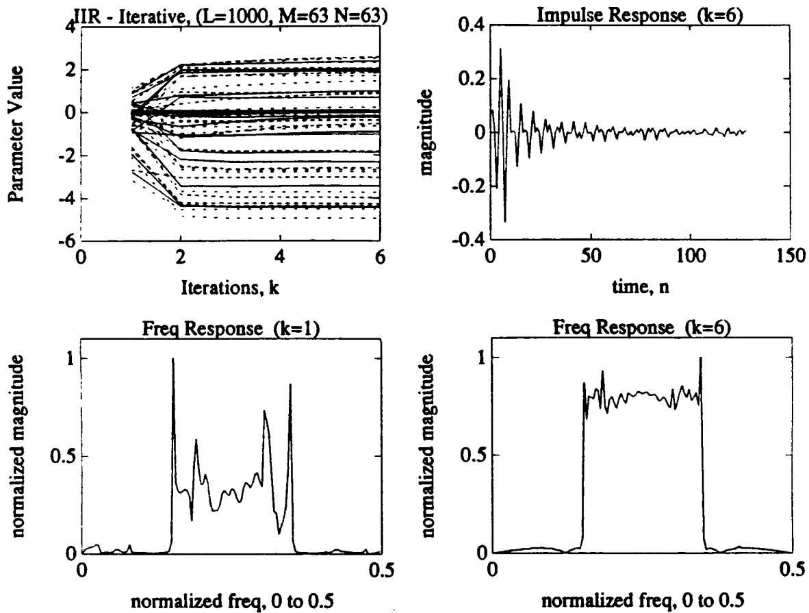
Figure C.10: 63 rd Order IIR Model Using the Straight Iterative Method. Impulse and normalized frequency responses shown using L=1000 data points.
