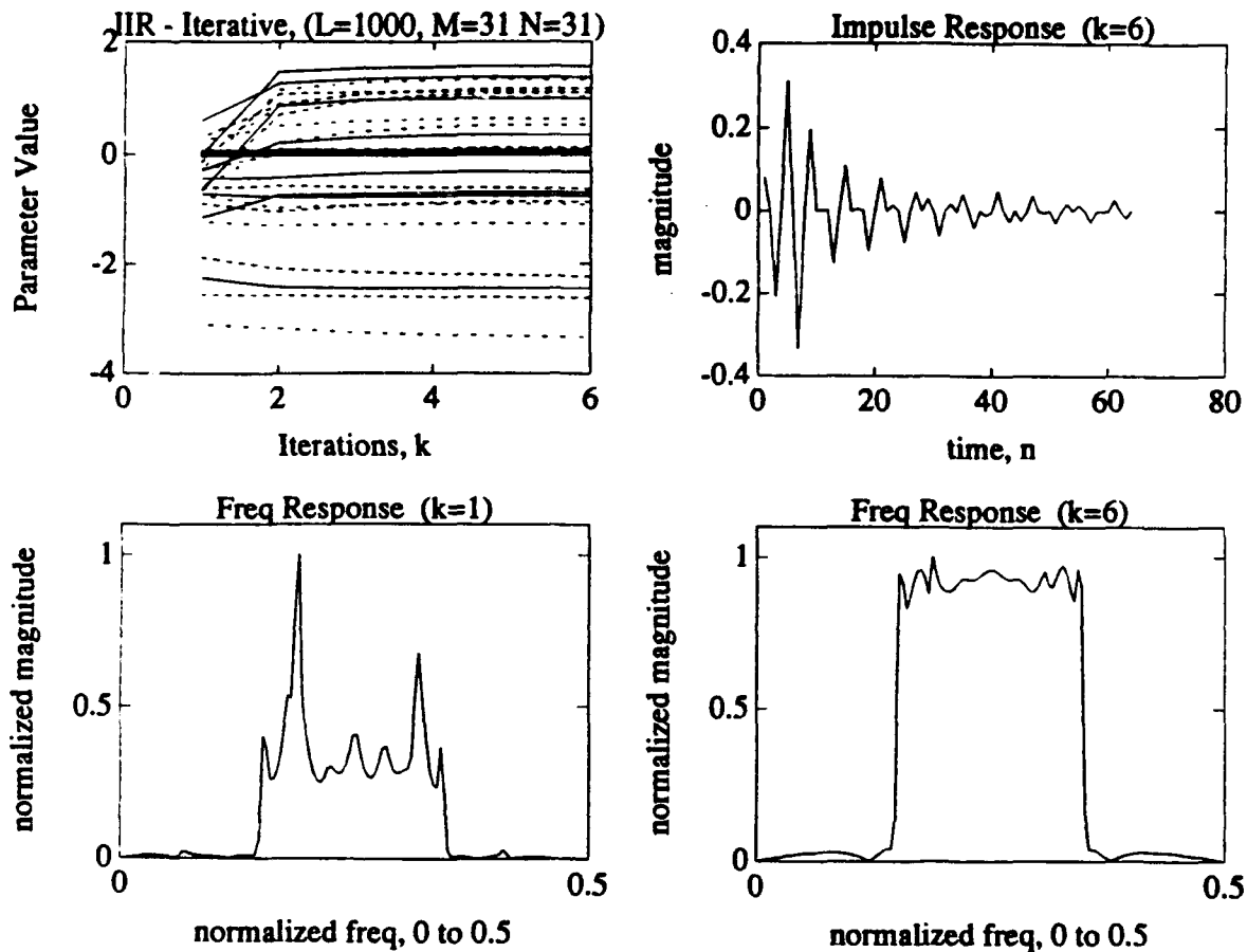
Figure 4.9: 31 st Order IIR Model Using Straight Iterative Method. Impulse and frequency responses are shown using L=1000 data points.
