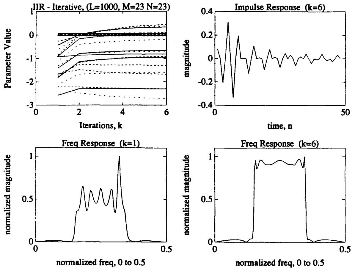
Figure C.7: 23 rd Order IIR Model Using the Straight Iterative Method. Impulse and normalized frequency responses shown using L=1000 data points.
