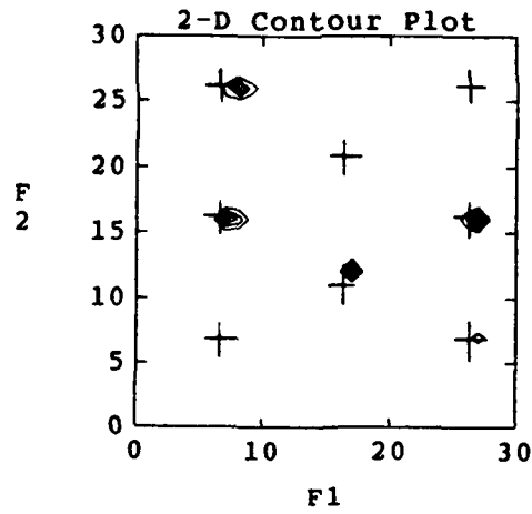
Figure D.12: 2-D AR Spectral Estimate of Eight Sinusoids in Noise (SNR = 10dB) Using the FMV-cycle Method. CQ estimate shown, ( k=3 , 9 \times 9 mask).
