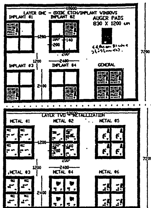
MASK LAYOUTS FOR IMPLANTED CONTACTS Layer One is for the oxide etch and implant mask. Layer Two is for the metal mask.
