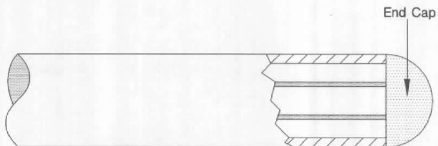
Grounded Junction
