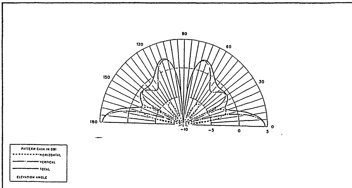
Figure 4.14 E-Field Elevation Pattern for an inverted cone antenna 0.4 m above the wire grid box connected to it by four vertical wires and wire radius 0.01 m, at 20 MHz, \phi = 63.47 degrees.
