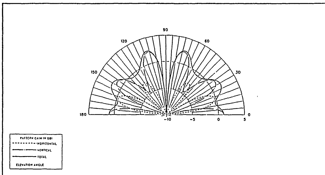
Figure 4.11 E-Field Elevation Pattern for an inverted cone antenna mounted on the wire grid box with 12 feed points, one connection point and wire radius 0.01 m, at 20 MHz, \phi = 63.47 degrees.
