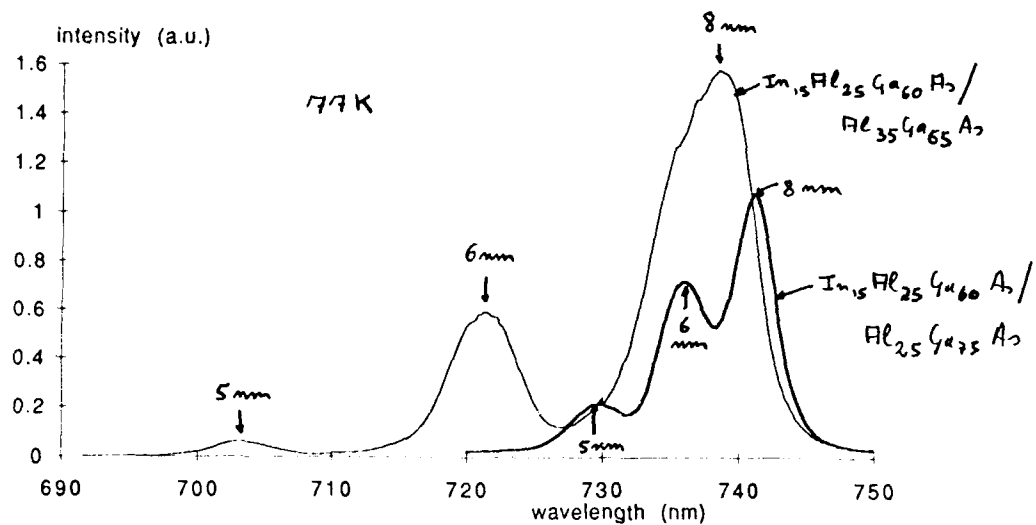
Figure 6.2. Examples of photoluminescence spectra of InAlGaAs/AlGaAs strained quantum wells
