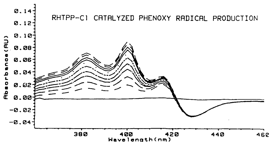
Figure 11: Production of Phenoxy Radical
