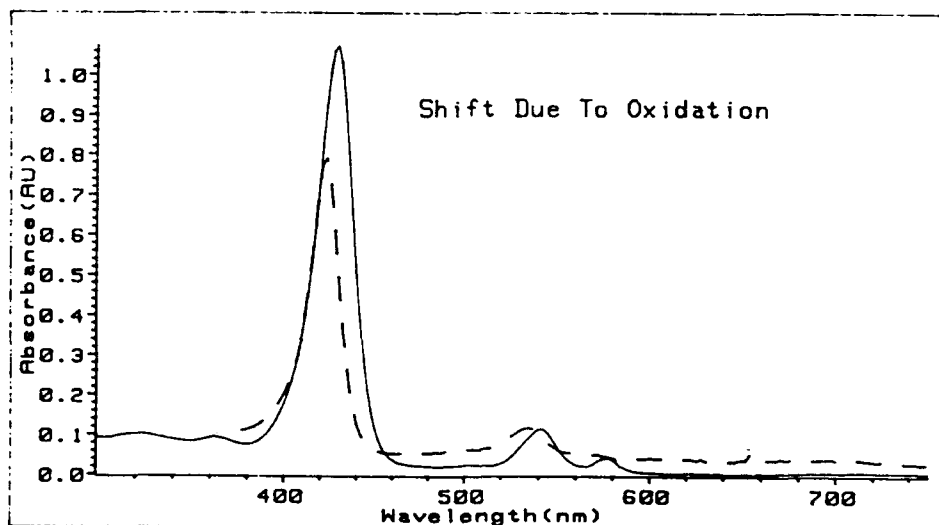
Figure 10: Spectral Shifts Upon Oxidation
