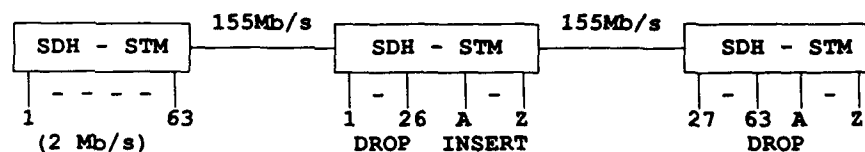
Fig. 4: SDH Drop and Insert Technique
