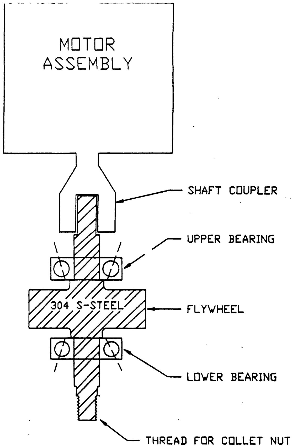
Figure 3-2. Motor and Flywheel Configuration
