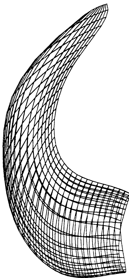
Figure 5.9: B-spline representation of a propeller blade
