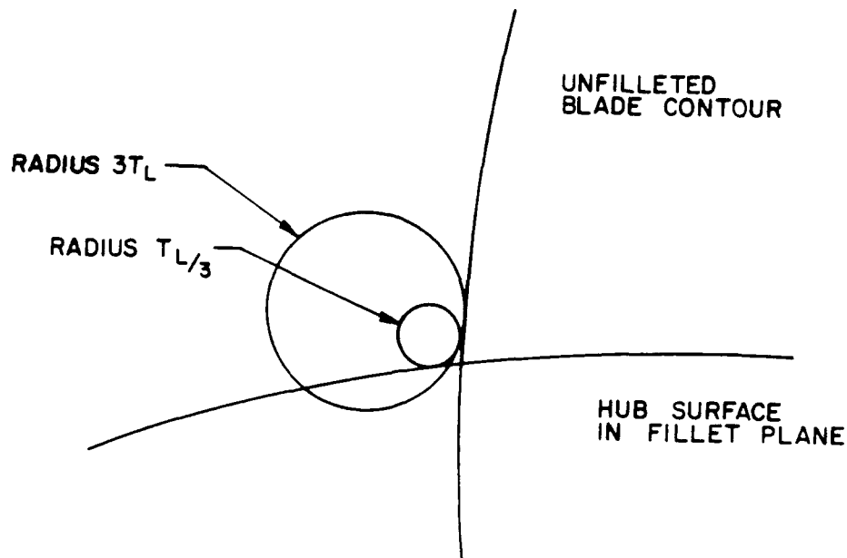
Figure B.1: 3T-T/3 fillet cross-link curve geometry
