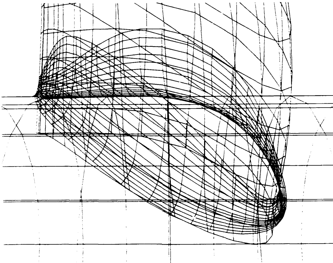
Figure 5.16: 3T-T/3 fillet with blade and hub
