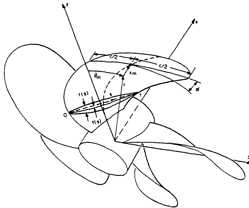
Figure A.1: Propeller blade geometry (from [Kerwin 86])
