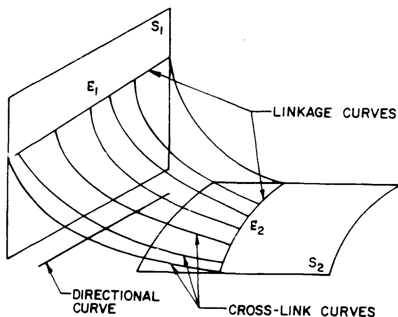
Figure 1.1: Components of a blending surface
