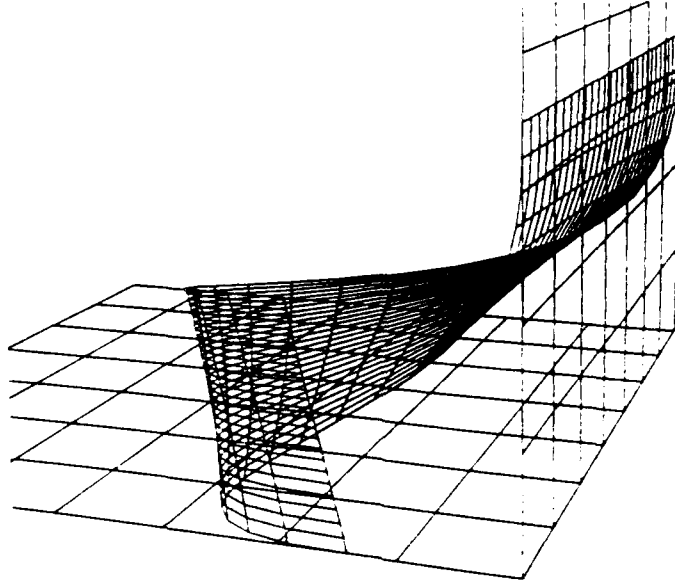
Figure 4.3: Blend with wrong tangent direction
