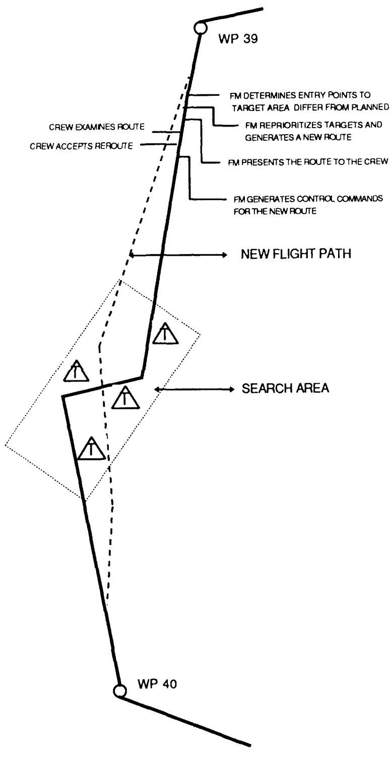
Figure 3-4 Relocatable Target Search Event Sequence
