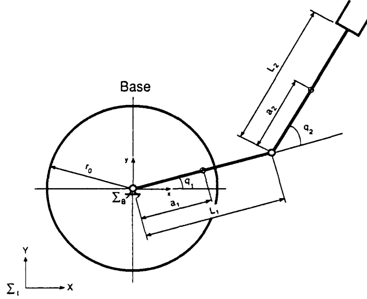
Figure 2: A free-flying planar space robot system.
