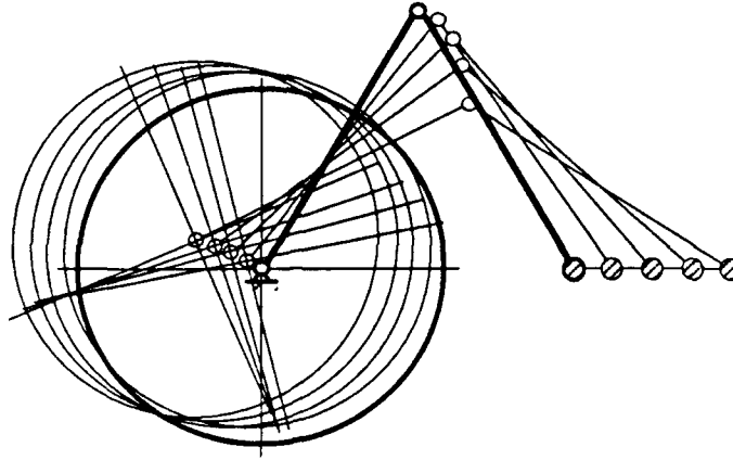
Figure 3: Motion trajectory of a planar free-flying robot system.
