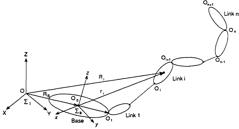
Figure 1: A free-flying space robot system model.
