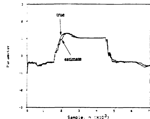
Figure 8: Simulation results of the selective forgetting SM-WRLS algorithm with suboptimal data selection for the word six. 1.86% of the data is employed in the estimation process.
