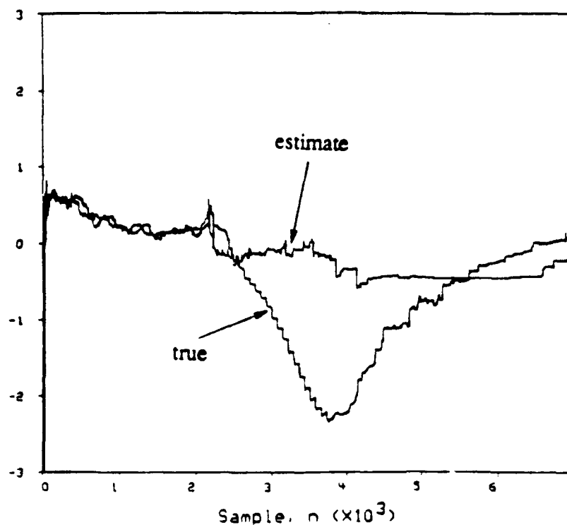
Figure 2: "Nonadaptive" SM-WRLS algorithm applied to the estimation of parameter a_{4s} . Only \rho = 0.079 of the data is used, but the estimate fails to track the true parameter.
