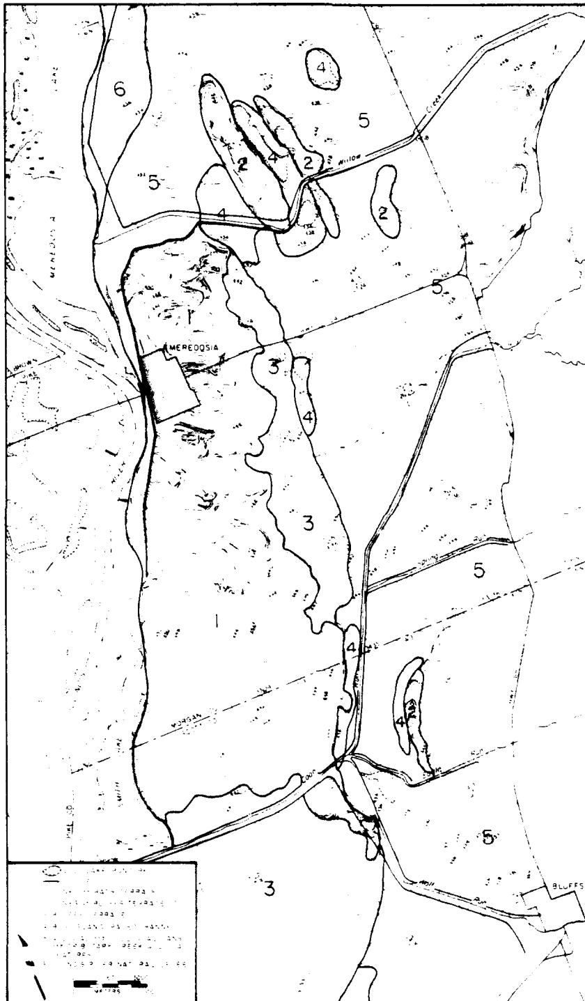
Figure 4. Geomorphology of the Meredosia Village District.
