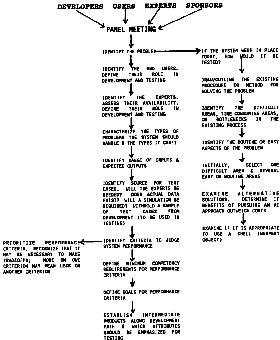
Figure 4 Requirements Generation Process
