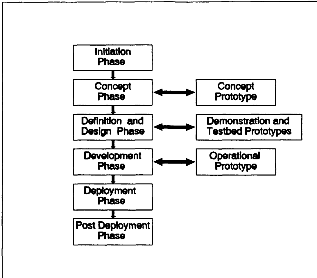
Figure 2 Expert system life cycle
