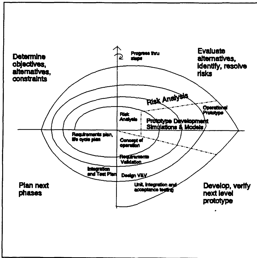
Figure 1 (Boehm, 1988) Spiral software development model
