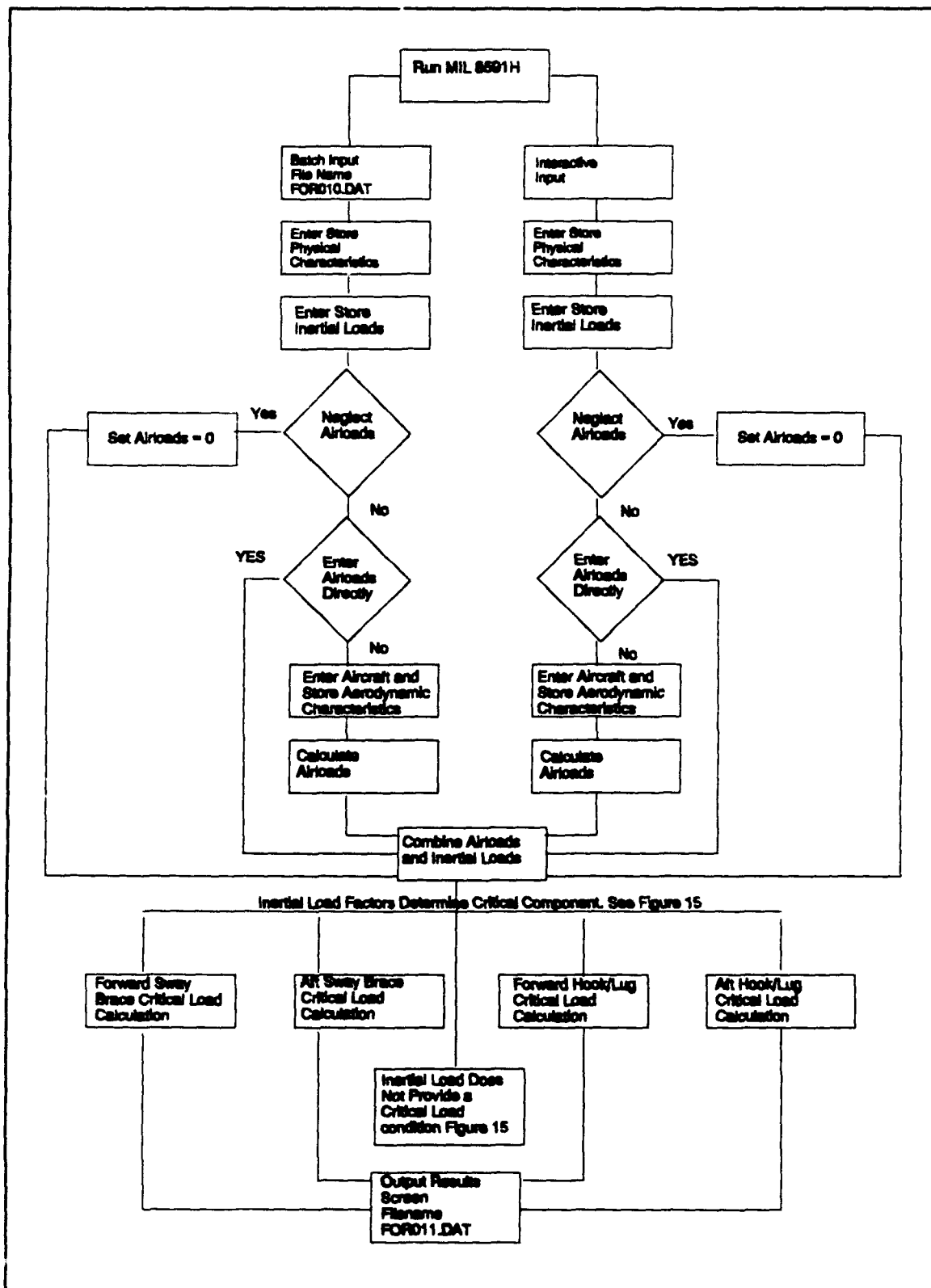
Figure 6. Program Flowchart
