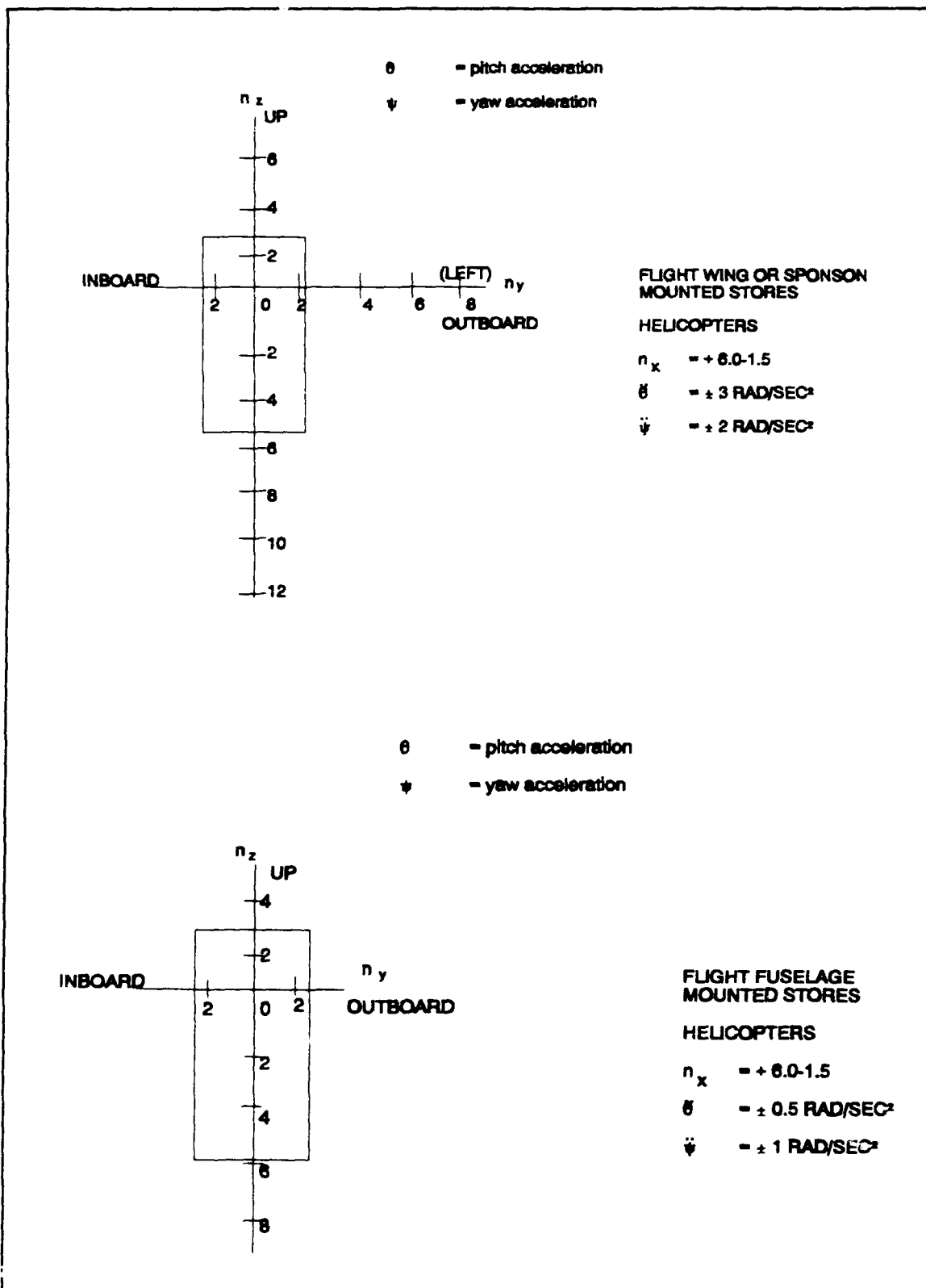
Figure 14. Inertial Load Factors for Helicopters
