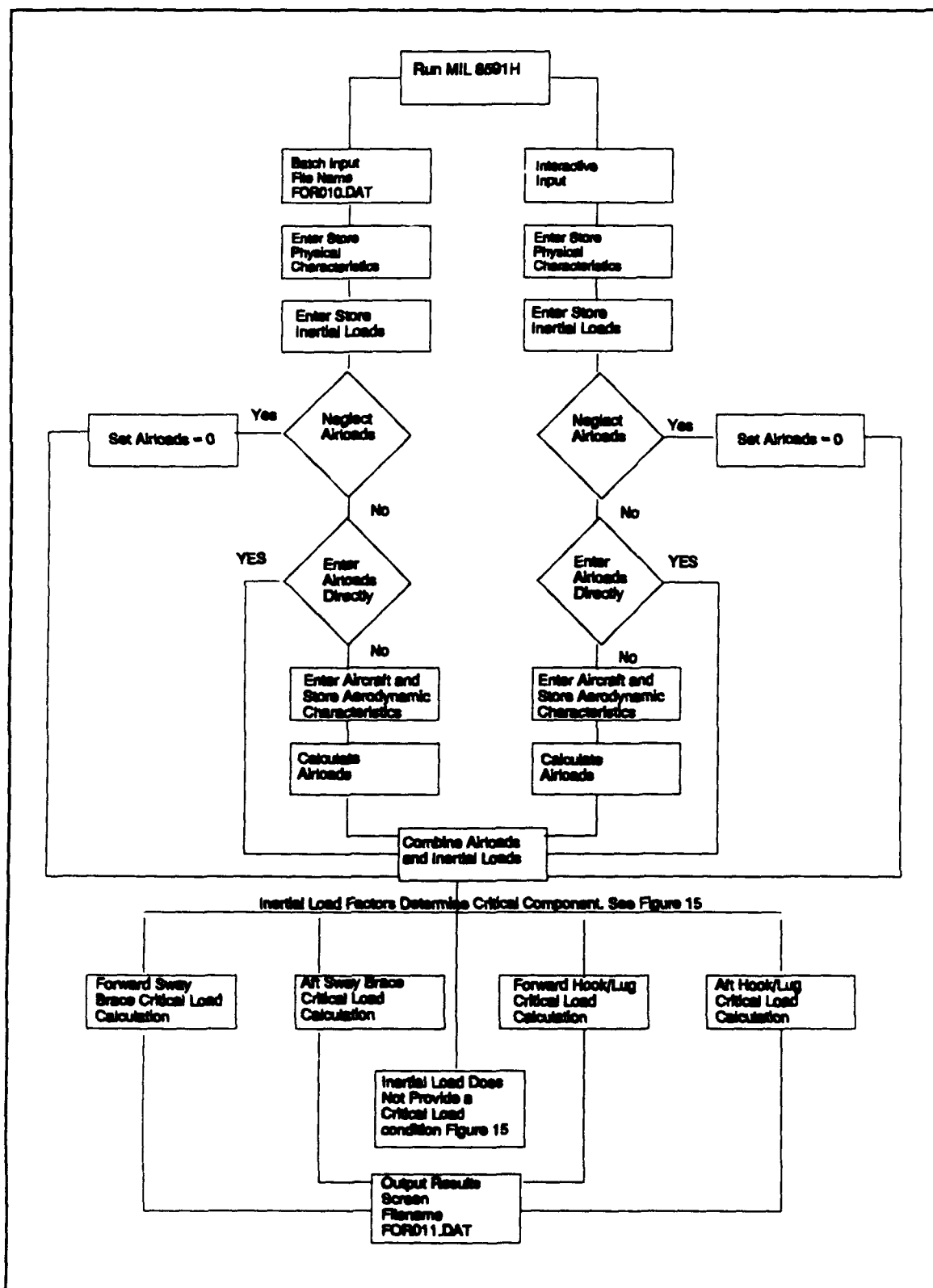
Figure 8. Program Flowchart
