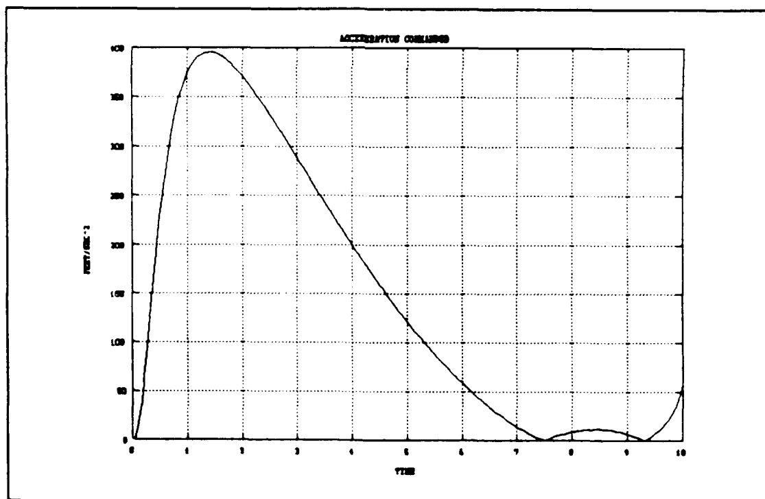
Figure 12. Commanded Acceleration
