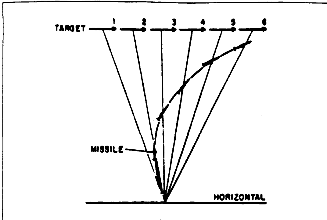
Figure 2. Line-of-Sight Trajectory
