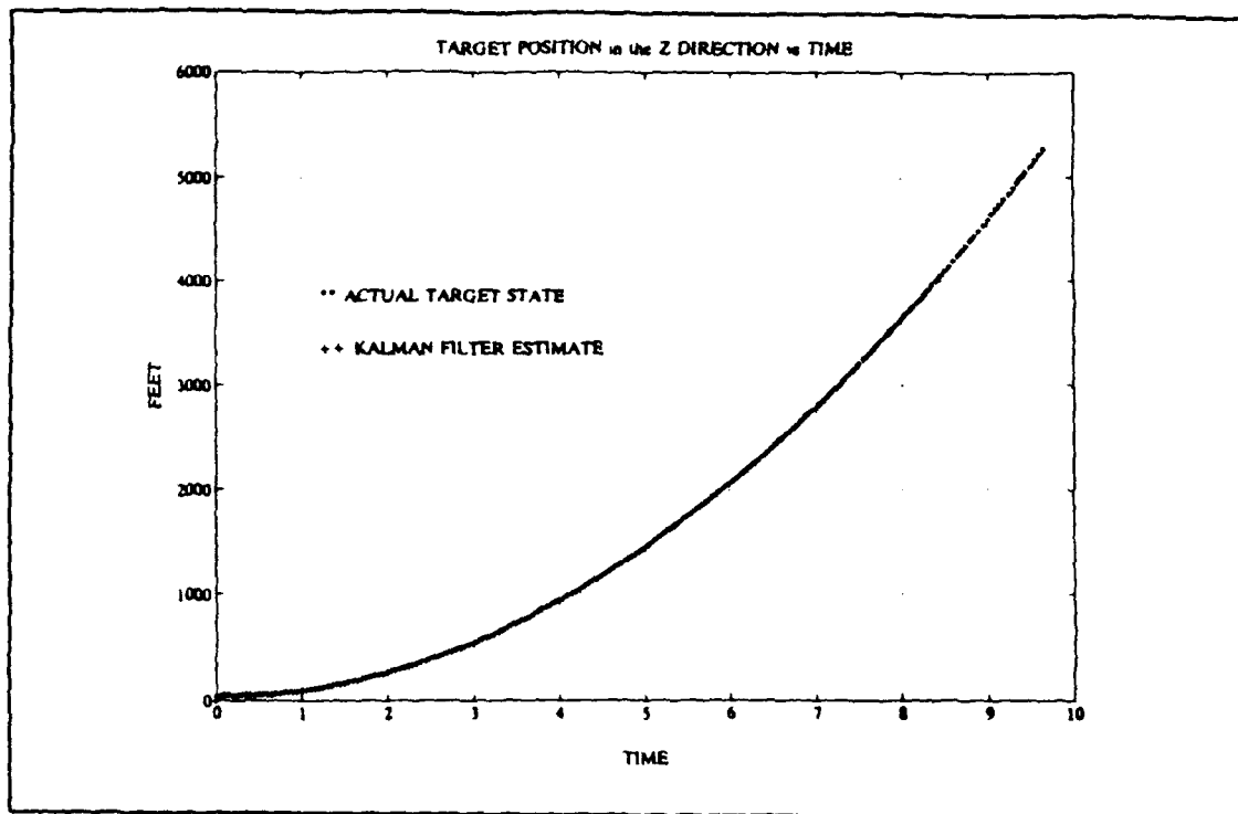
Figure 59. Target Position in the Z Direction
