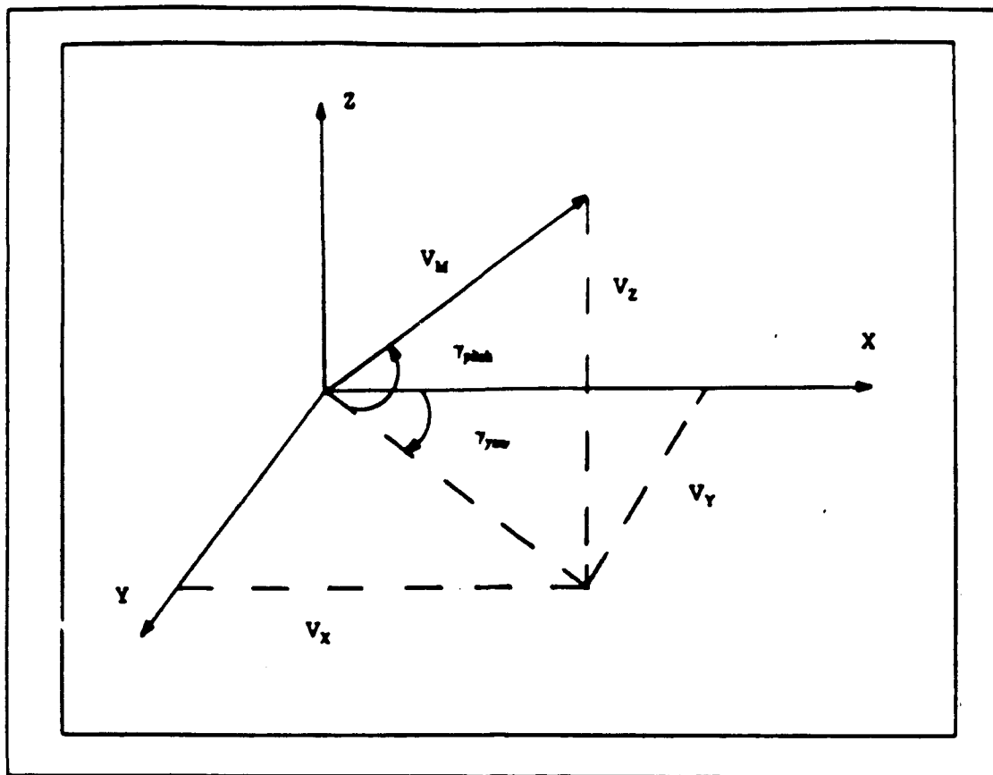
Figure 6. Flight Path Geometry
