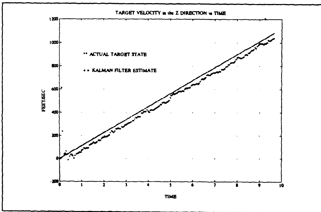
Figure 60. Target Velocity in the Z Direction
