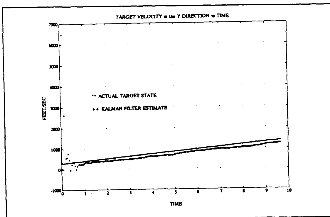
Figure 58. Target Velocity in the Y Direction
