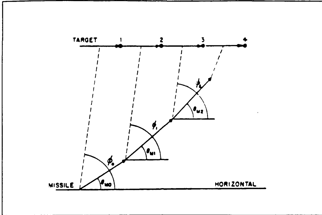
Figure 3. Proportional Guidance Trajectory
