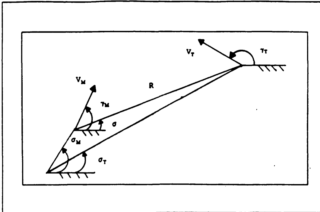
Figure 5. Intercept Geometry for Proportional Navigation
