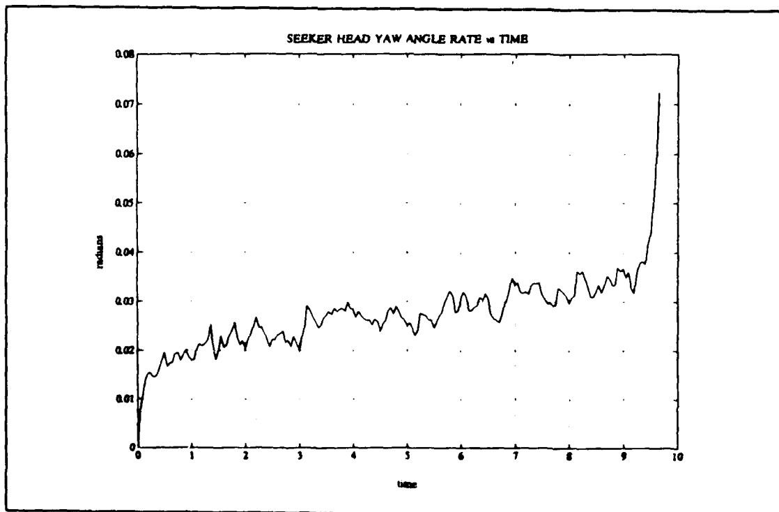
Figure 64. Seeker Head Angle Rate in the Yaw Plane
