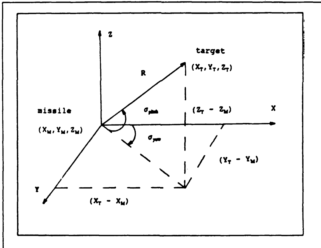
Figure 7. Sightline Geometry
