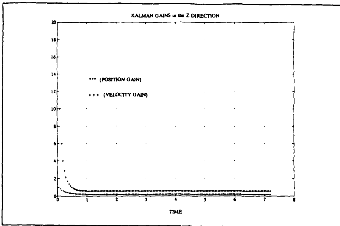
Figure 63. Kalman Gains in the Z Direction
