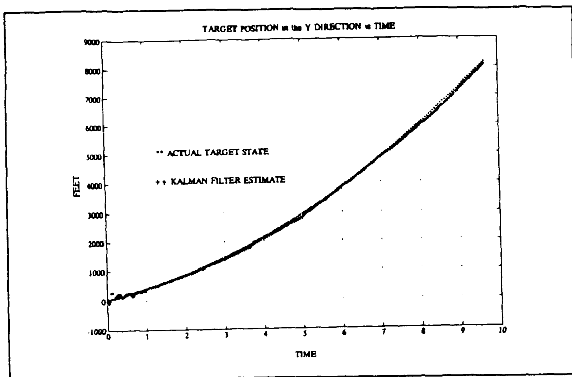
Figure 57. Target Position in the Y Direction
