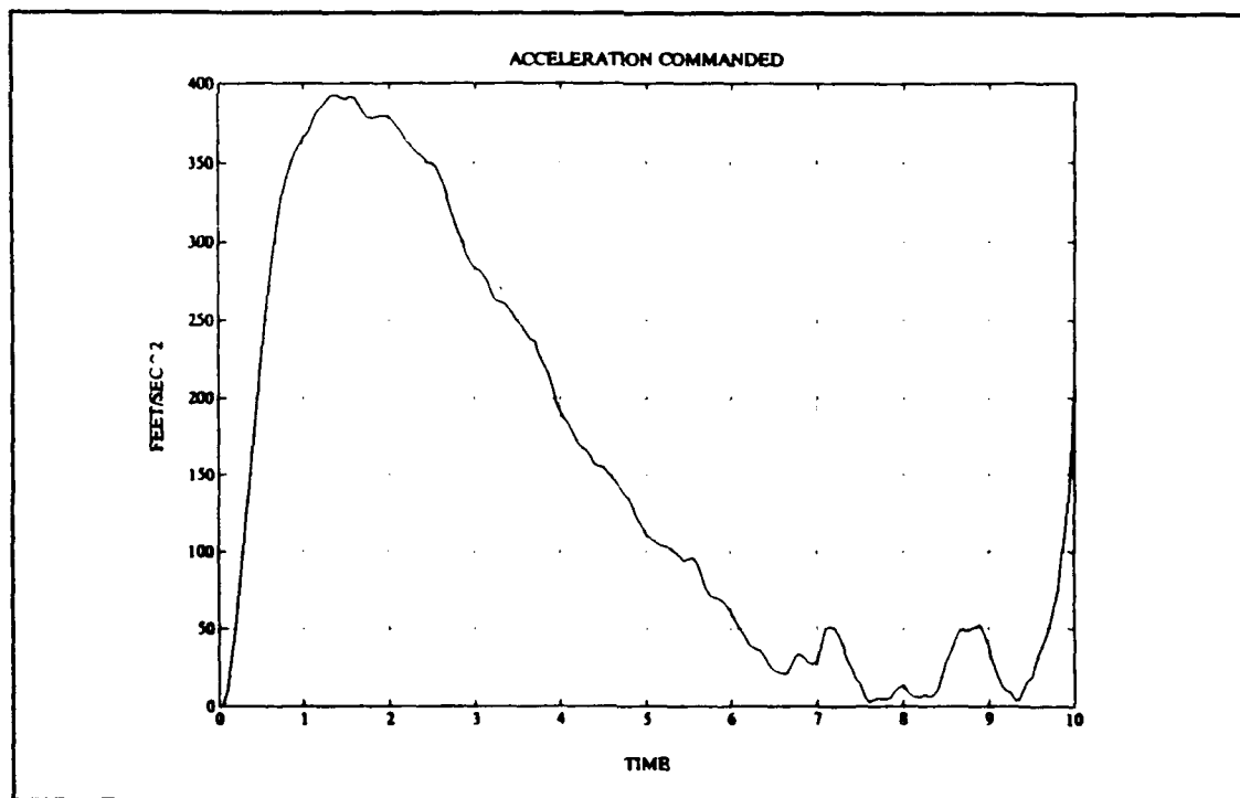
Figure 54. Acceleration Commanded
