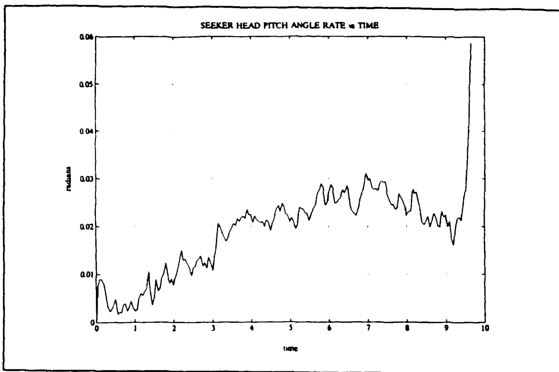
Figure 65. Seeker Head Angle Rate in the Pitch Plane
