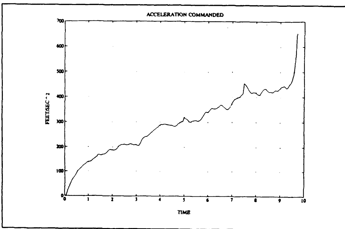
Figure 66. Commanded Acceleration
