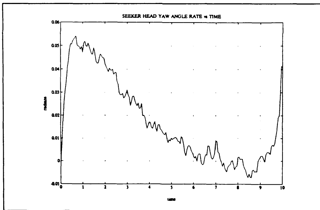
Figure 52. Seeker Head Angle Rate in the Yaw Plane
