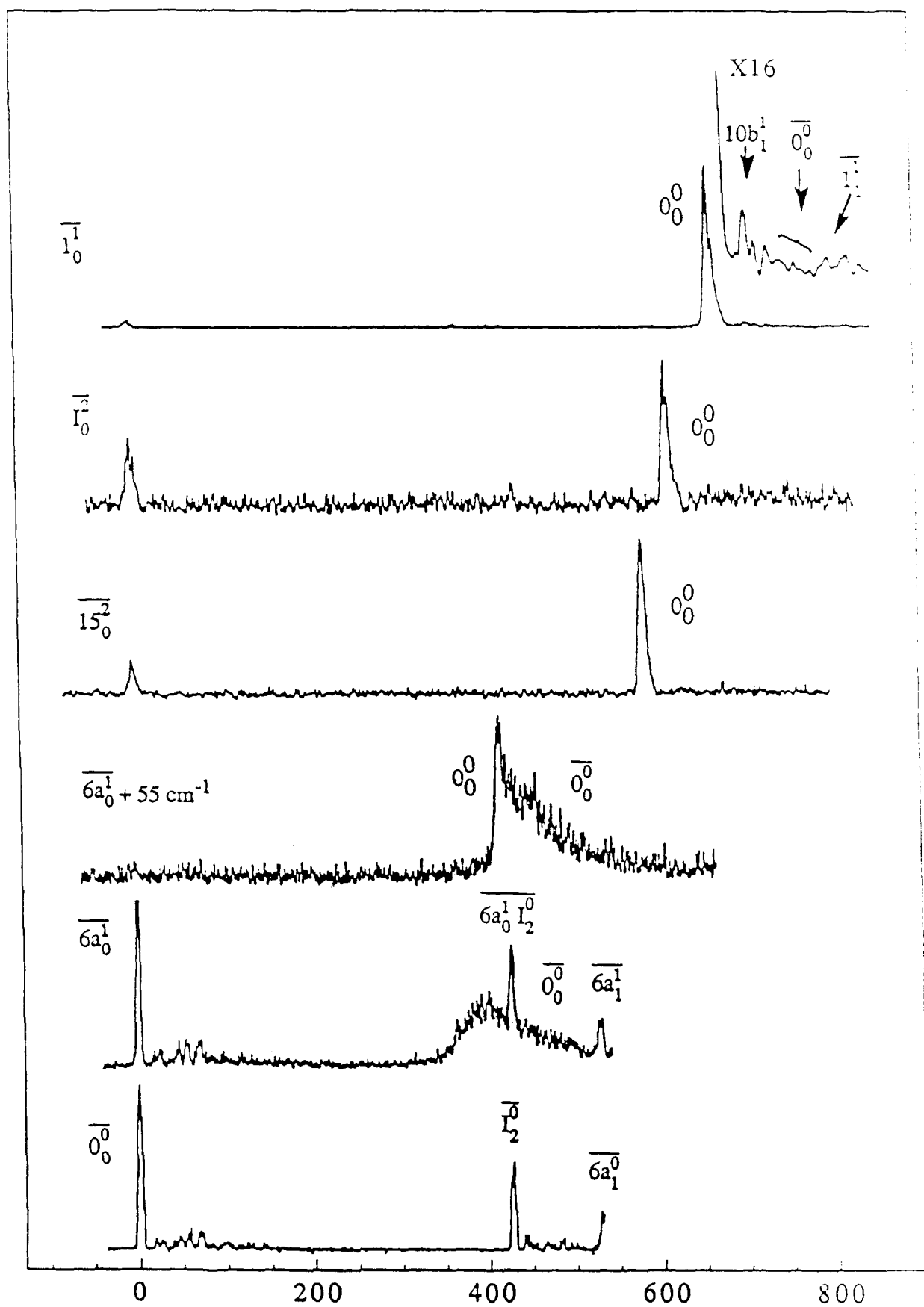
Relative Energy (cm -1 )
