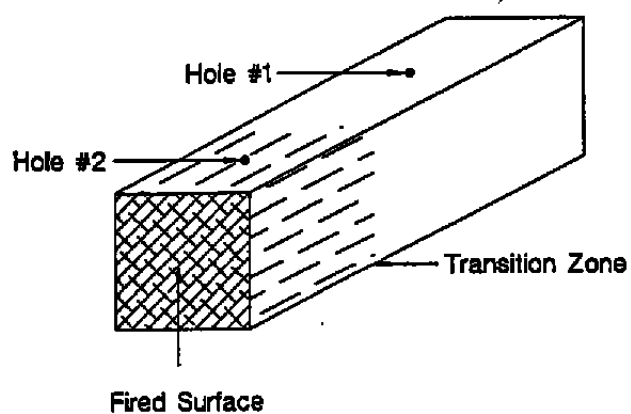
Figure 1. Carbon Phenolic Test Fixture For Laboratory Tests.
