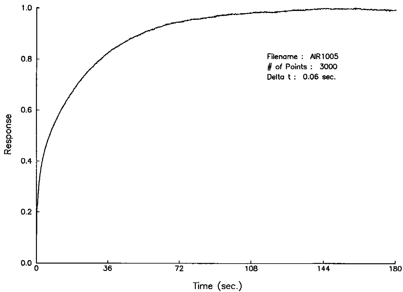
Figure 3.4.6 Averaged LCSR Transient for Sensor Tag No. AF #04 in Air .
