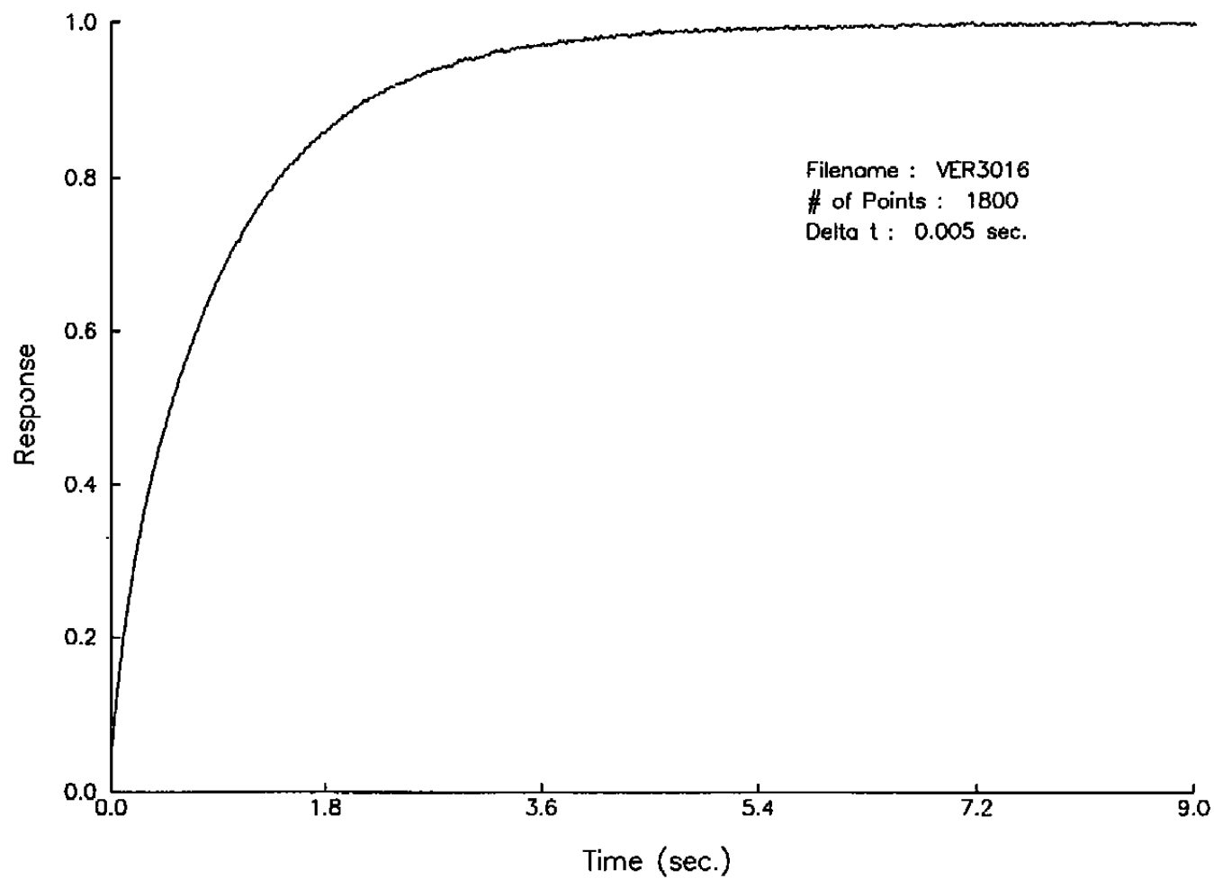
Figure 3.3.2. Averaged LCSR Transient for Sensor Tag No. AF #29 in water .
