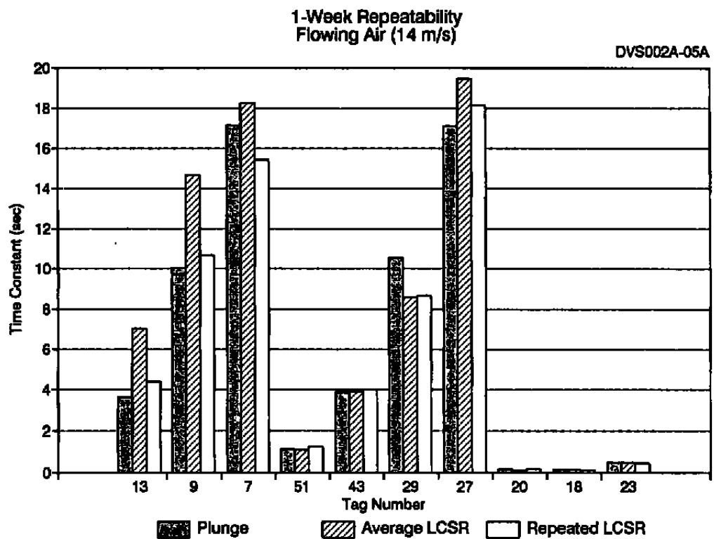
Figure 7.4. One Week Repeatability (14 m/s Air).
