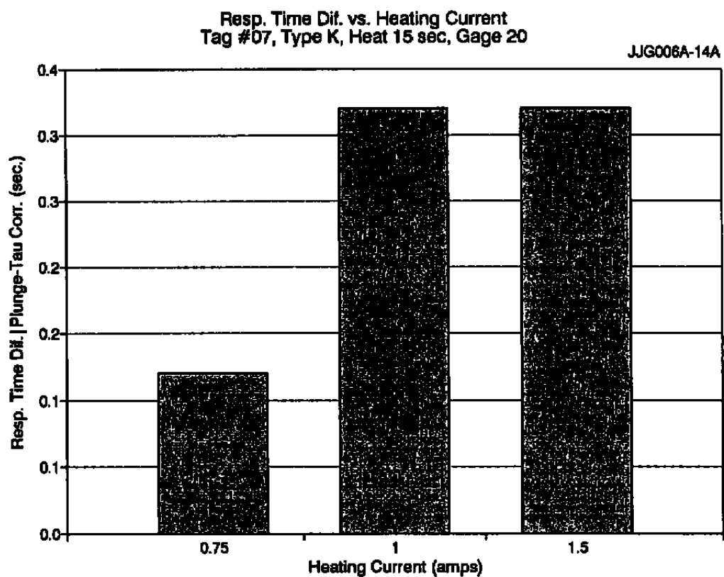
Figure 4.6. Example of Thermocouple with Increasing Errors as Current was Increased. (AF#07, 15 Second Heating Time.)
