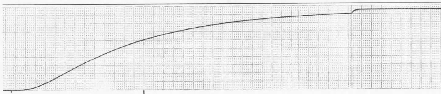
Figure 2.5. Typical Plunge Response for Type "J" Thermocouple in Water.
