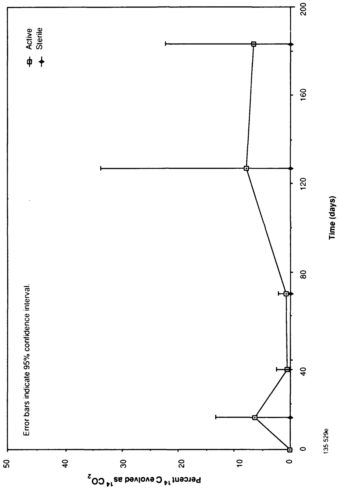
Figure 4-11. ^{14}\text{C} -DIMP evolved as ^{14}\text{CO}_2 in RMA uncontaminated soil.
