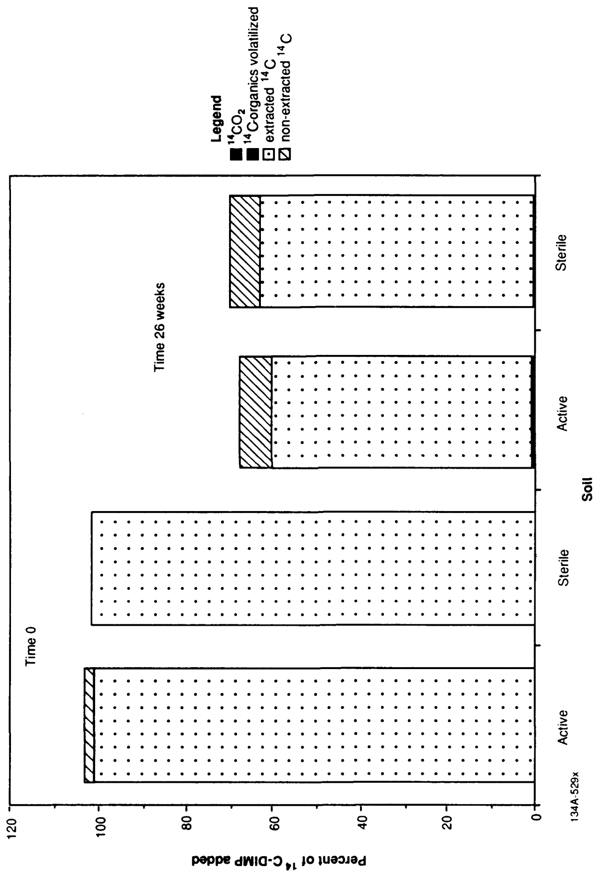
Figure 4-24. Mass balance of ^{14}\text{C} -PCPMSO in RMA uncontaminated soil.
