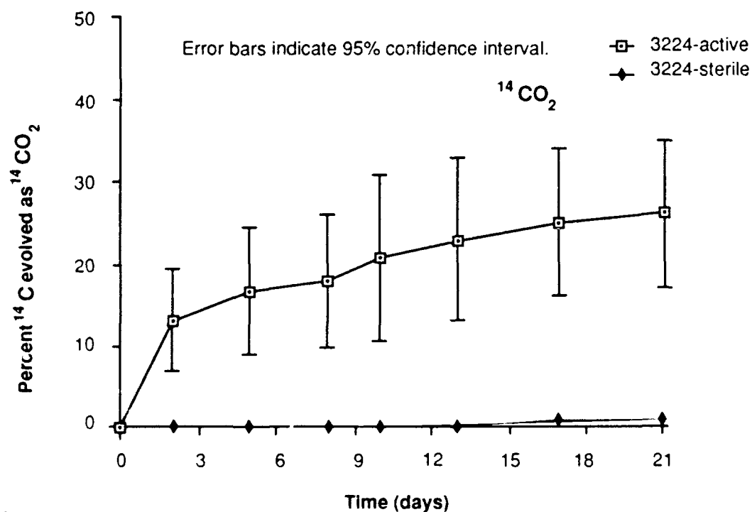
Figure 4-4. Plot of percent ^{14}\text{C} -glucose, ^{14}\text{C} -amino acids, and ^{14}\text{C} -acetate mineralized in RMA soil #3224.
