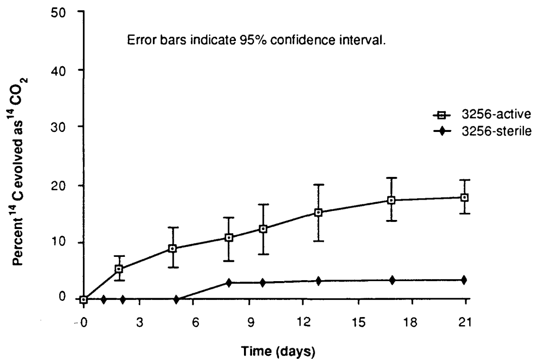
Figure 4-5. Plot of percent ^{14}\text{C} -glucose, ^{14}\text{C} -amino acids, and ^{14}\text{C} -acetate mineralized in RMA soil #3256.
