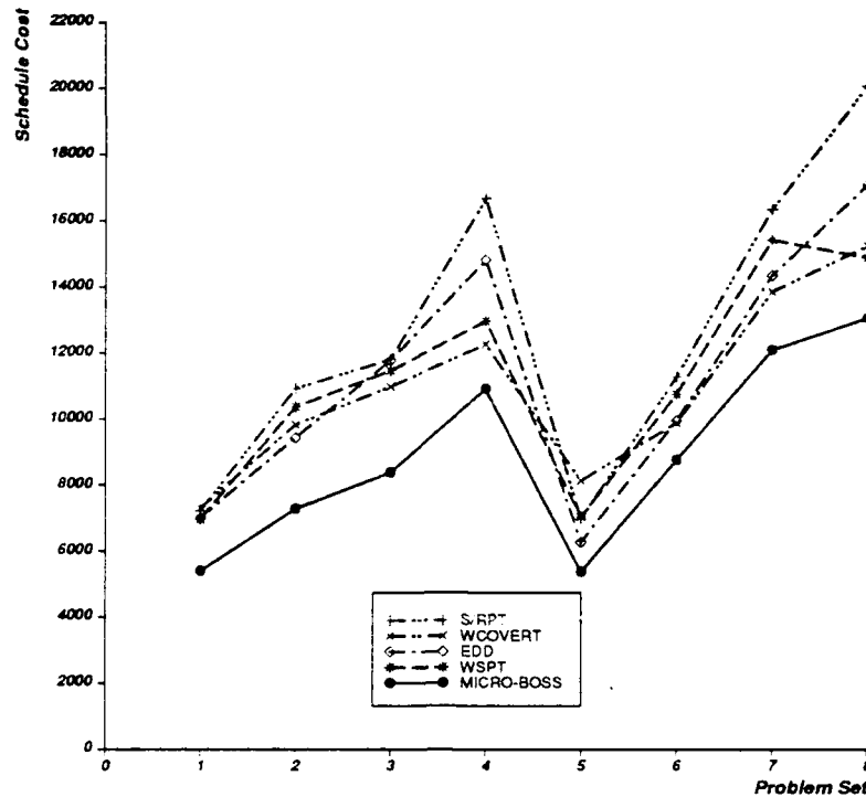
Figure 8: Comparison of the costs of schedules produced by MICRO-BOSS, the WSPT, EDD, S/RPT and WCOVERT dispatch rules.
