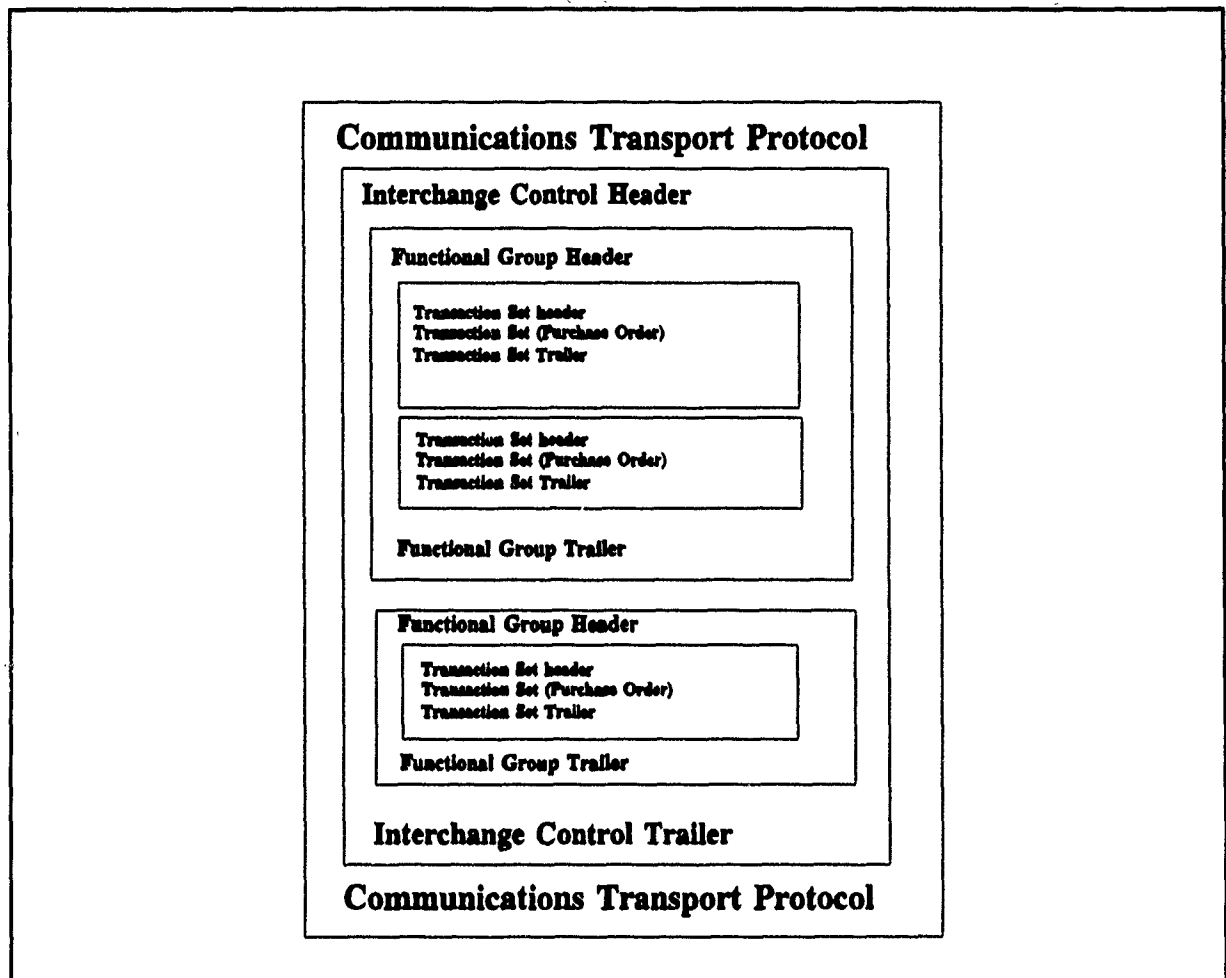
Figure 7 Data structure of an EDI transaction
