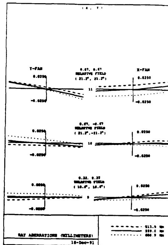
Figure 4.4. Tangential and sagittal ray fan plots for 11 field angles for a pupil size of 3mm.
