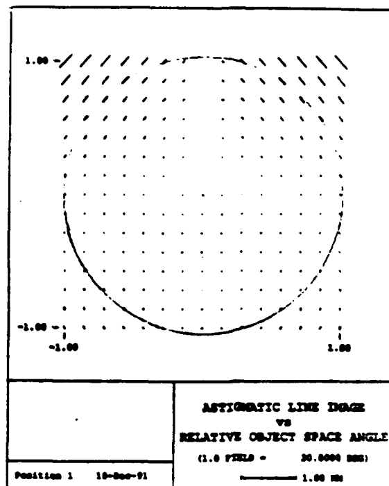
Figure 4.5. Astigmatic line image over a 60x60-degree FOV. The circle drawn on this picture represents a circular FOV of 60 degrees. This is a typical image of an optical system well compensated for astigmatism. Note the scale chosen to represent the lines.
