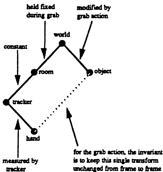
Figure 2. Coordinate systems diagram for grabbing an object
