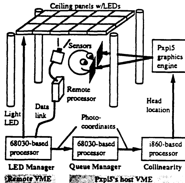
Figure 5: System Dataflow
