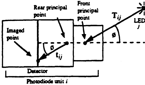
Figure 9: Optical model
