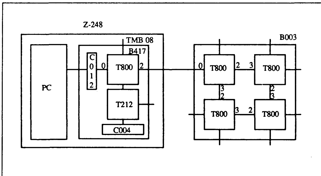
Figure 3: Connection Network of Transputers
