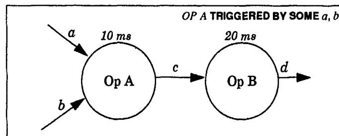
Figure 2.9 PSDL data-flow diagram with control constraints
