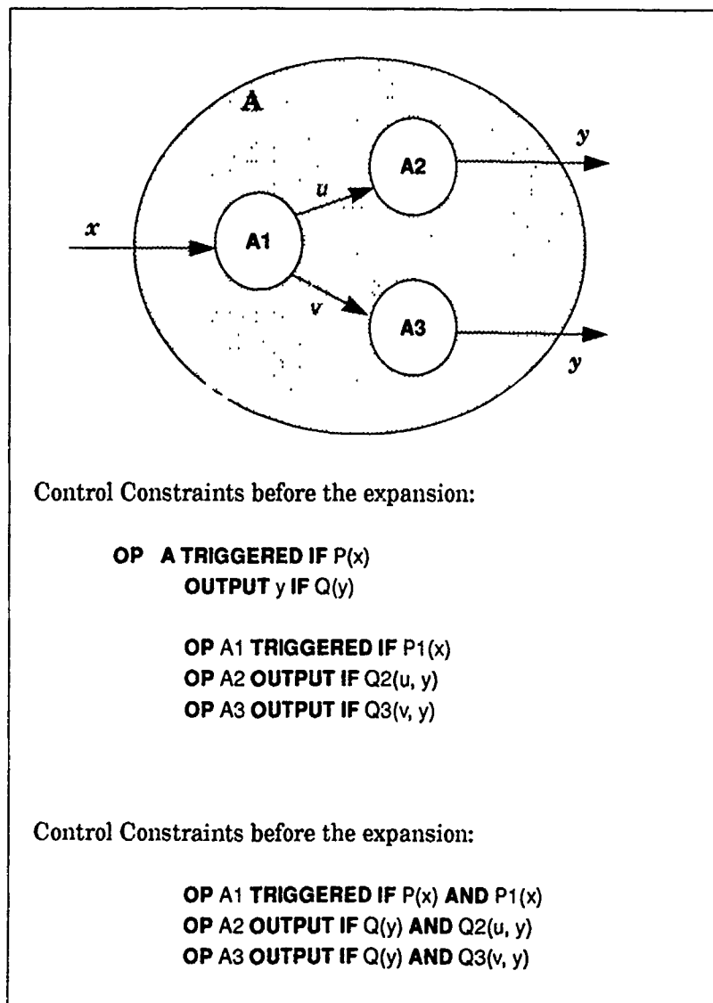
Figure 3.17 The Inheritance of Input and Output Guards
