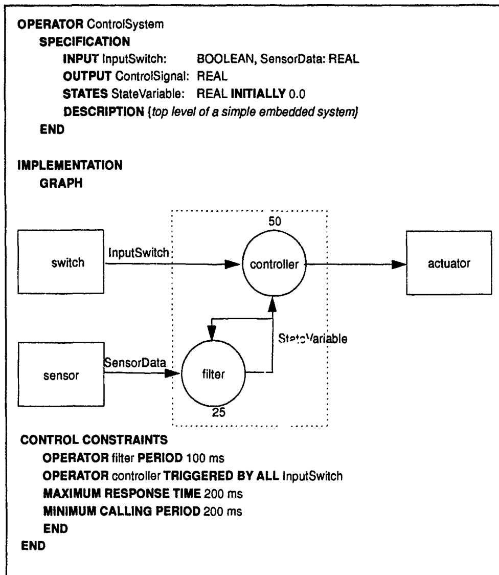
Figure 2.10 Example of an Augmented Data-flow diagram in PSDL
