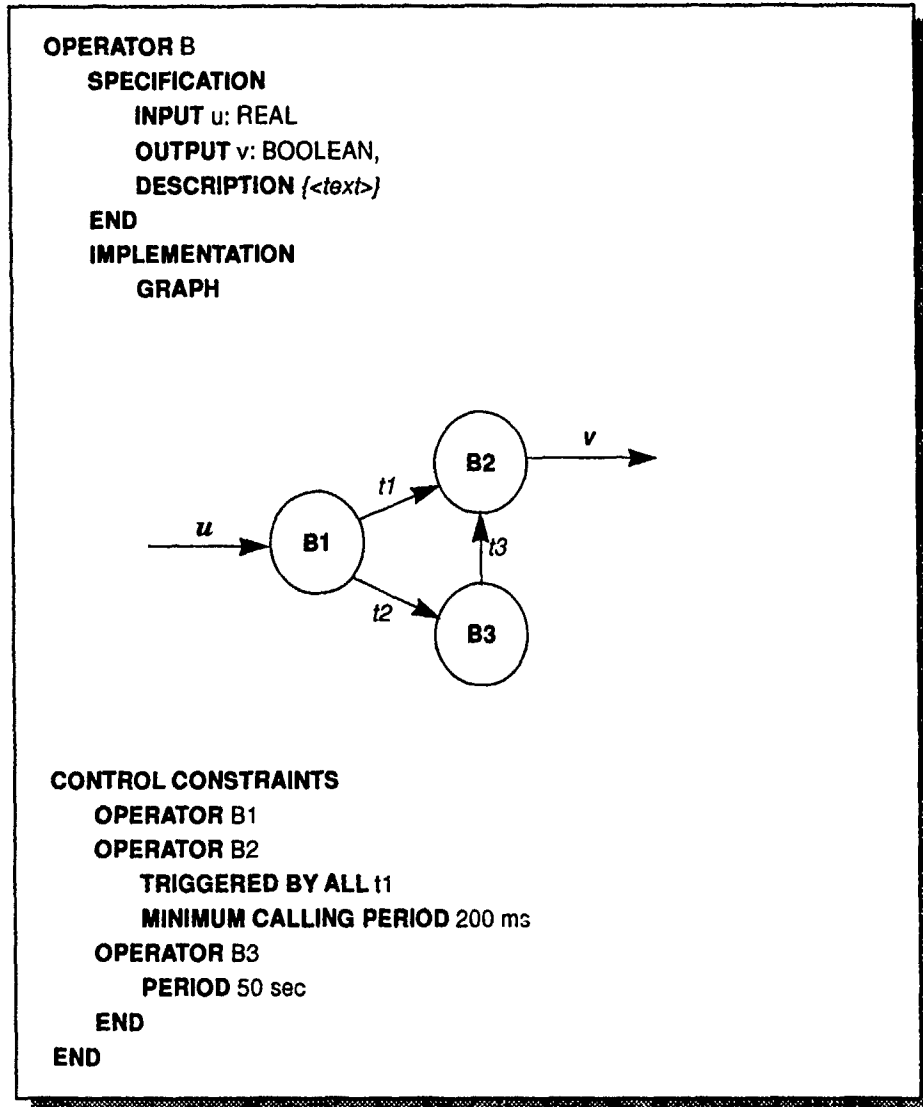
Figure 3.12 PSDL Code for Operator B
