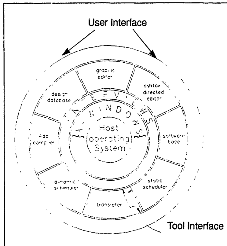
Figure 2.5 CAPS Advanced Rapid Prototyping Environment: ARPE
