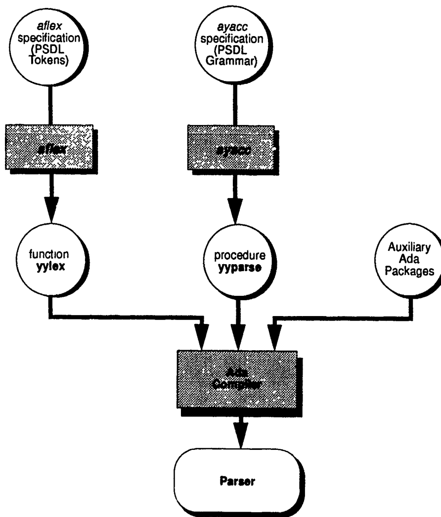
Figure 3.7 Parser Generation Process
