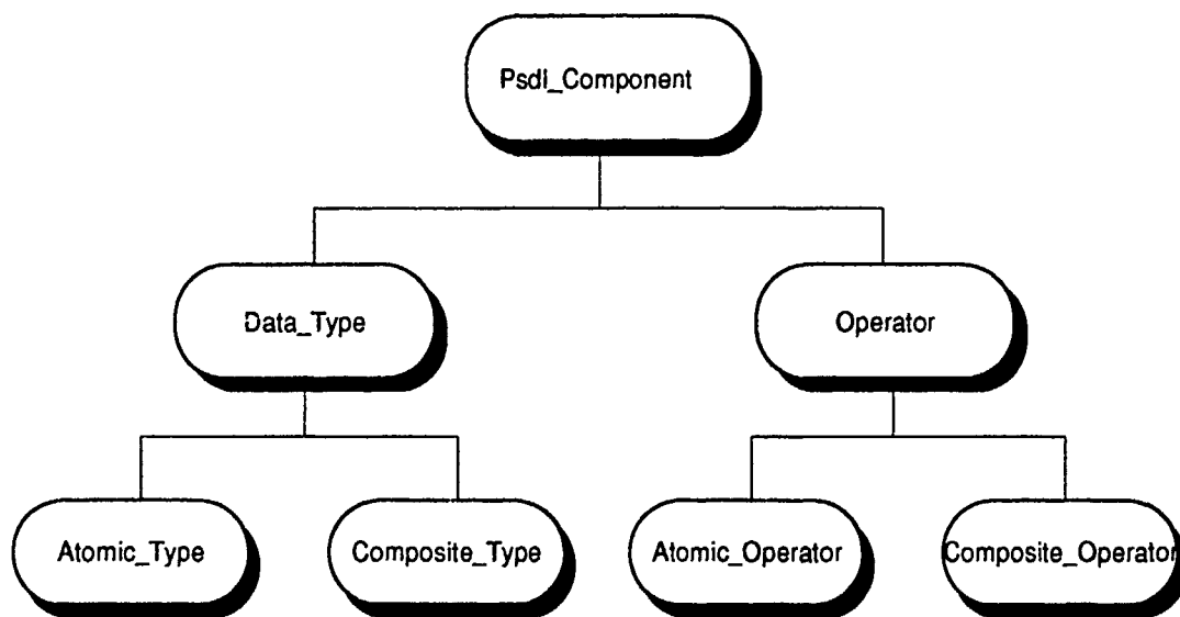
Figure 3.4 PSDL ADT Type Hierarchy
