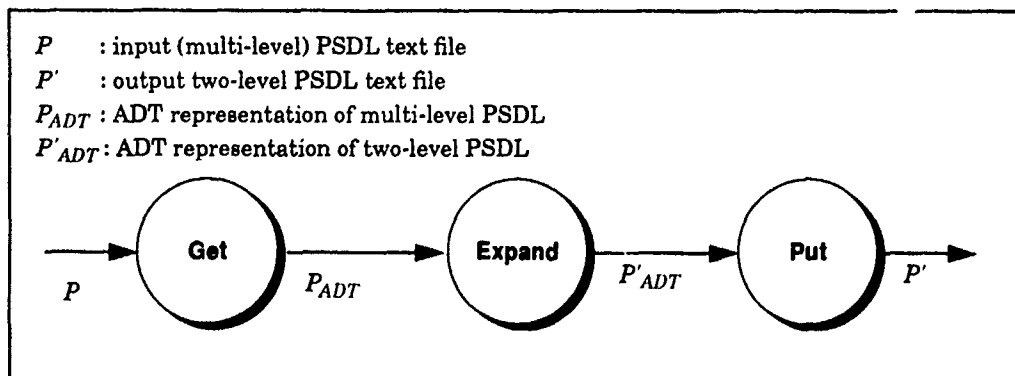
Figure 3.2 The Steps in the Expanding Process
