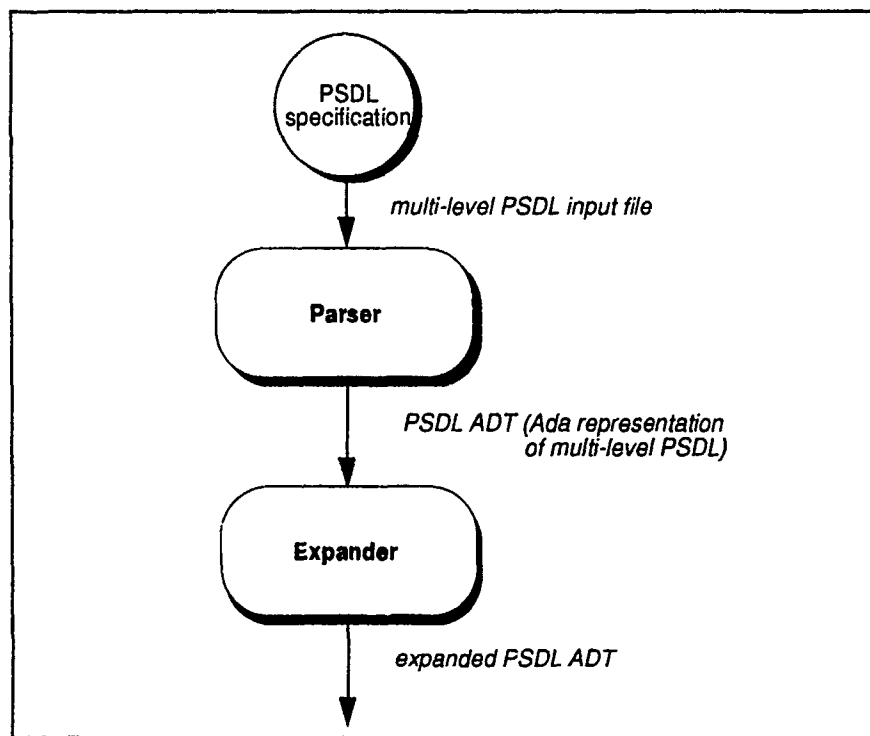
Figure 3.1 The Expansion Process
