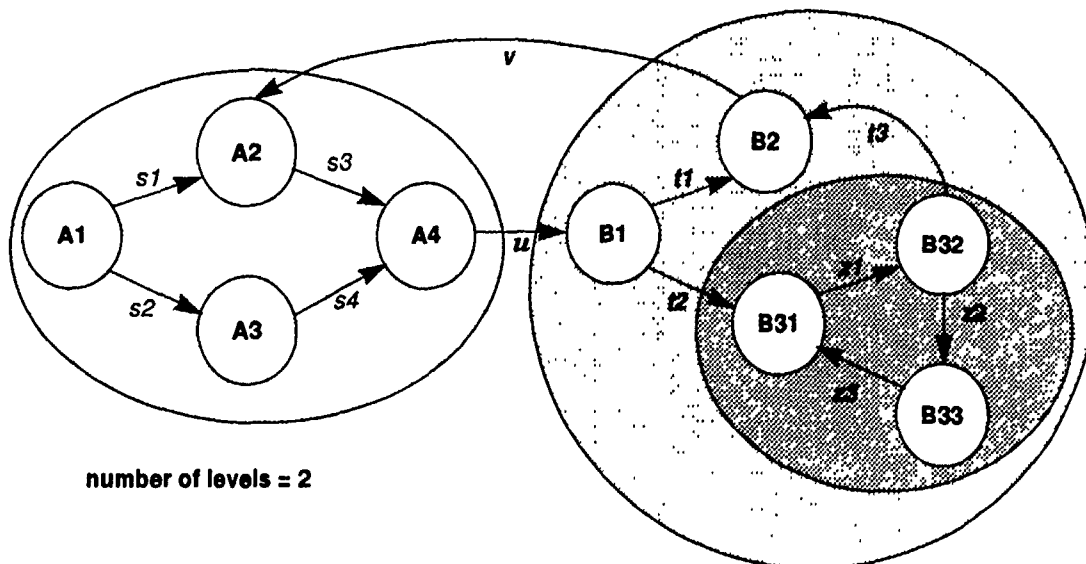
Figure 3.16 The expanded graph for Operator Example
