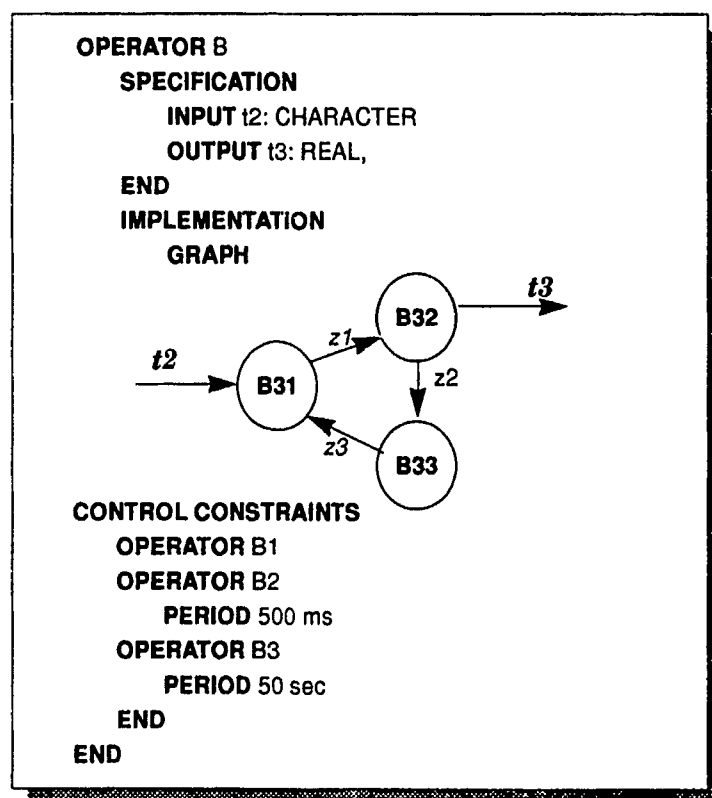
Figure 3.14 PSDL Code for Operator B3
