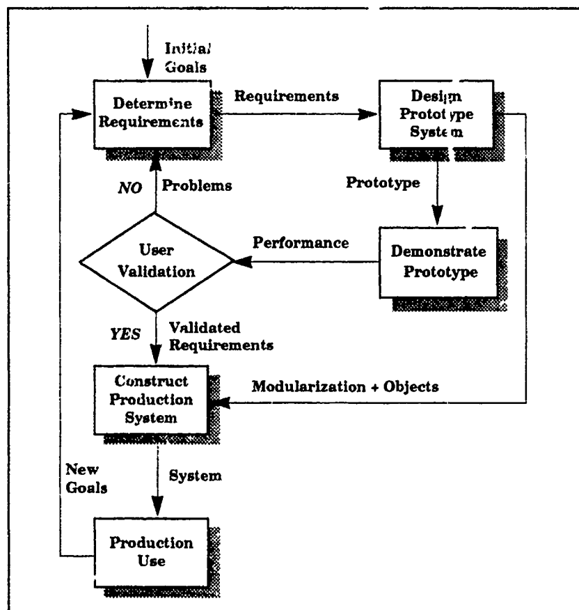
Figure 2.2 Prototyping Life Cycle
