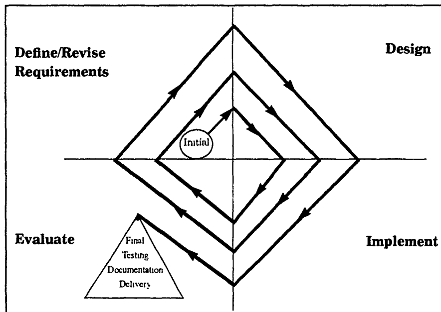
Figure 2.3 Iterative Prototype Development
