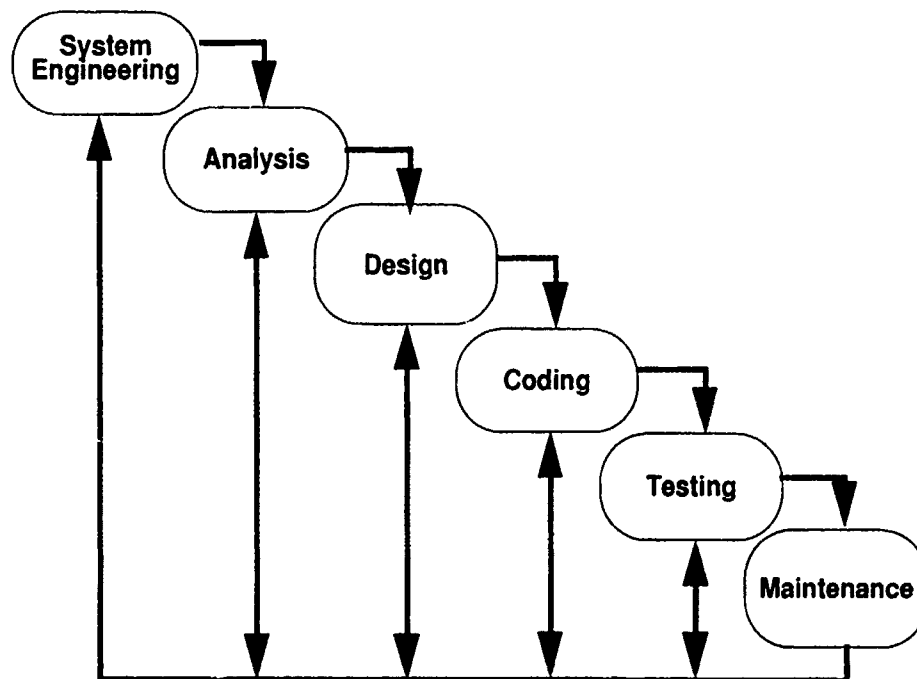
Figure 2.1 The Classic Life Cycle ( Waterfall Model )
