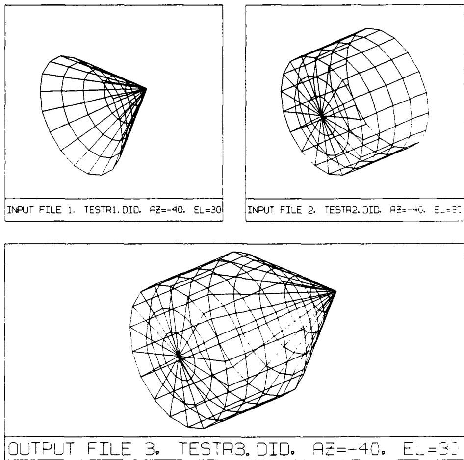
Figure 5-1 Example of an object created by merging and editing simple shapes generated by HEDRON.
