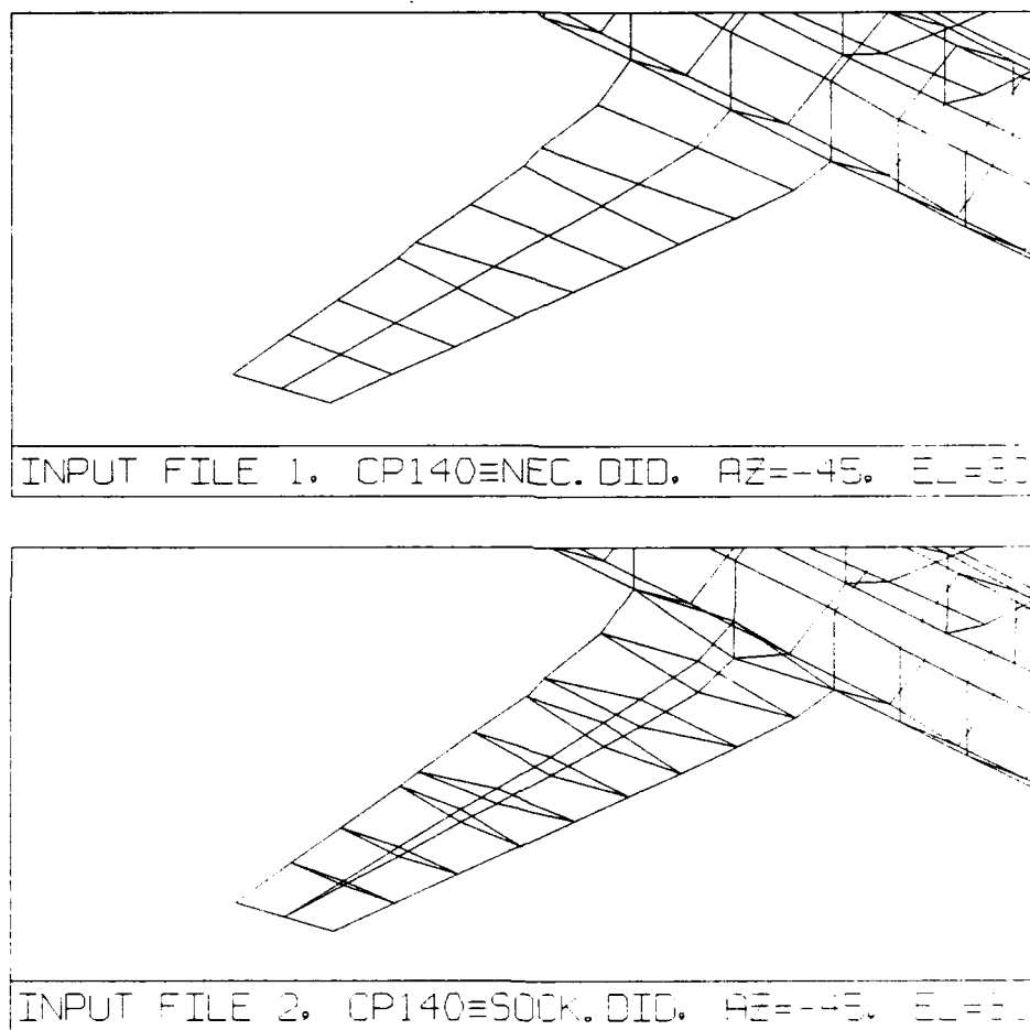
Figure 1-4 Right wing of the CP140 aircraft, before (top) and after (bottom) inflation.
