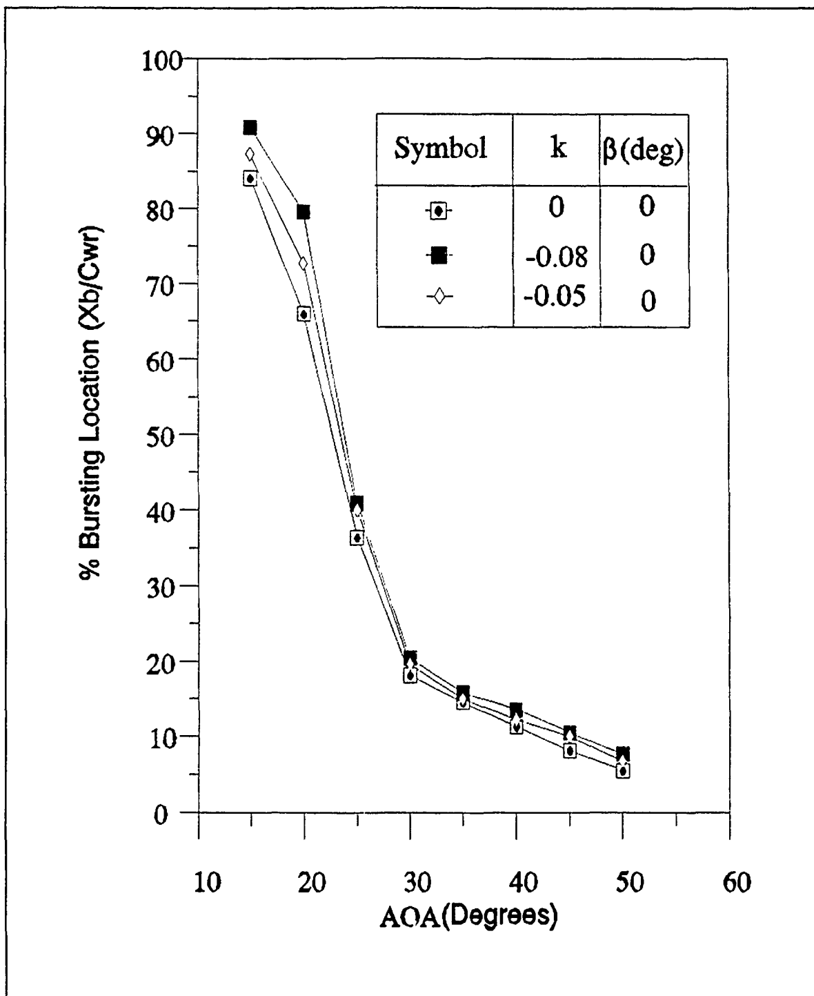
Figure 74. Wing Root Vortex Burst Location at 0° instantaneous Sideslip Angle During Sideslipping Motion, as a Function of AOA
