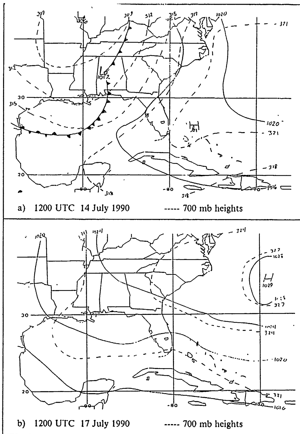
Figure 11. Synoptic pattern in Marathon area (cont.): Surface pressure (mb) and 700 mb heights ( m \cdot 10^{-1} ) from NMC analysis for 1200 UTC is provided for the following days: a) 14 July b) 17 July.
