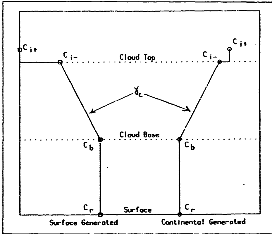
Figure 7. Schematic diagram of aerosol concentration: Dry aerosol concentration based on maritime and continental sources for a weak cumulus convection boundary layer structure. (Gathman, 1989)
