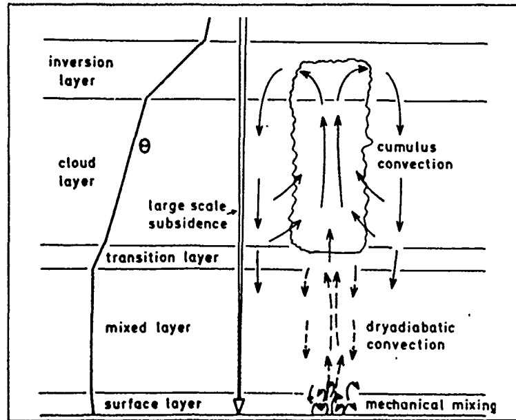
Figure 4. Schematic of dominant processes in a multi-layered MABL: \theta = potential temperature. (Augstein, 1976)
