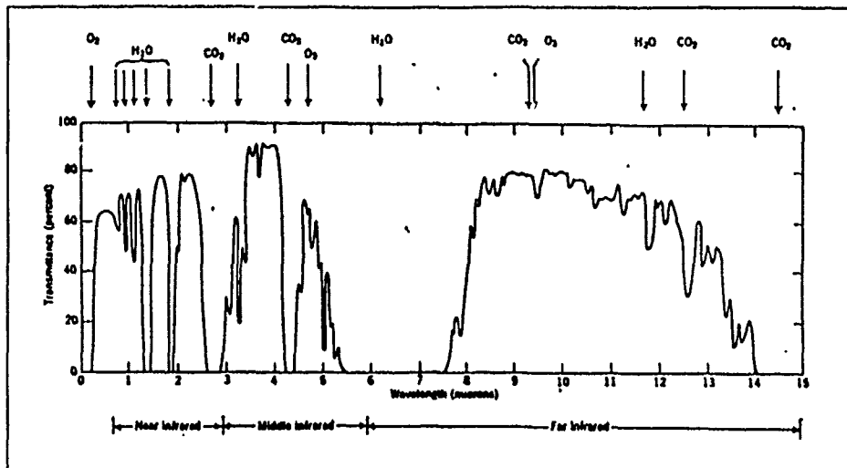
Figure 2. Atmospheric Transmittance (0 - 15 microns): Atmospheric Transmittance measured over a 1.82 km horizontal path at sea level (Hudson, 1969).
