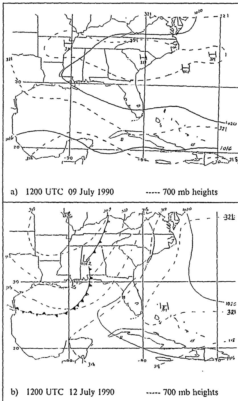
Figure 10. Synoptic pattern in Marathon area: Surface pressure (mb) and 700 mb heights ( m \times 10^{-1} ) from NMC analysis for 1200 UTC is provided for the following days: a) 9 July b) 12 July.
