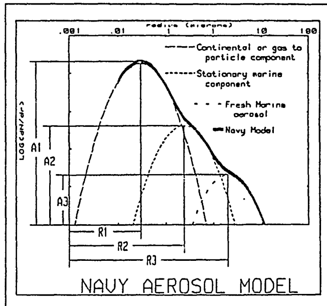
Figure 3. Idealized three lognormal marine aerosol: (Gathman, 1983).
