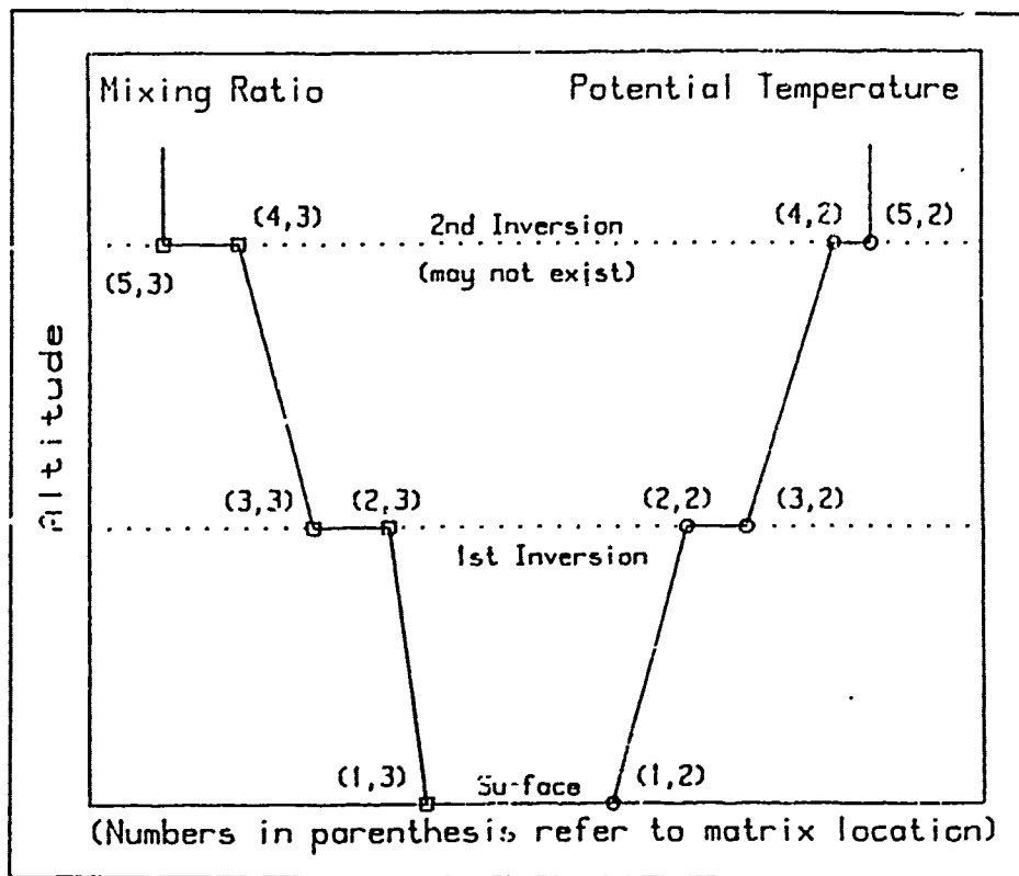
Figure 5. Stylized profile definitions for use in preamble: (Gathman, 1989).
