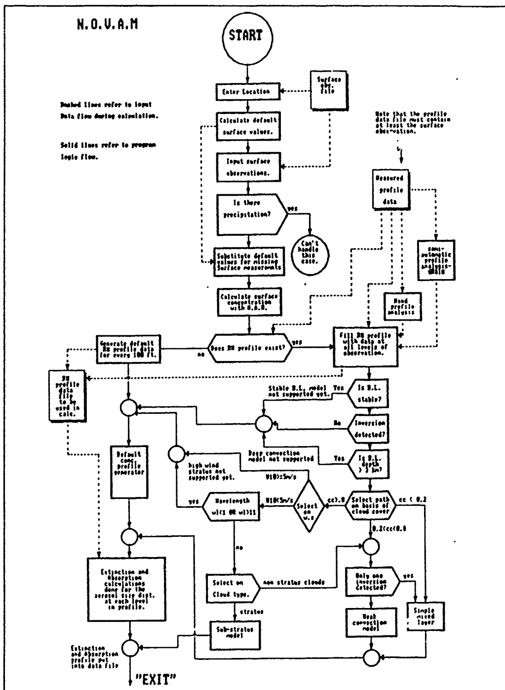
Figure 6. NOVAM flow diagram: (Gathman, 1989).
