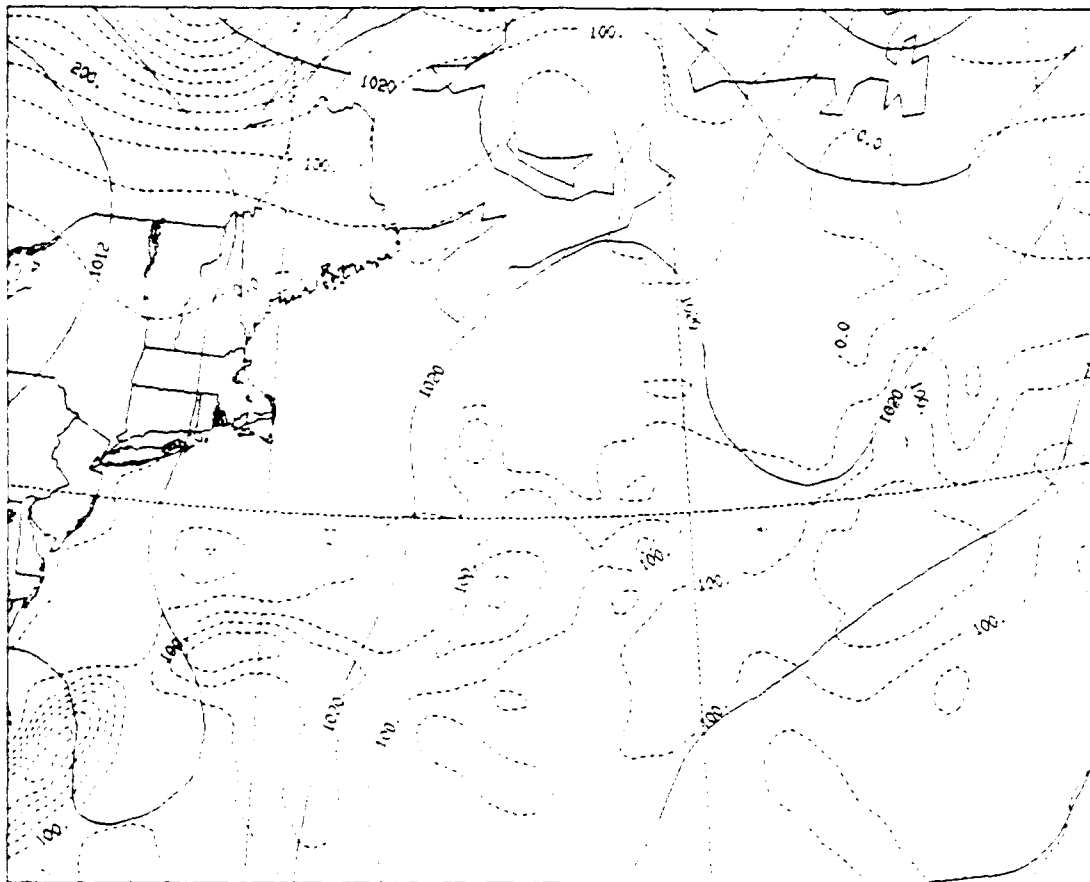
Fig. 17. Sensible Surface Heat Fluxes at 19/0000 UTC January 1989: Same as Fig. 15.
