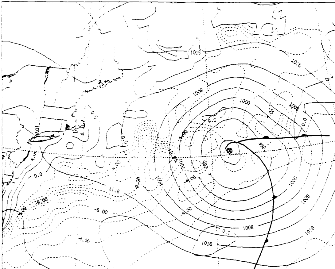
Fig. 23. Air-Sea Temperature Differences at 19/2100 UTC January 1989: Contour interval is 2^{\circ} C. Negative values indicate sea temperature is warmer than air temperature.
