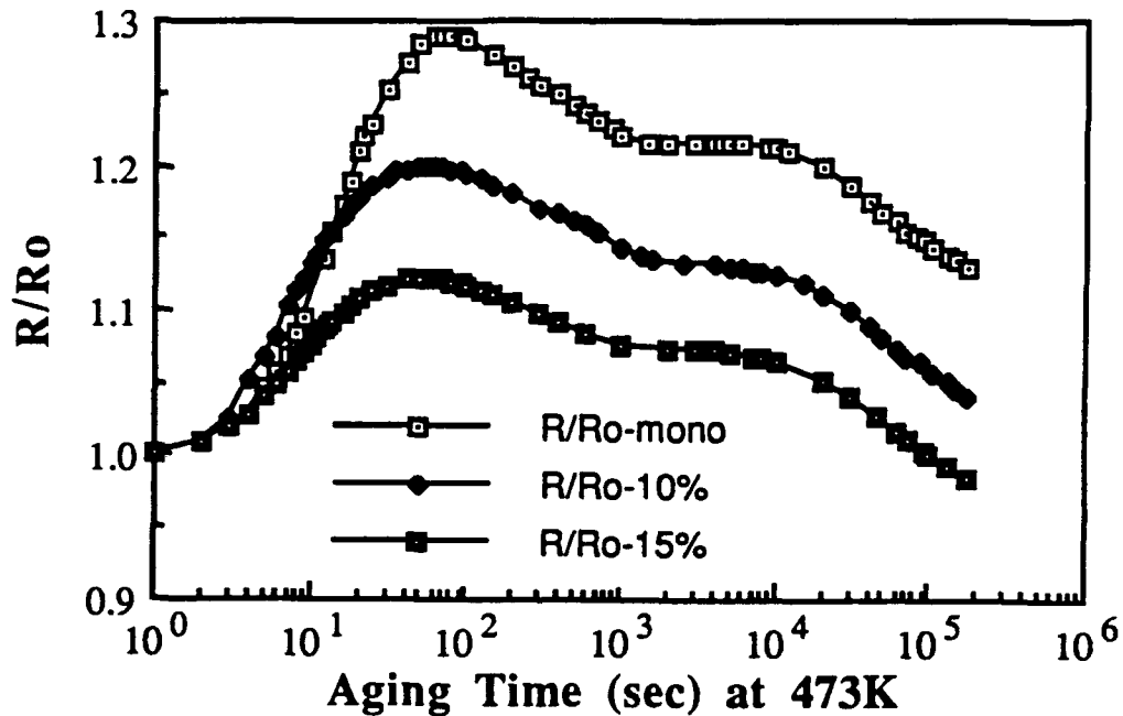
Figure 13: Changes in resistivity of 2014 Al alloy reinforced with 0, 10, and 15 vol% \text{Al}_2\text{O}_3 as a function of time at aging temperature.
