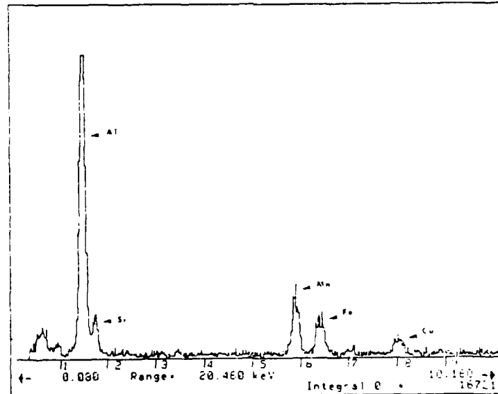
Figure 5b: EDX spectral analysis of the large insoluble particles found in the solutionized and quenched microstructure of Figure 5a.
