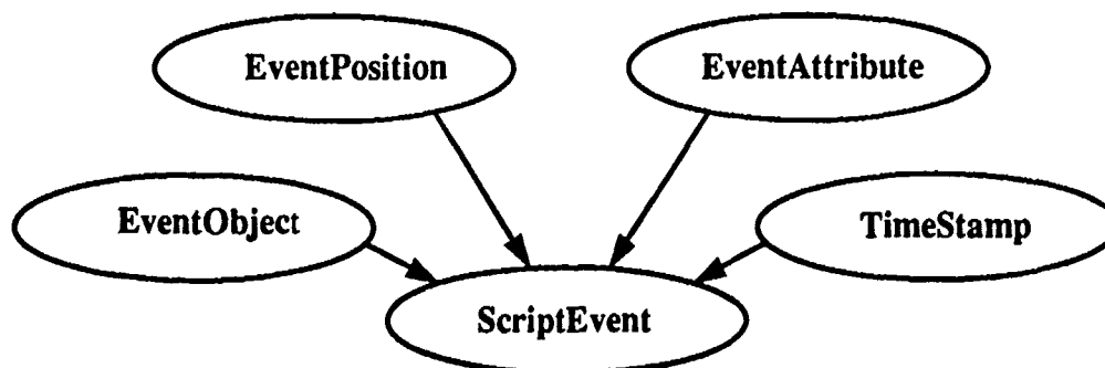
Figure 2.2 Ancestors of Class ScriptEvent
