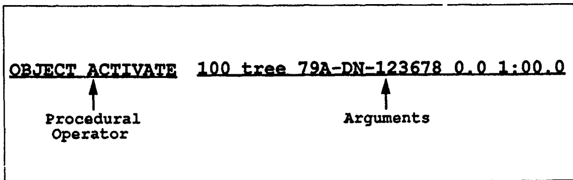
Figure 2.7 General Syntax for Script Statements
