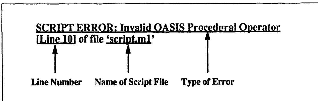
Figure 3.2 Error Message
