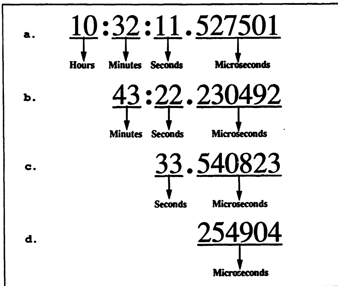
Figure 3.8 Timestamp Formats
