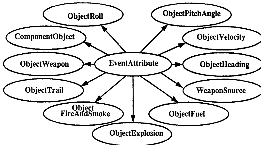
Figure 2.3 Descendants of Class EventAttribute
