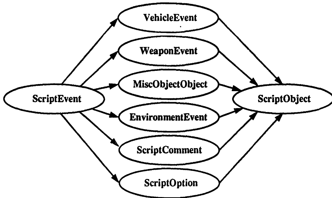
Figure 2.4 Ancestors of Class ScriptObject
