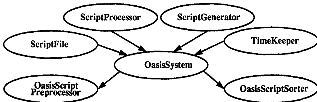
Figure 2.5 Ancestors and Descendants of Class OasisSystem
