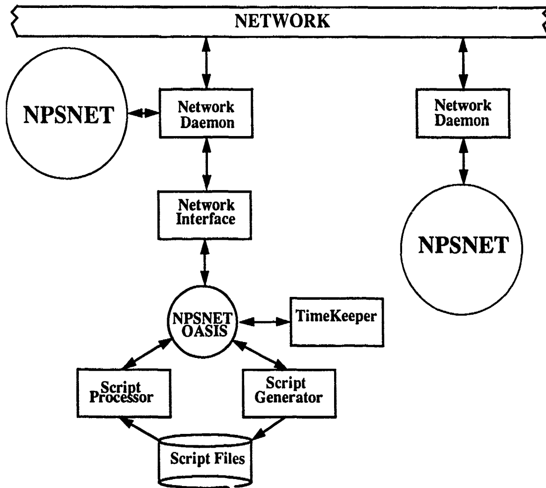
Figure 4.1 NPSNET-OASIS Network Interface
