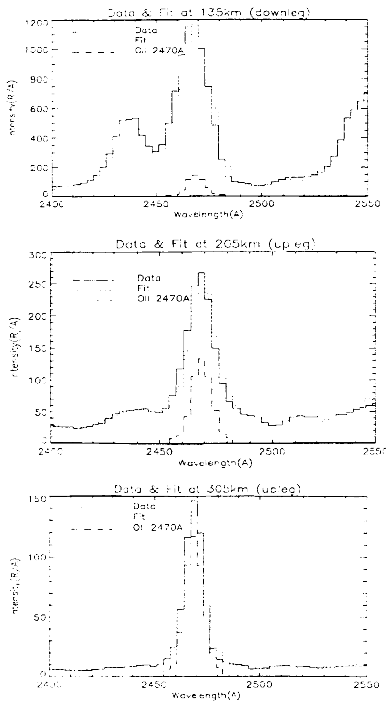
Figure 5-8 Data & fit of OII 2470Å emission at 135, 205, 305km.
