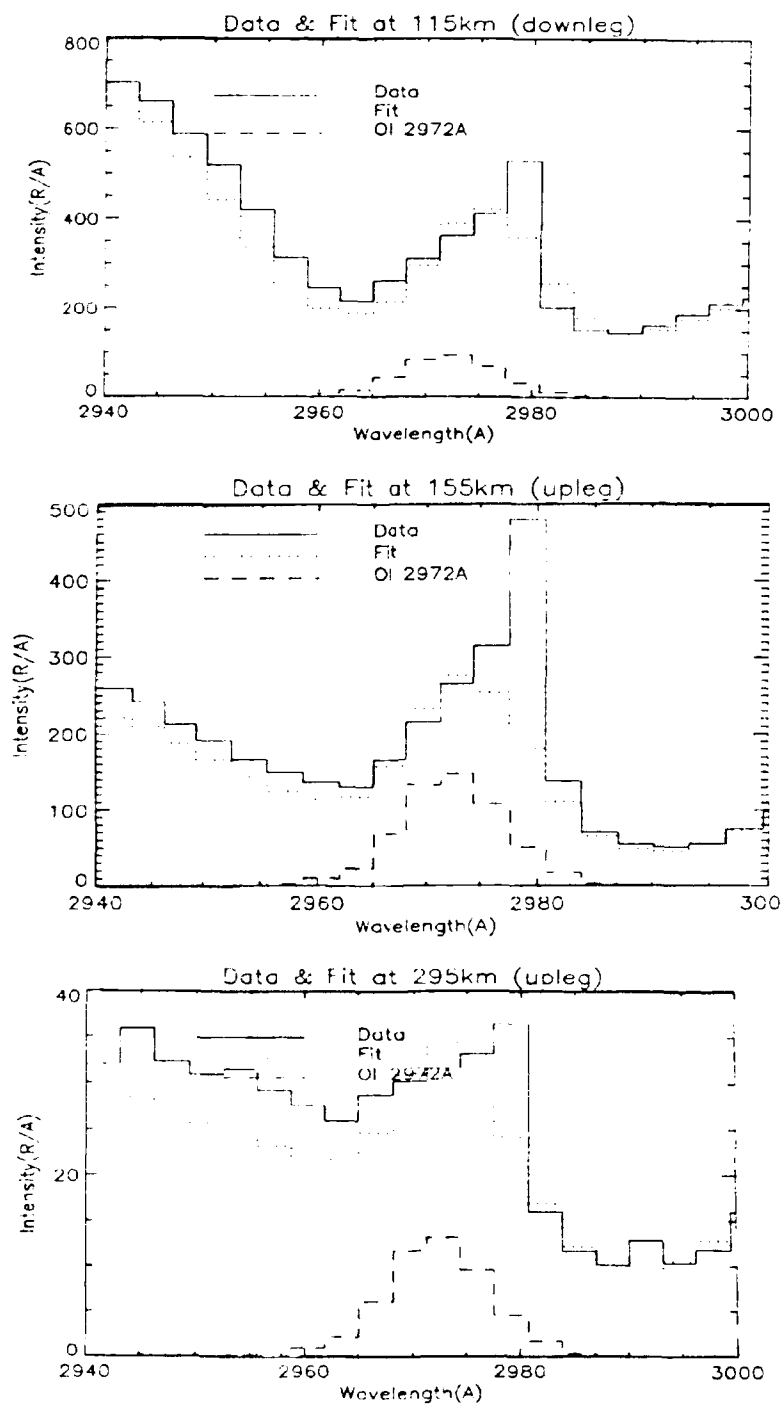
Figure 5-7 Data & fit of OI 2972A emission at 115, 155, 295km.
