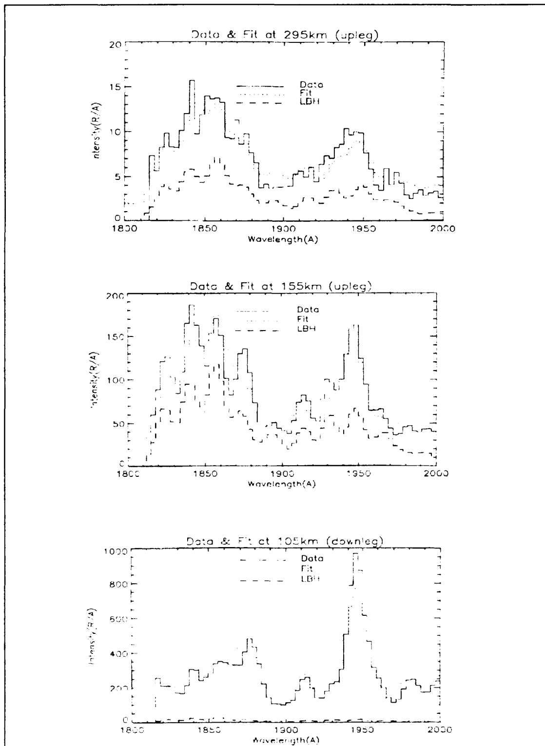
Figure 5-5 Comparison of data & LBH synthetic spectrum for 295, 155, 105km.
