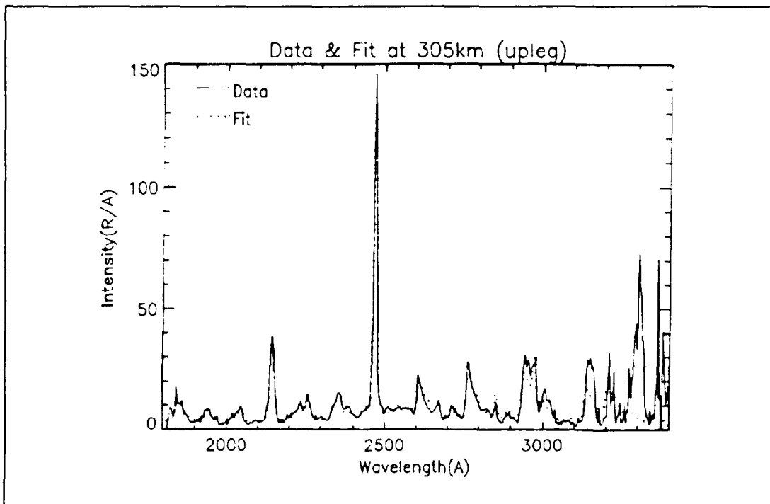
Figure 5-15 Data and best-fitting synthetic spectrum at 305km.
