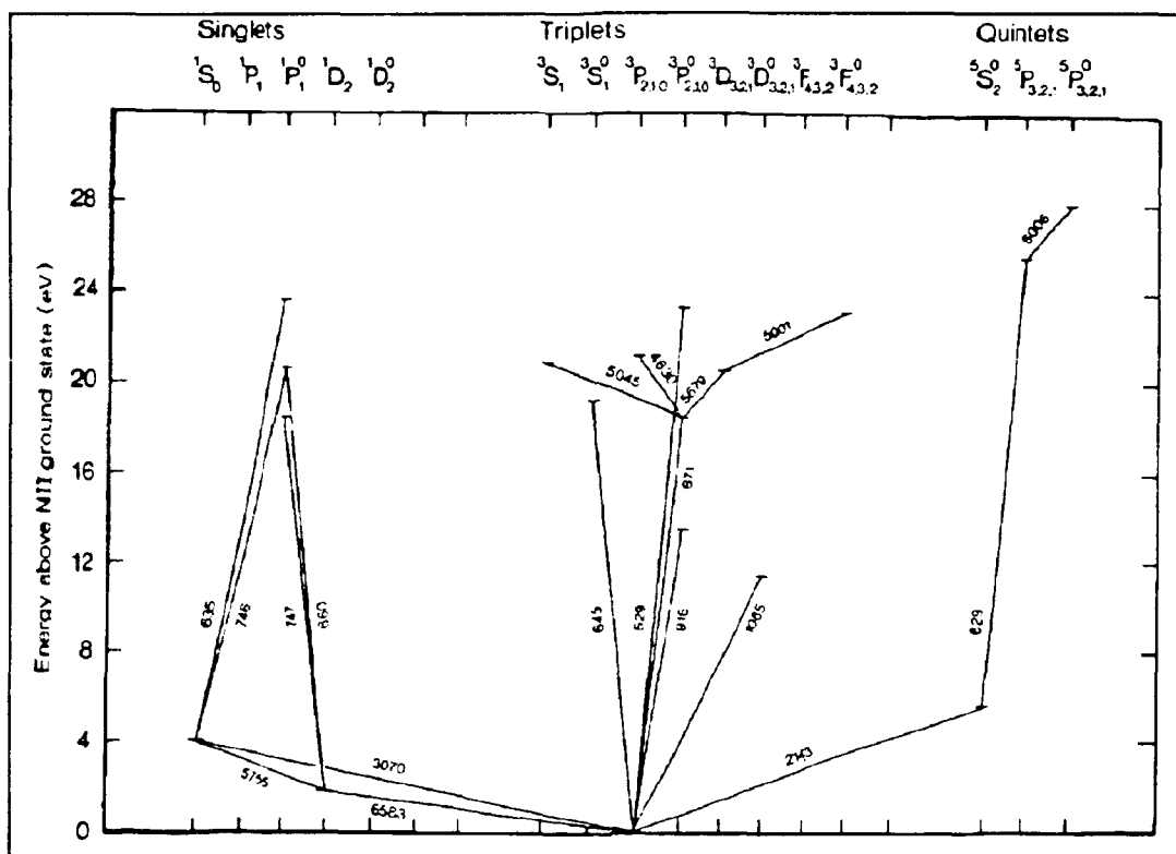
Figure 3-2 Energy level diagram for N^+ (Rees, 1989).
