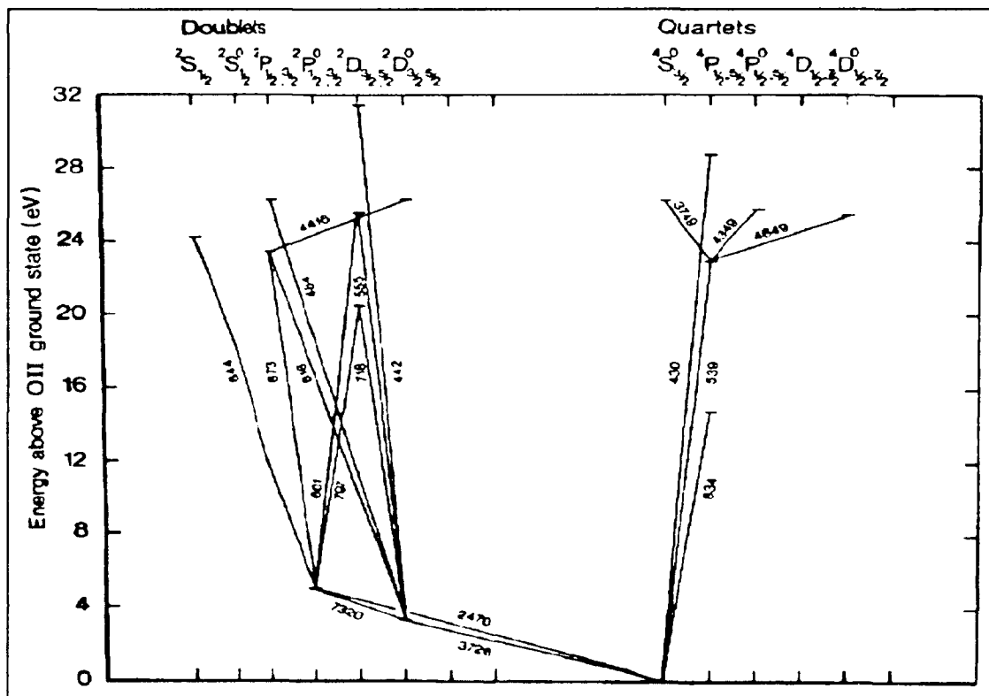
Figure 3-4 Energy level diagram for O^+ (Rees, 1989).
