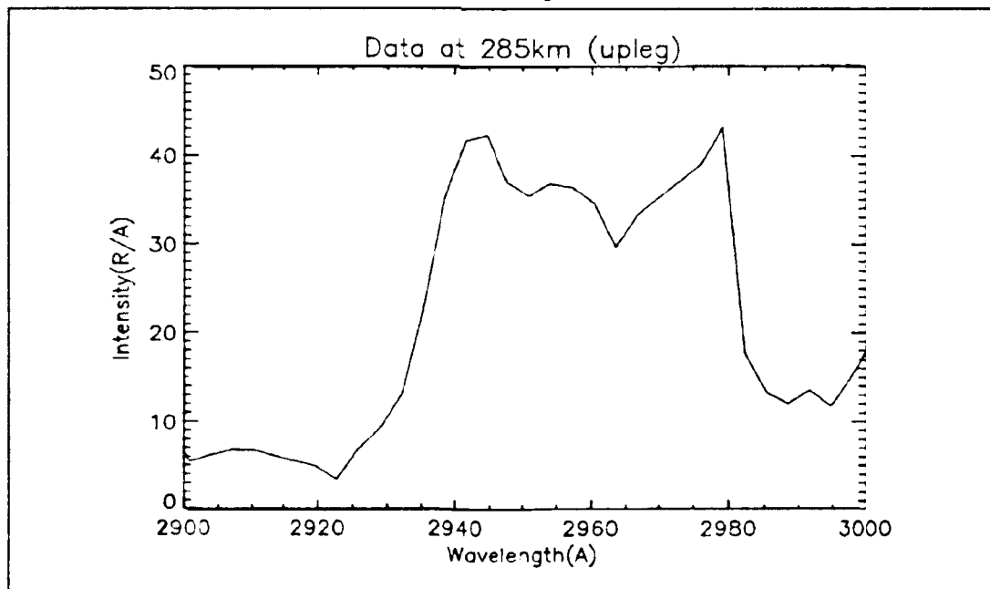
Figure 5-16 Averaged spectrum for 285km. The peak at 2940Å is VK(0,7), the peak at 2980Å is due to OI 2972Å, and the feature at 2955Å is unidentified.
