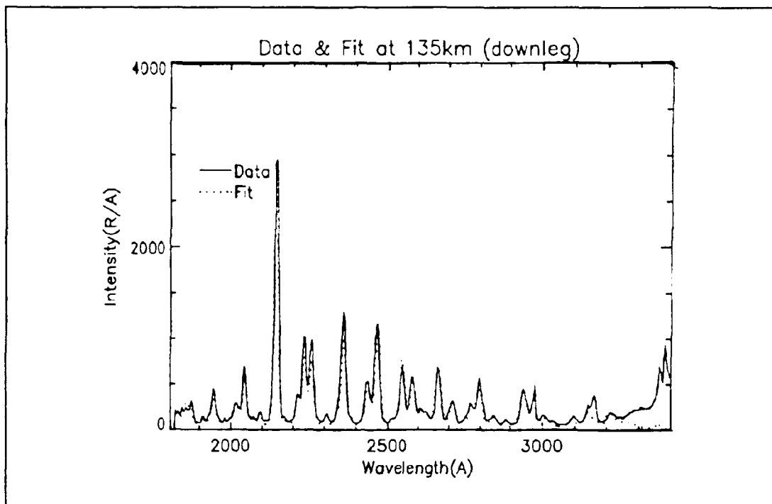
Figure 5-14 Data and best-fitting synthetic spectrum at 135km.
