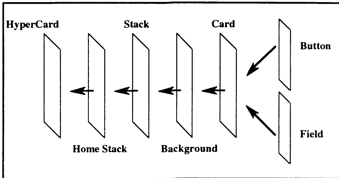
FIGURE 1. OBJECT HIERARCHY [Ref. 1, p. 341]
