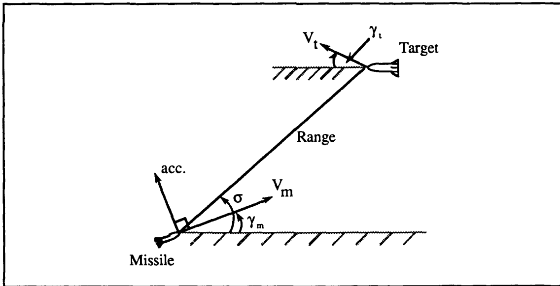
Figure 3.1 Missile/Target Geometry
