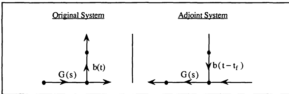
Figure 5.3 Converting Nodes to Summing Junctions
