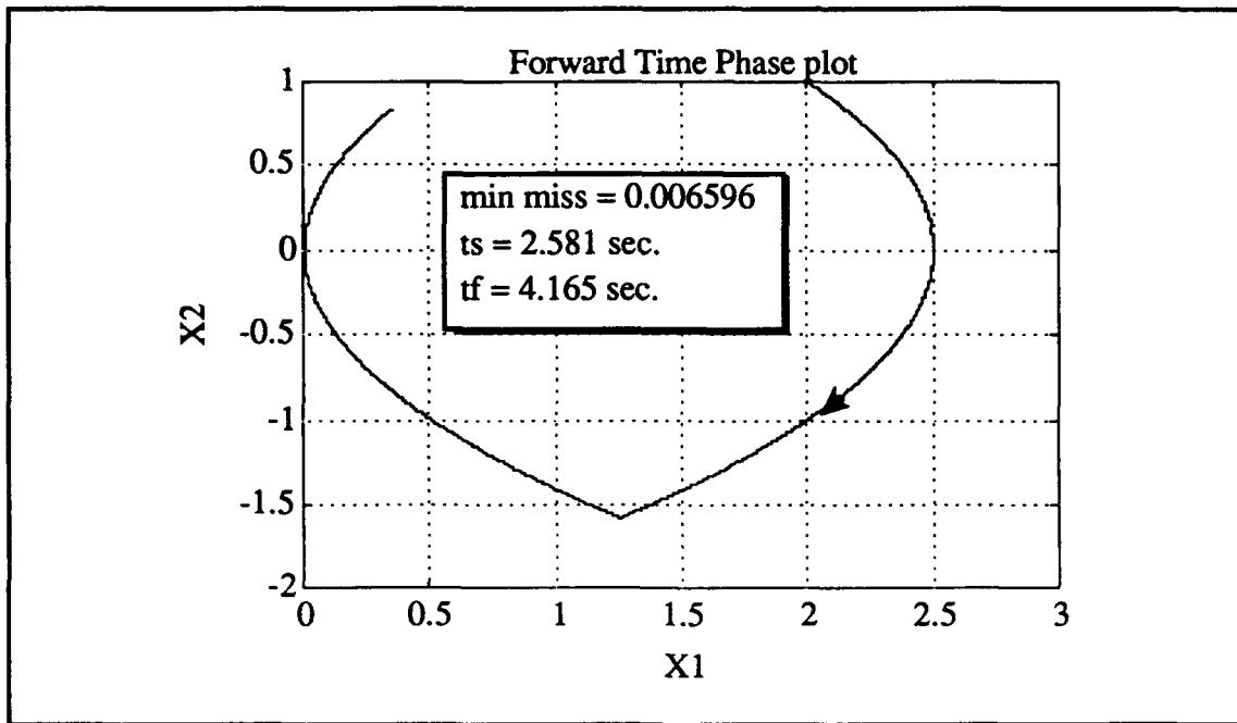
Figure 5.7 Simulation of Forward Time System
