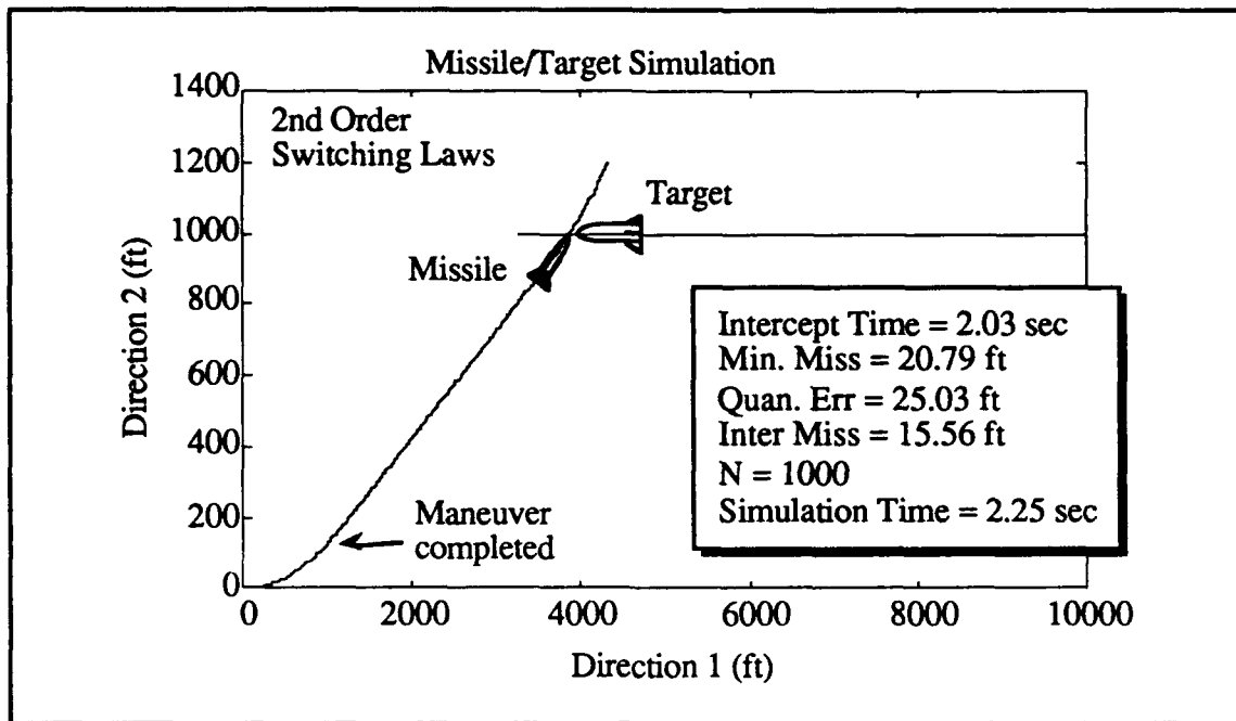
Figure 3.4 Missile/Target Intercept Simulation Using Second Order Controller
