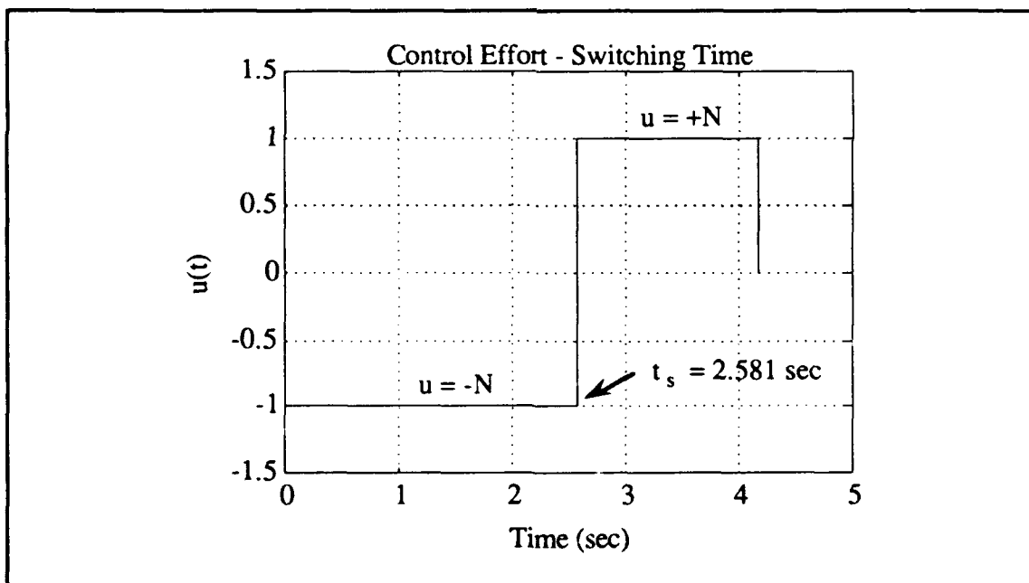
Figure 2.10 Control Effort for Analytic Switching Time Simulation
