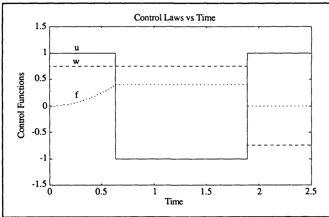
Figure 4.5 Control Laws For Third Order Solution
