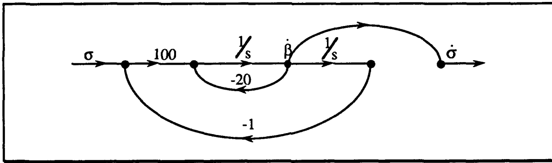
Figure 5.11 Signal Flow Diagram of the Estimator
