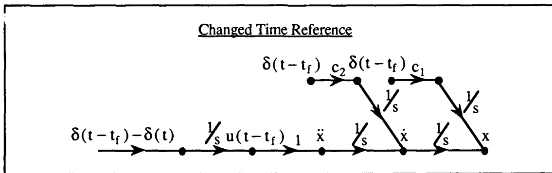
Figure 5.5 Application of Rule 2 on Second Order Example
