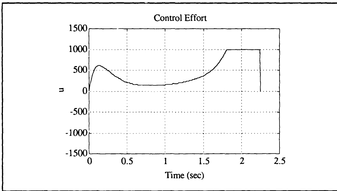
Figure 3.8 Control Effort for Proportional Navigation Missile/Target Simulation
