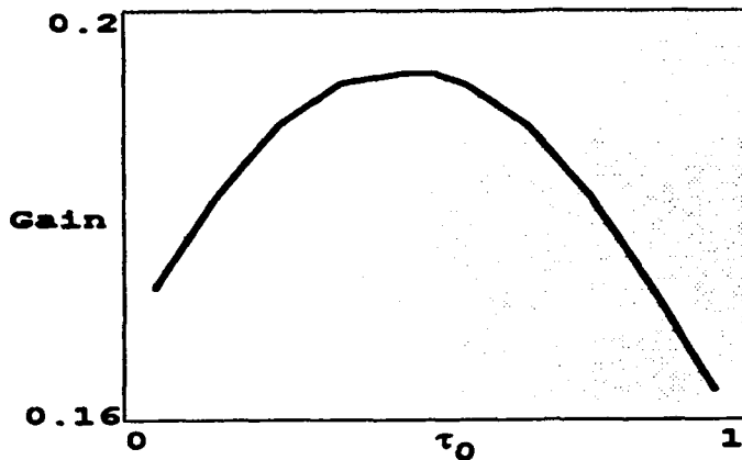
Figure 4-2: Gain versus optical mode waist position for CEBAF UV FEL parameters. Gain peaks at \tau_w \approx 0.45 .
