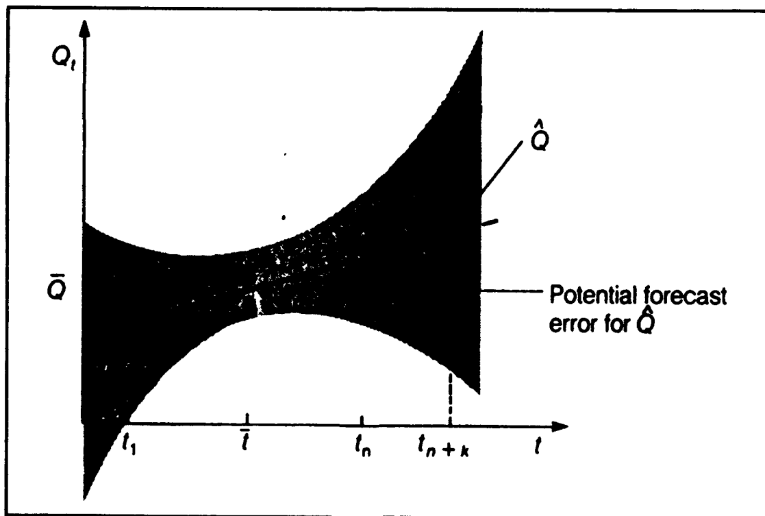
Figure 6: Confidence Intervals
