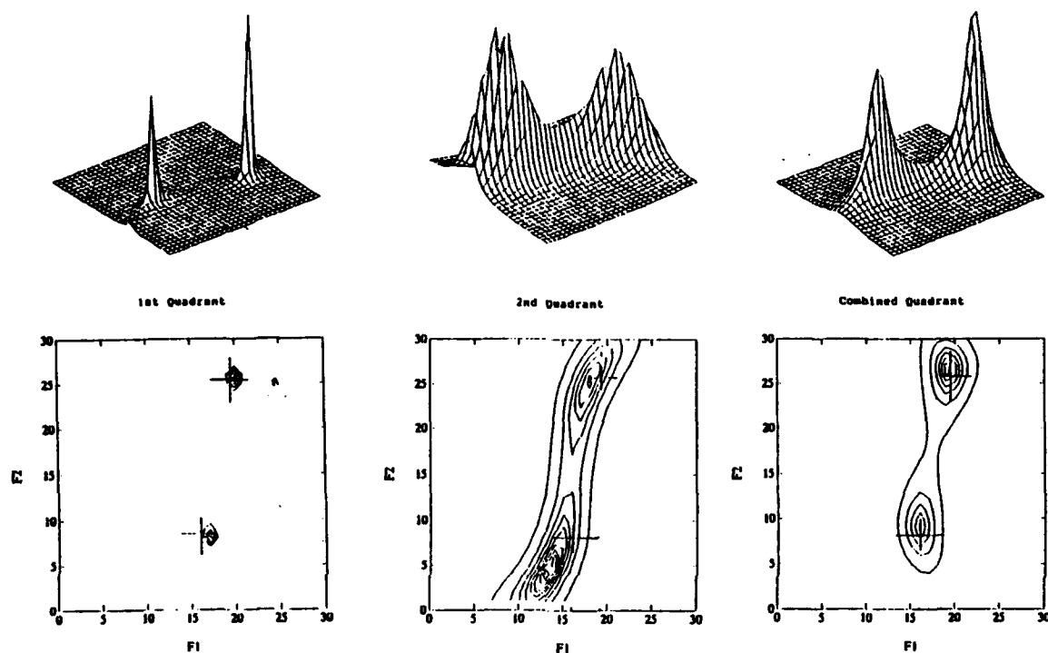
Figure 5.10: 8 \times 8 input array, offset frequencies, (Covariance Method), SNR=10 dB.
