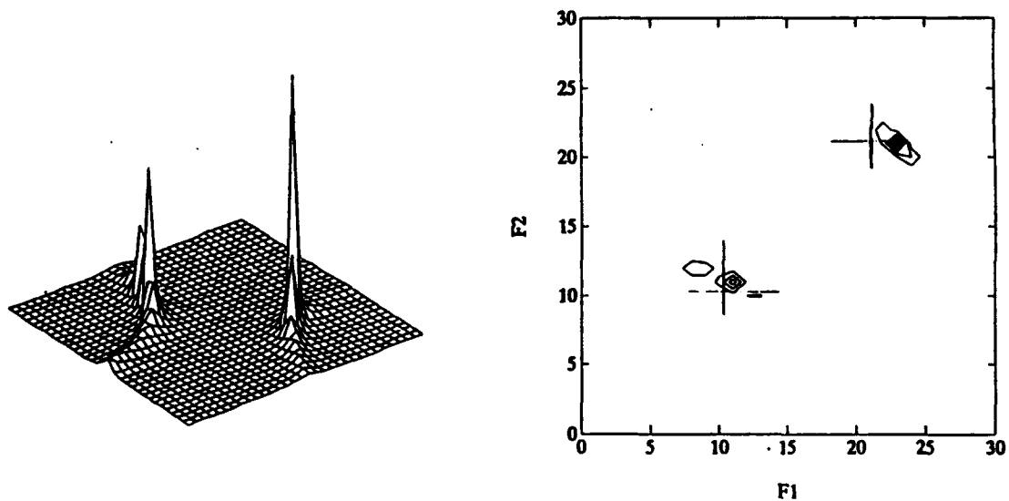
Figure 5.12: 16 \times 16 input array (Covariance Method), SNR=10 dB; non-symmetric half-plane support.
