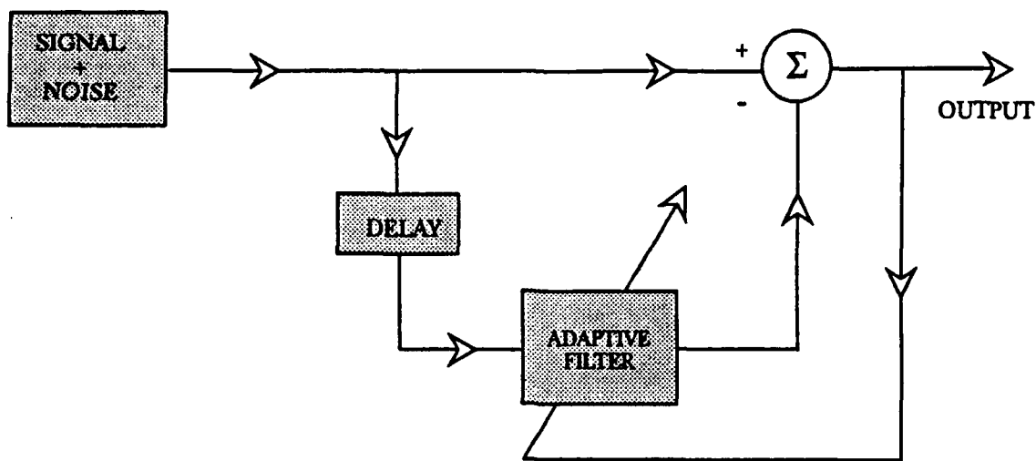
Figure 6.6: The adaptive line enhancer block diagram.
