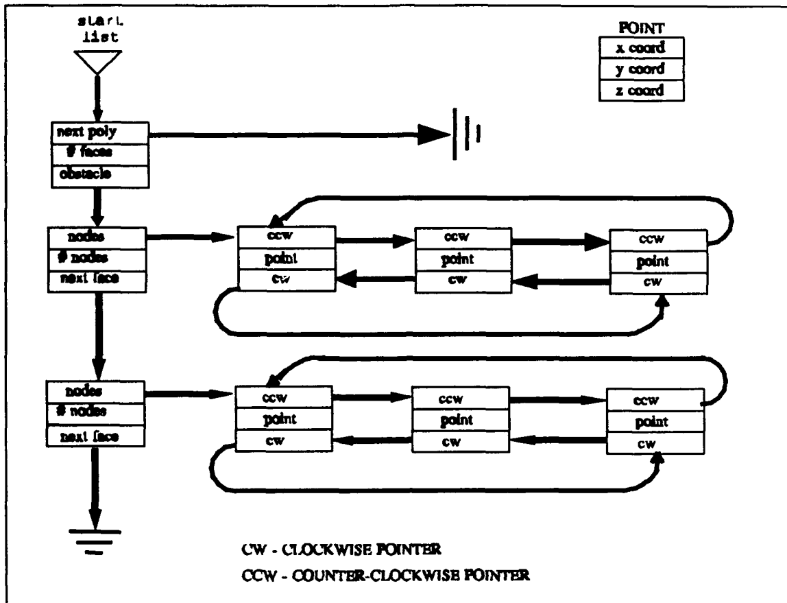
Figure 2 - Polyhedron Link List
