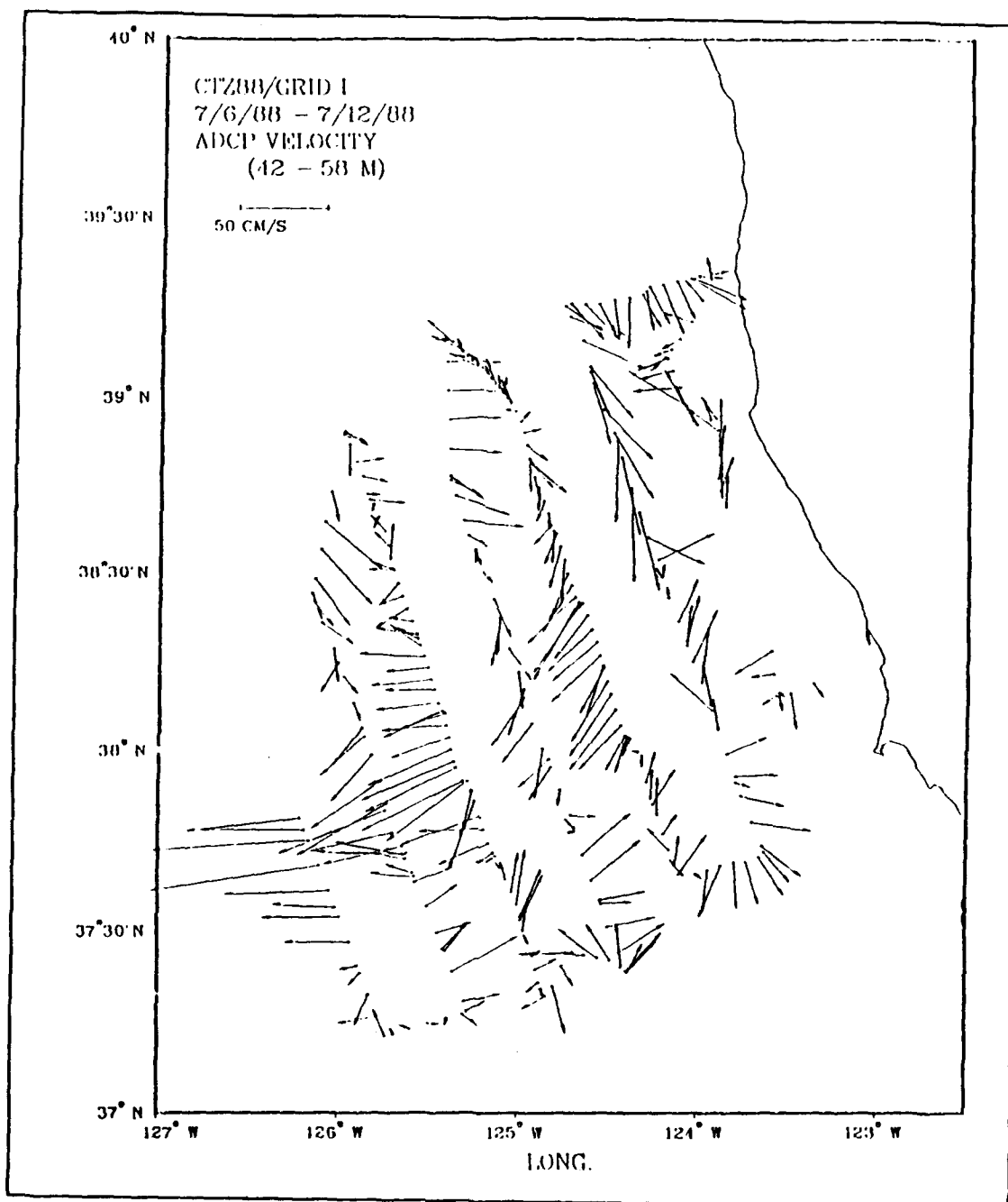
Figure 41. The ADCP Velocity Vector Field at 50 Meters for CTZR1.
