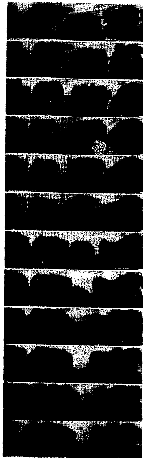
Figure 216. Vortex Pair Collapse Visualization, De=100 , \theta=115^\circ Interval 1/30 s
