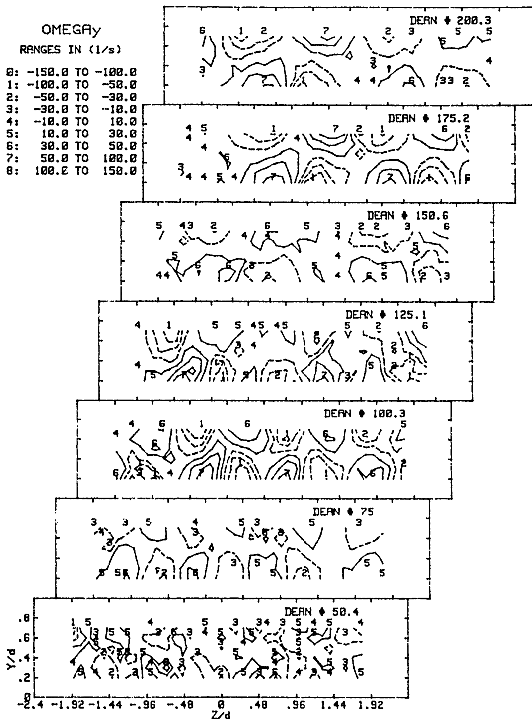
Figure 29. Radial Vorticity Contours De=50.4 to De=200.3
