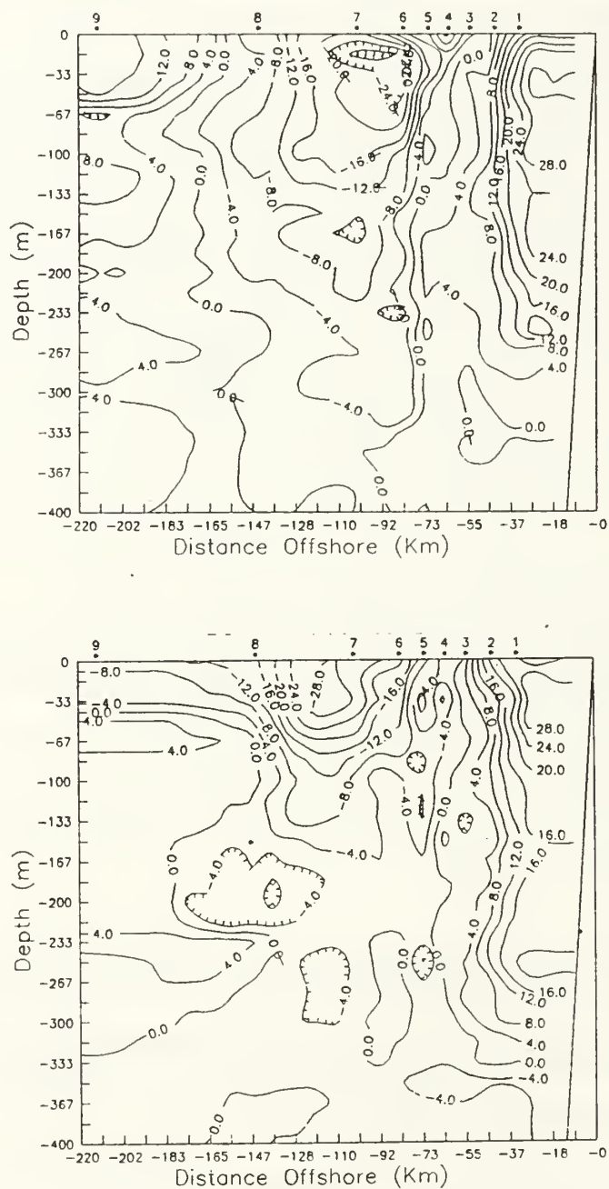
Figure 23. ADCP V Velocities. Top first run. Bottom second run
