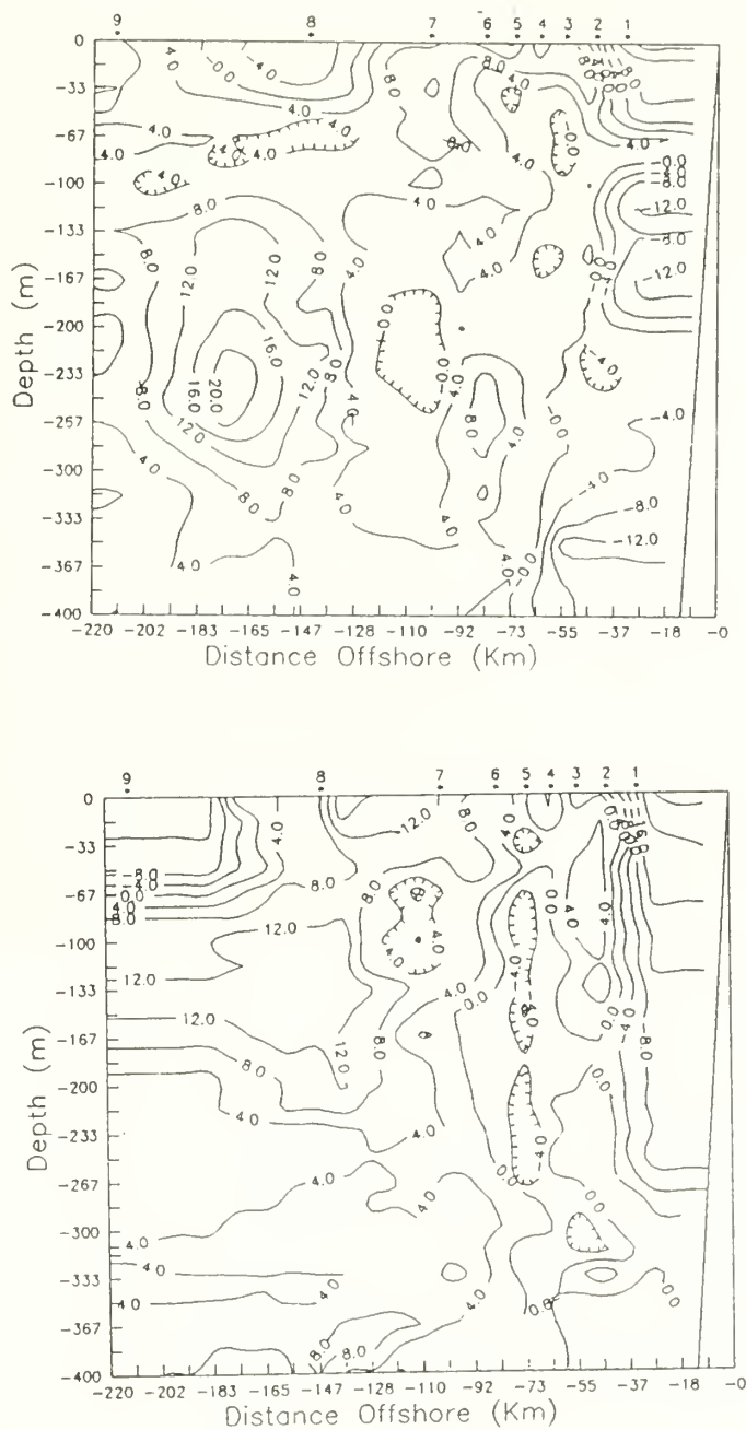
Figure 25. ADCP U Velocities. Top first run. Bottom second run
