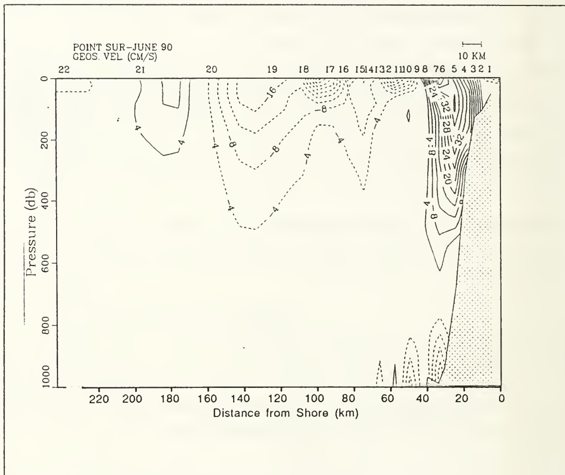
Figure 16. Geostrophic velocities for LNM 700 dbars
