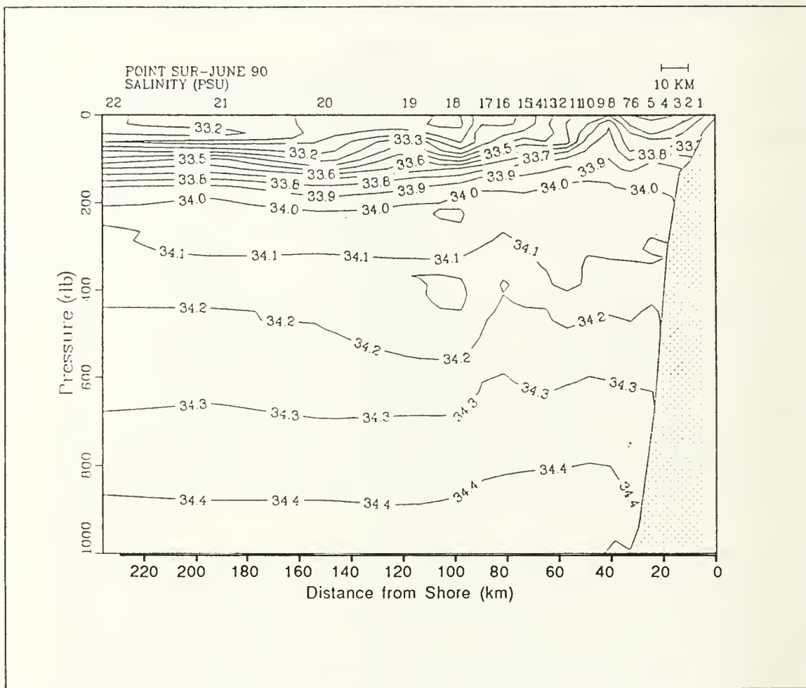
Figure 7. Salinity distribution
