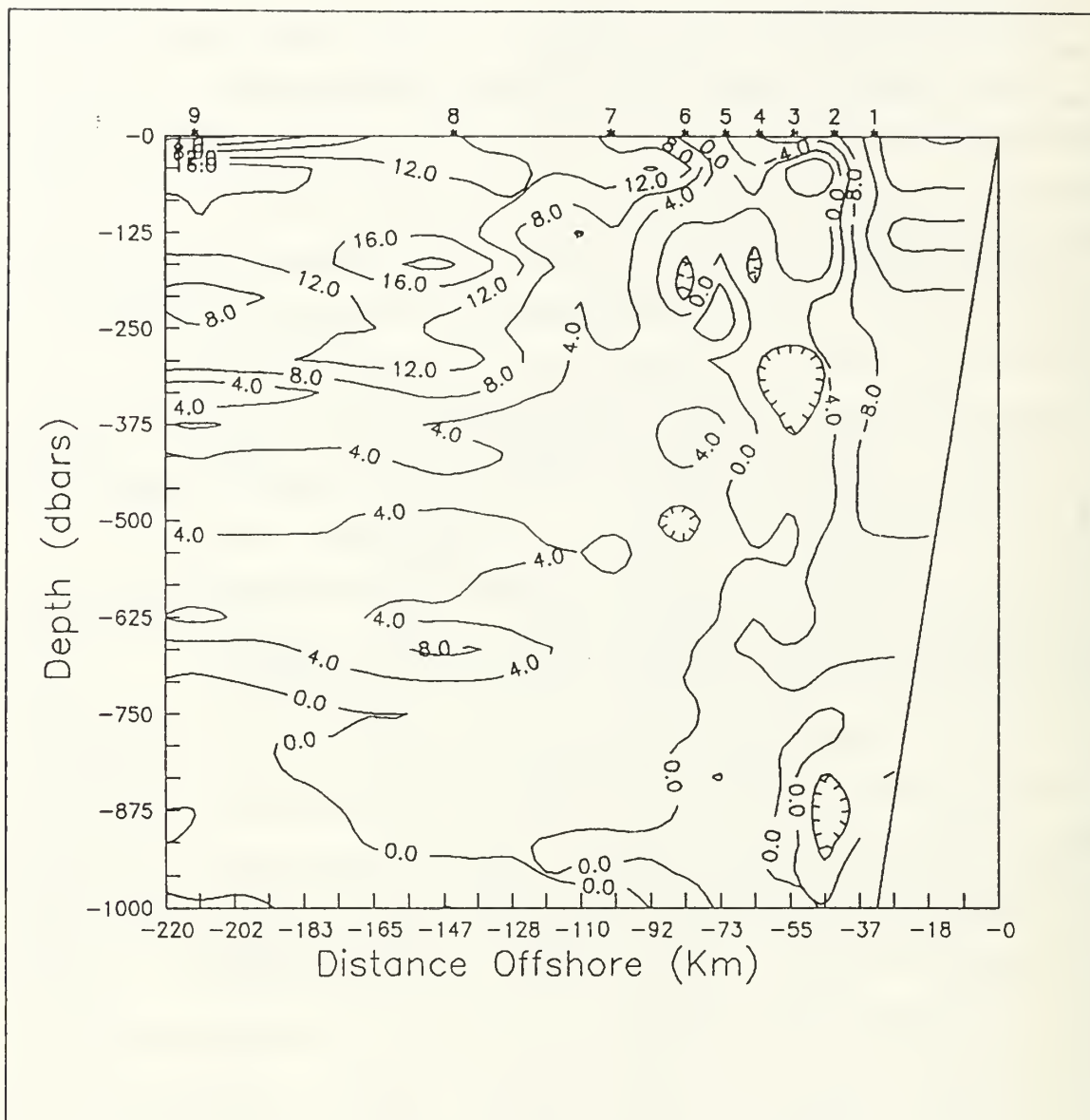
Figure 20. Pegasus U Velocities. Average velocities of the runs
