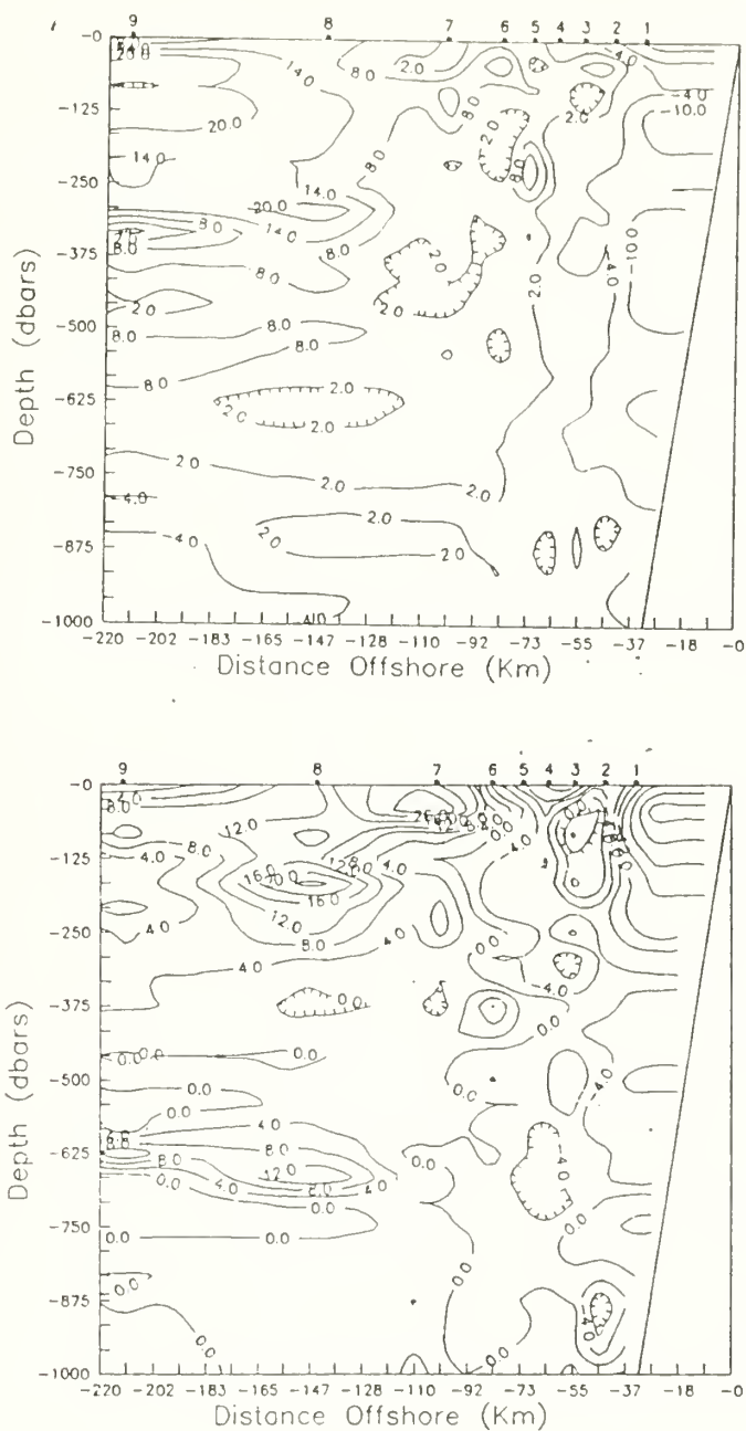
Figure 21. Pegasus U Velocities. Top first run. Bottom second run
