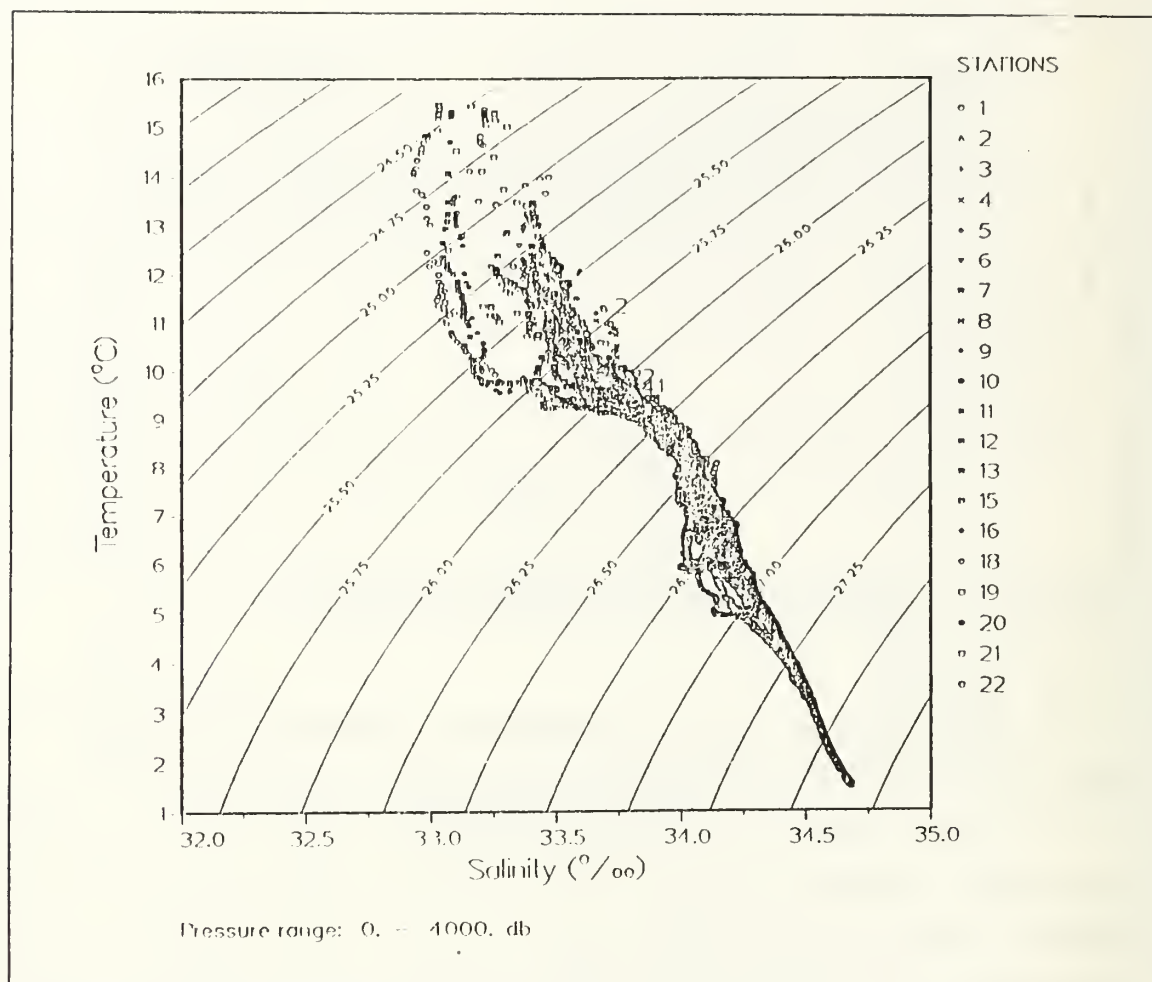
Figure 11. T/S characteristics
