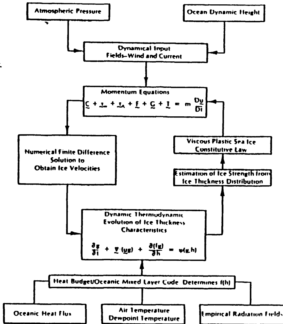
Figure 2.5 A flow chart for the dynamic-thermodynamic ice model. At the top winds and ocean currents are fed into the momentum equation to determine ice velocities. Thermodynamic fluxes are inputted into a heat budget that influences ice thickness along with ice advection. This is sent to an estimation of ice strength which is used to determine the internal ice stress which in turn is used in the momentum balance. In this figure C represents Coriolis force, \tau_w the wind stress, \tau_a the water stress, F the internal ice stress, G ocean currents, and T the surface tilting term, h the ice thickness, and f(h) the growth rate (Hibler, 1979).
