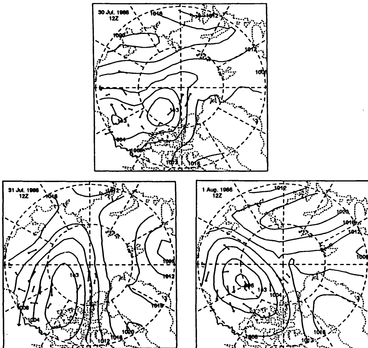
Figure 4.16 Buoy trajectories and buoy derived surface pressure for (c) 30 July, (l) 31 July, and (l) August 1986. For estimation of buoy speed 1 cm equals 23.1 cm/s.
