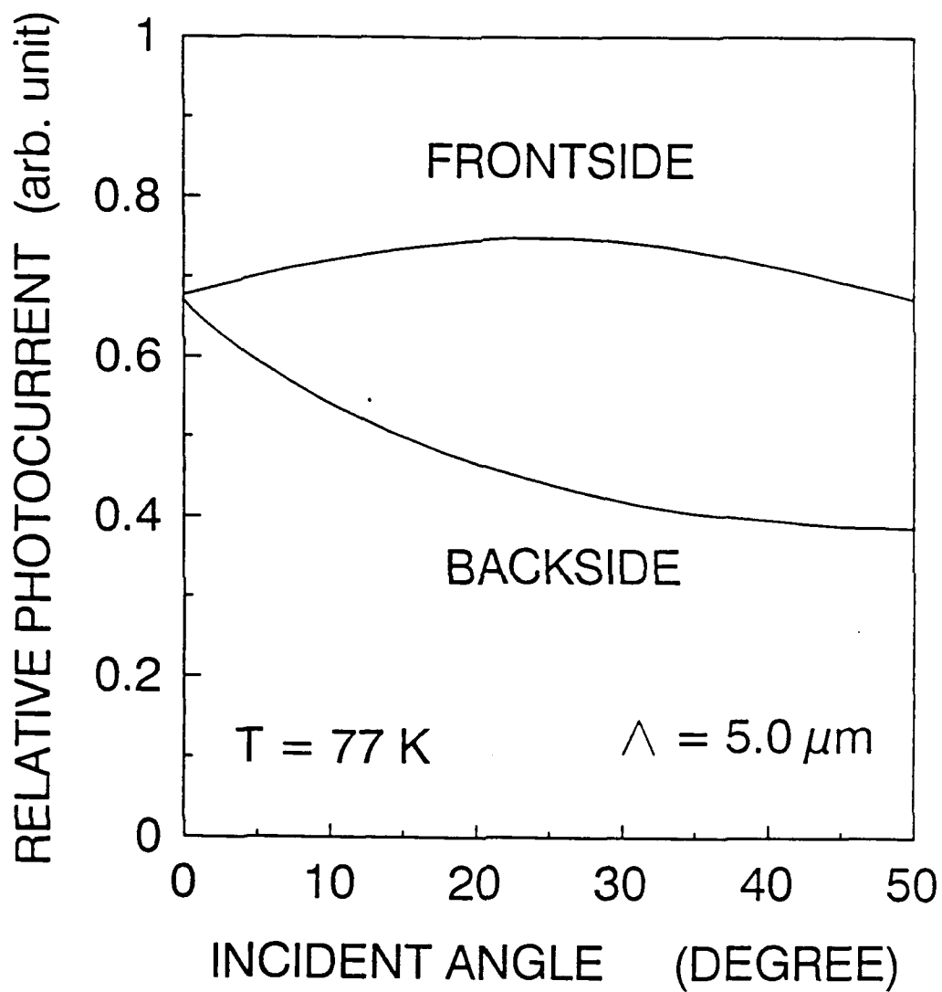
Figure 3.5 Relative photocurrent I_{ph} versus incident angle \theta_i of IR radiations for the front side and backside illumination, using a 5\text{ }\mu\text{m} grating periodicity.
