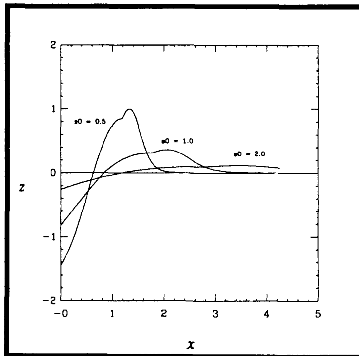
Figure 5-15 Effects of s_0 on \kappa
