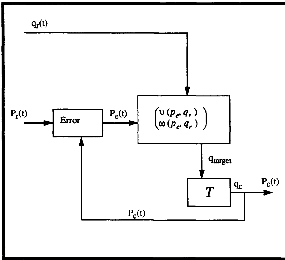
Figure 5-1 Cross Track Guidance Control Loop
