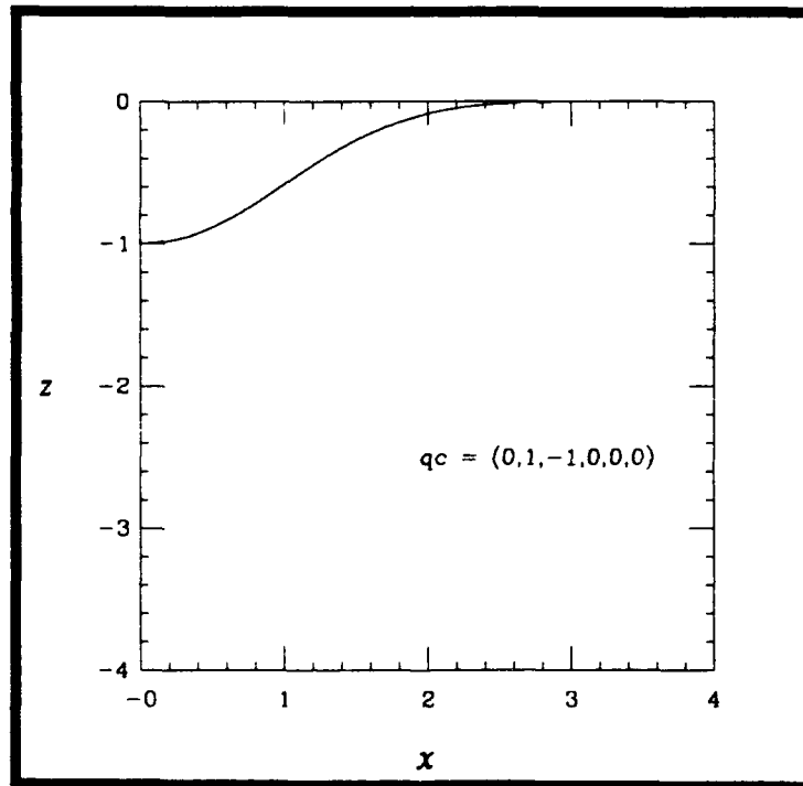
Figure 5-12 Spatial Tracking Convergence (x versus z)
