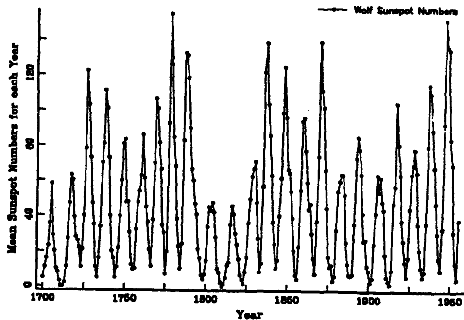
Figure 12. The yearly Wolf sunspot numbers (1700-1955). The data is quite 'periodic' but has nonsymmetric cycles with extremely sharp peaks and troughs. The cycles generally vary between 10 and 12 years with the greater number of sunspots concentrated in each descent period versus the accompanying ascent period.
