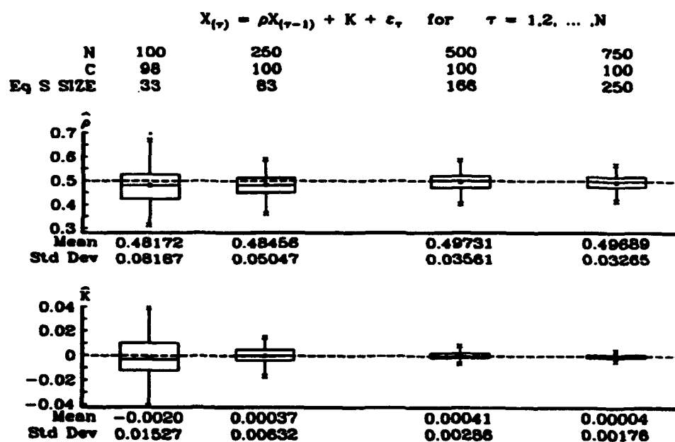
Figure 2. AR(1) MODEL SIMULATION: ASTAR estimates for \rho = .5, K = 0 using \sigma_{\epsilon}^2 = N(0, 1) from C simulations of an AR(1) model for increasing values of N , with P = 1 lag predictor variables, and M = 3 , the number of forward-step subregions permitted in the ASTAR algorithm. Each simulation consists of 100 replications. The boxplots are for the estimates \hat{\rho} and \hat{K} of the model parameters when ASTAR correctly identified the AR(1) model. For N = 100 , 2 simulations were incorrectly identified as constant models.
