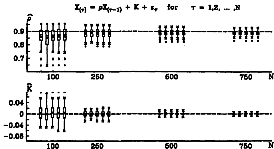
Figure 44. AR(1) MODEL SIMULATION: Boxplots of the estimates from each model selection criterion for \rho = .9, K = 0 when the model selection criterion within MARS correctly identified the data as from an AR(1) model (as reflected in Table 6). For increasing values of N , MARS attempted to identify the AR(1) model (64) from the simulated data using P = 1 lagged predictor variables and M = 3 , the maximum number of subregions allowed in the forward-step MARS procedure, with \sigma_{\varepsilon}^2 = N(0, 1) and a minimum span of MS = .02(N) data points between knots. Each simulation consists of 100 replications. The model selection criterion represented by the boxplots are, from left to right and for each value of N ; GCV^* , AIC , PC , SC and AIC2 . The true value of the model coefficients, \rho = .9 and K = 0 , are identified by the dashed line across each of the boxplots.
