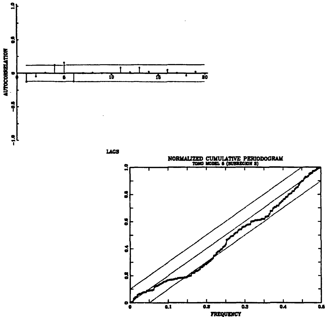
Figure 26. Fitted Residual Plots from Tong Model 5. The autocorrelation function (first 20 lags) and the normalized cumulative periodogram of the fitted residuals from the second subregion, -2 < Z_t < 2 , of Tong Model 5 from Tong et al. (1985) of the Vatnsdalsa River system for the period 1972-1974. If the fitted residuals of the model are truly Gaussian white noise then the fitted residuals from each subregion should also be independent. Although the fitted values of the model, Figure 25, appear to capture the overall structure of the riverflow data, the approximate 95% individual confidence bounds show that some short term residual autocorrelation in the second subregion still exists. Also, the cumulative normalized spectrum of the fitted residuals falls outside the 90% K-S bounds for Gaussian white noise indicating that we should reject the hypothesis that the fitted residuals are Gaussian white noise. Note that the results of the fitted residual analysis from the other subregions of Tong Model 5 are similar.
