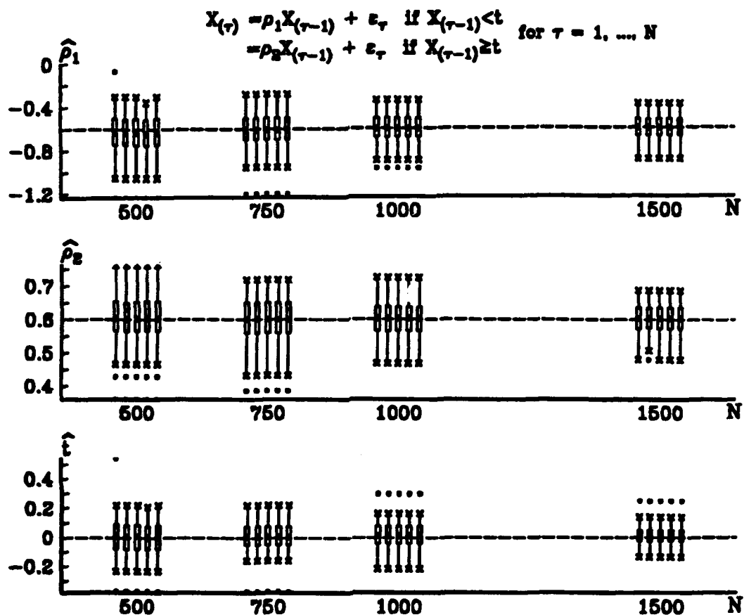
Figure 49. THRESHOLD MODEL SIMULATION: Boxplots of the estimates for \rho_1, \rho_2 = -.6, .6 , and t = 0 when the model selection criterion within MARS correctly identified the data as a threshold model (as reflected in Table 7). For increasing values of N , MARS attempted to identify the threshold model (65) from the simulated data using P = 4 lagged predictor variables and M = 10 , the maximum number of subregions allowed in the forward-step MARS procedure, with \sigma_{\varepsilon}^2 = N(0, .5) and a minimum span of MS = .02(N) data points between knots. Each simulation consists of 100 replications. The model selection criterion represented by the boxplots are, from left to right and for each value of N ; GCV^* , AIC , PC , SC and AIC2 . The true value of the model coefficients, \rho_1 = -.6, \rho_2 = .6 and t = 0 , are identified by the dashed line across each of the boxplots.
