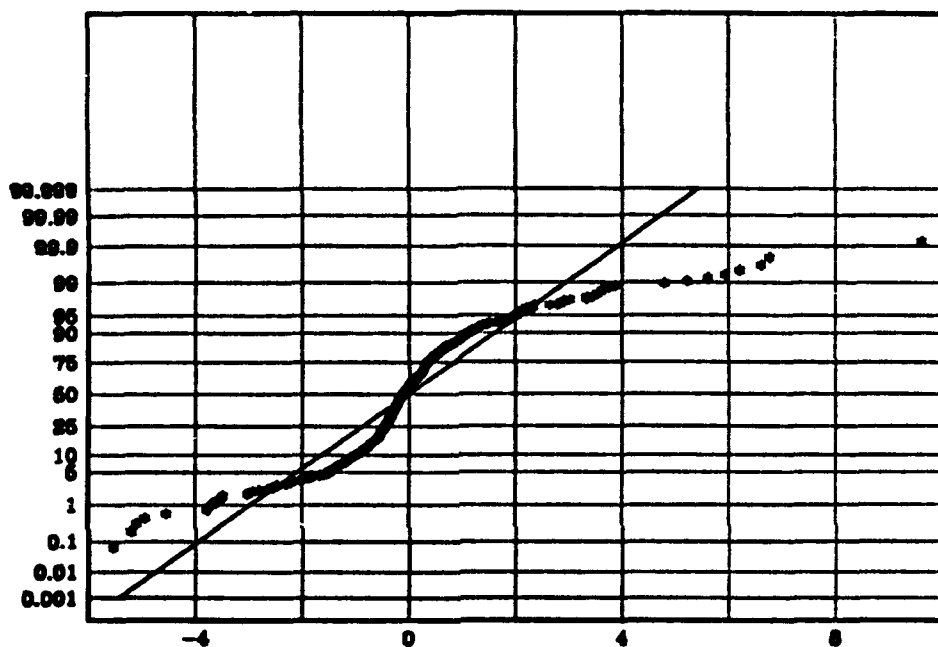
Figure 30. The normal probability plot of the fitted residuals for SMASTAR Model ICE486 of the Vatnsdalsa River system for the period 1972-1974. The horizontal axis shows the range of the fitted residuals from Model ICE486 while the vertical axis shows the corresponding percentiles from the normal distribution. Analysis of this plot shows that the fitted residuals from Model ICE486 are slightly skewed with the extremely heavy tails that we might expect with this type riverflow data. Note that the heavy tails could be an indication of different distributions for the residuals in different regions of the predictor variables.
