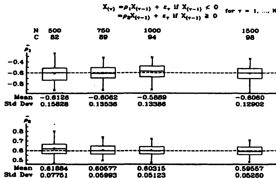
Figure 11. THRESHOLD MODEL SIMULATION: ASTAR estimates for \rho_1, \rho_2 = -.6, .6 using \sigma_\epsilon^2 = N(0, .25) from C simulations of a threshold model for increasing values of N , with P = 4 lag predictor variables, and M = 10 , the number of forward-step subregions permitted in the ASTAR algorithm. Each simulation consists of 100 replications. The boxplots are for the estimates \hat{\rho}_1 and \hat{\rho}_2 of the model parameters when ASTAR correctly identified the threshold models. The models of the simulations that ASTAR did not correctly identify as the threshold model contained an incorrect number of subregions, lacked an AR(1) term in one of the two subregions or contained terms with X_{t-2}, X_{t-3} , or X_{t-4} .
