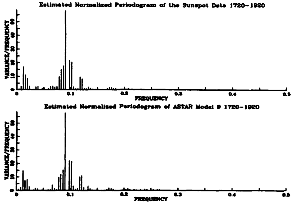
Figure 14. The estimated normalized periodogram of the yearly Wolf sunspot numbers (1720-1920) [top] versus the estimated normalized periodogram of ASTAR Model 9 (1720-1920) [bottom]. The broad conclusion from the top periodogram is that there is a rather diffuse cycle in the data with a period of about 11 years, and a longer period of about 67 years.
