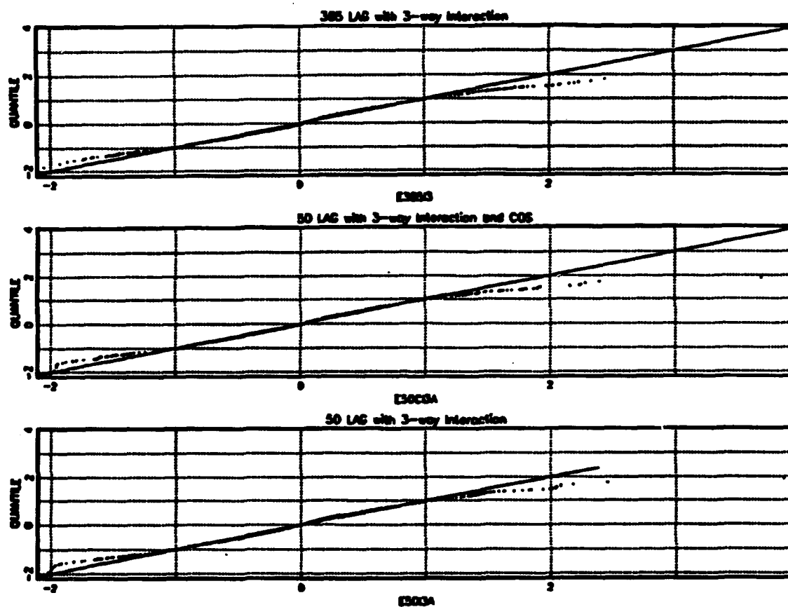
Figure 39. Normal Probability plots of the fitted residuals from 12 years of data (1 March 1971 to 1 March 1980) for three ASTAR time series models of the Granite Canyon sea-surface temperatures. Note that in all three cases the fitted residuals are slightly skewed with heavy tails, thus indicating the nonnormality of the fitted residuals.
