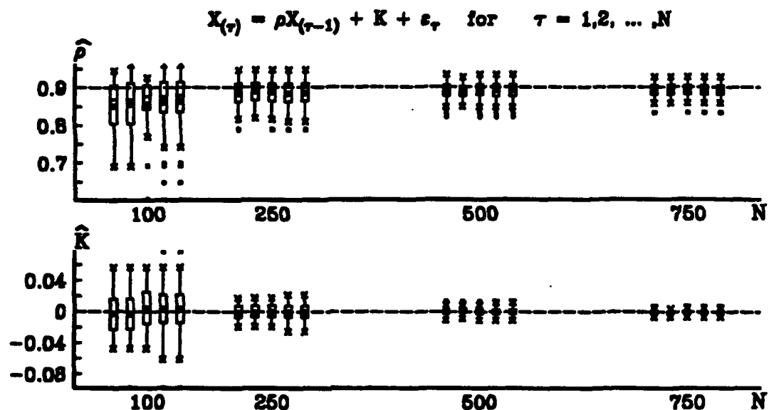
Figure 45. AR(1) MODEL SIMULATION: Boxplots of the estimates from each model selection criterion for \rho = .9, K = 0 when the model selection criterion within MARS correctly identified the data as from an AR(1) model (as reflected in Table 6). For increasing values of N , MARS attempted to identify the AR(1) model (64) from the simulated data using P = 4 lagged predictor variables and M = 8 , the maximum number of subregions allowed in the forward-step MARS procedure, with \sigma_{\varepsilon}^2 = N(0, 1) and a minimum span of MS = .02(N) between knots. Each simulation consists of 100 replications. The model selection criterion represented by the boxplots are, from left to right and for each value of N ; GCV^* , AIC , PC , SC and AIC2 . The true value of the model coefficients, \rho = .9 and K = 0 , are identified by the dashed line across each of the boxplots.
