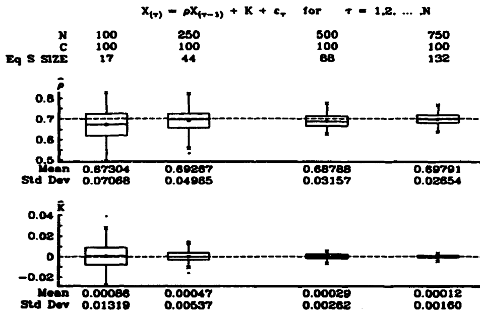
Figure 4. AR(1) MODEL SIMULATION: ASTAR estimates for \rho = .7, K = 0 using \sigma_e^2 = N(0, 1) from C simulations of an AR(1) model for increasing values of N , with P = 1 lag predictor variables, and M = 3 , the number of forward-step subregions permitted in the ASTAR algorithm. Each simulation consists of 100 replications. The box-plots are for the estimates \hat{\rho} and \hat{K} of the model parameters when ASTAR correctly identified the AR(1) model. Here all cases were correctly identified.
