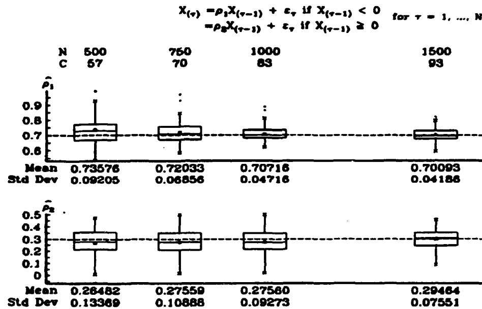
Figure 9. THRESHOLD MODEL SIMULATION: ASTAR estimates for \rho_1, \rho_2 = .7, .3 using \sigma_\varepsilon^2 = N(0, .25) from C simulations of a threshold model for increasing values of N , with P = 4 lag predictor variables, and M = 10 , the number of forward-step subregions permitted in the ASTAR algorithm. Each simulation consists of 100 replications. The boxplots are for the estimates \hat{\rho}_1 and \hat{\rho}_2 of the model parameters when ASTAR correctly identified the threshold model. The models of the simulations that ASTAR did not correctly identify as the threshold model contained an incorrect number of subregions, lacked an AR(1) term in one of the two subregions or contained terms with X_{t-2}, X_{t-3} , or X_{t-4} .
