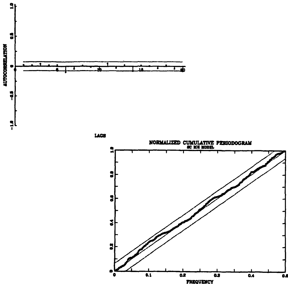
Figure 57. Fitted Residual Plots from SMASTAR Model ICE SC160. The autocorrelation function (first 20 lags) [top] and the normalized cumulative periodogram [bottom] of the fitted residuals from SMASTAR Model ICE SC160 of the Vatnsdalsa River system for the period 1972-1973. The top plot, with approximate 95% individual confidence bounds, shows that no apparent autocorrelation exists in the fitted residuals. Also the K-S bounds in the normalized cumulative periodogram plot indicates no departure from a flat spectrum, so that if the residuals are normally distributed, the residuals are independent.
