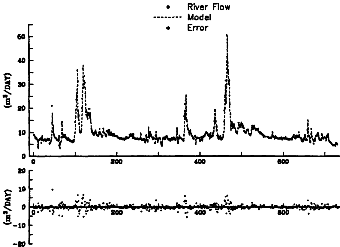
Figure 29. The Vatnsdalsa riverflow data for years 1972 and 1973 versus the fitted values (top) and residuals (bottom) for SMASTAR Model ICE486. The SMASTAR model for the riverflow at time t , X_t , was a function of lagged riverflow X_{t-1} to X_{t-5} , lagged precipitation Y_{t-1}^* to Y_{t-6}^* , i.e., the natural log transformation Y_{t-i}^* = \ln(1 + Y_{t-i}) , lagged temperature Z_{t-1} to Z_{t-6} , and a variable for time of year effect. The final model contains 21 parameters that includes 13 terms with 8 thresholds (1 each on the lagged riverflow predictor variables; X_{t-1}, X_{t-2}, X_{t-4} , the lagged precipitation predictor variables; Y_{t-1}, Y_{t-2} , and the lagged temperature variable, Z_{t-2} and 2 on the lagged temperature variable Z_{t-1} ). The standard error of the fitted residuals \sigma_e was 1.27\text{m}^3/\text{sec} . The initial nine values of each time series were used to initialize the model.
