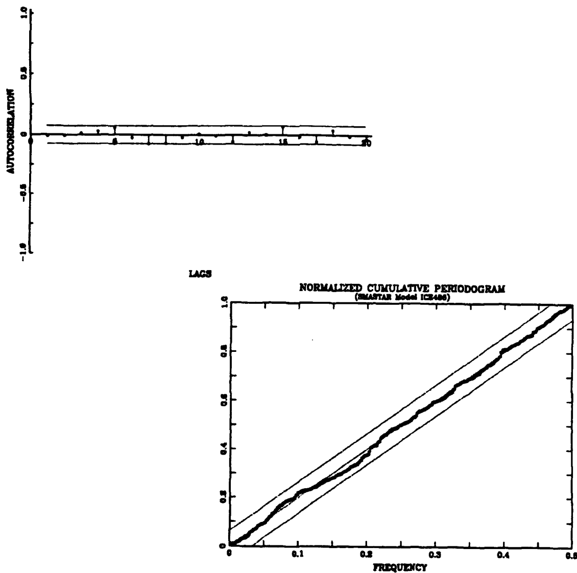
Figure 31. Fitted Residual Plots from SMASTAR Model 486. The autocorrelation function (first 20 lags) [top] and the normalized cumulative periodogram [bottom] of the fitted residuals from SMASTAR Model486 of the Vatnsdalsa River system for the period 1972-1973. The autocorrelation plot with approximate 95% individual confidence bounds shows that no apparent autocorrelation exists in the fitted residuals. Also, we could consider the residuals independent if they were normally distributed because the normalized cumulative spectrum of the fitted residuals falls entirely within the 90% K-S bounds from the cumulative spectrum for Gaussian white noise.
