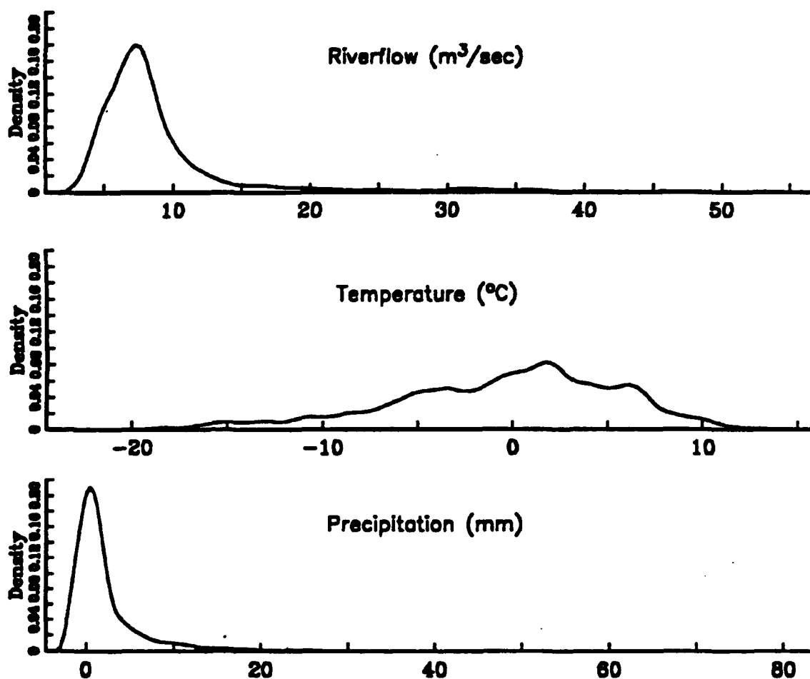
Figure 22. The empirical density functions of the riverflow, temperature and rainfall data for the Vatnsdalsa riverflow system for 1972 to 1974 taken at the Hveravellir meteorological station in Iceland. The y-axis scale (density) of the plots are equal while the x-axis is scaled for each time series and reflects the range of each time series for the years 1972-1974. The empirical density function of the temperature is relatively symmetric. In contrast, the empirical density functions of the riverflow and temperature data are extremely skewed. The skewness in the precipitation data is a result of the heavy but infrequent precipitation that occurs each year, while the skewness in the riverflow data can be attributed to the high riverflow that occurs each spring. This figure should be interpreted with the understanding that the data is clearly seasonal. The
