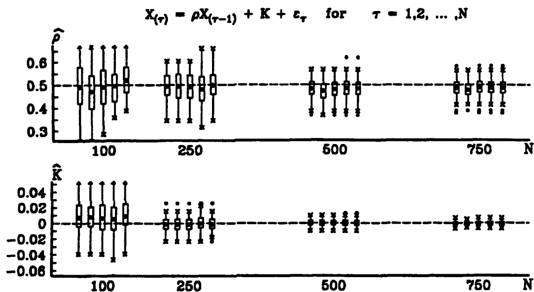
Figure 41. AR(1) MODEL SIMULATION: Boxplots of the estimates from each model selection criterion for \rho = .5, K = 0 when the model selection criterion within MARS correctly identified the data as from an AR(1) model (as reflected in Table 6). For increasing values of N , MARS attempted to identify the AR(1) model (64) from the simulated data using P = 4 lagged predictor variables and M = 8 , the maximum number of subregions allowed in the forward-step MARS procedure, with \sigma_{\varepsilon}^2 = N(0, 1) and a minimum span of MS = .02(N) data points between knots. Each simulation consists of 100 replications. The model selection criterion represented by the boxplots are, from left to right and for each value of N ; GCV^* , AIC , PC , SC and AIC2 . The true value of the model coefficients, \rho = .5 and K = 0 , are identified by the dashed line across each of the boxplots.
