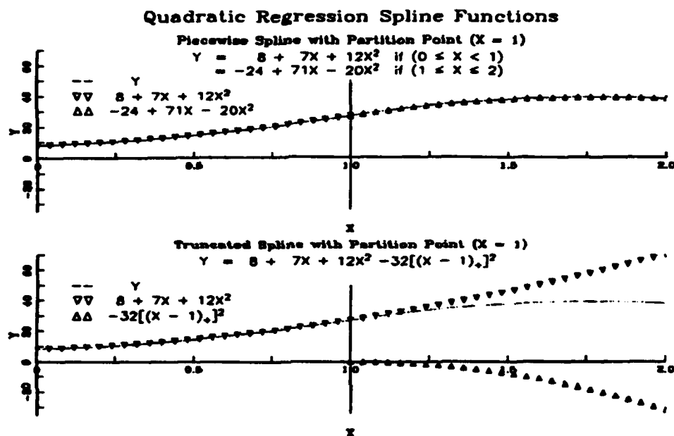
Figure 1. The different forms for a piecewise (16) and truncated (19) spline function using ( q = 2 )-order splines over the region D = [0, 2] with a single partition point at x = 1 . In the top plot, the line y is defined by two different disjoint 2nd-order polynomial functions; one 2nd-order polynomial function for the region [0, 1) shown as \nabla \nabla \dots and one 2nd-order polynomial function for the region [1, 2] shown as \Delta \Delta \dots . In the bottom plot the line y in the region from [0, 1) is again defined by the single 2nd-order polynomial function 8 + 7x + 12x^2 shown as \nabla \nabla \dots . However, in the subregion from [1, 2] , the line y is defined as the sum of two overlapping 2nd order polynomial functions; 8 + 7x + 12x^2 that continues from the first subregion and the truncated 2nd-order polynomial function -32[(x-1)_+]^2 shown as \Delta \Delta \dots .
